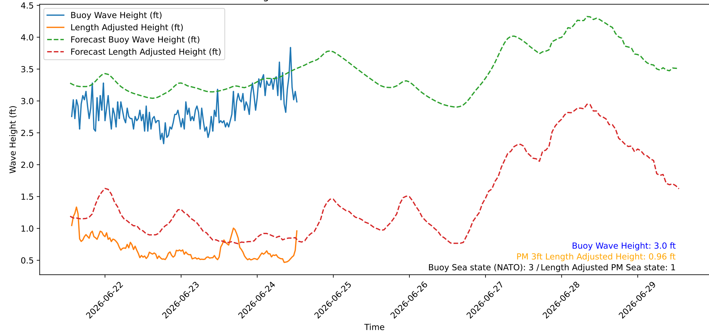
Wave Heights over Time for Red Beach at 2026-06-24 13:10:46
