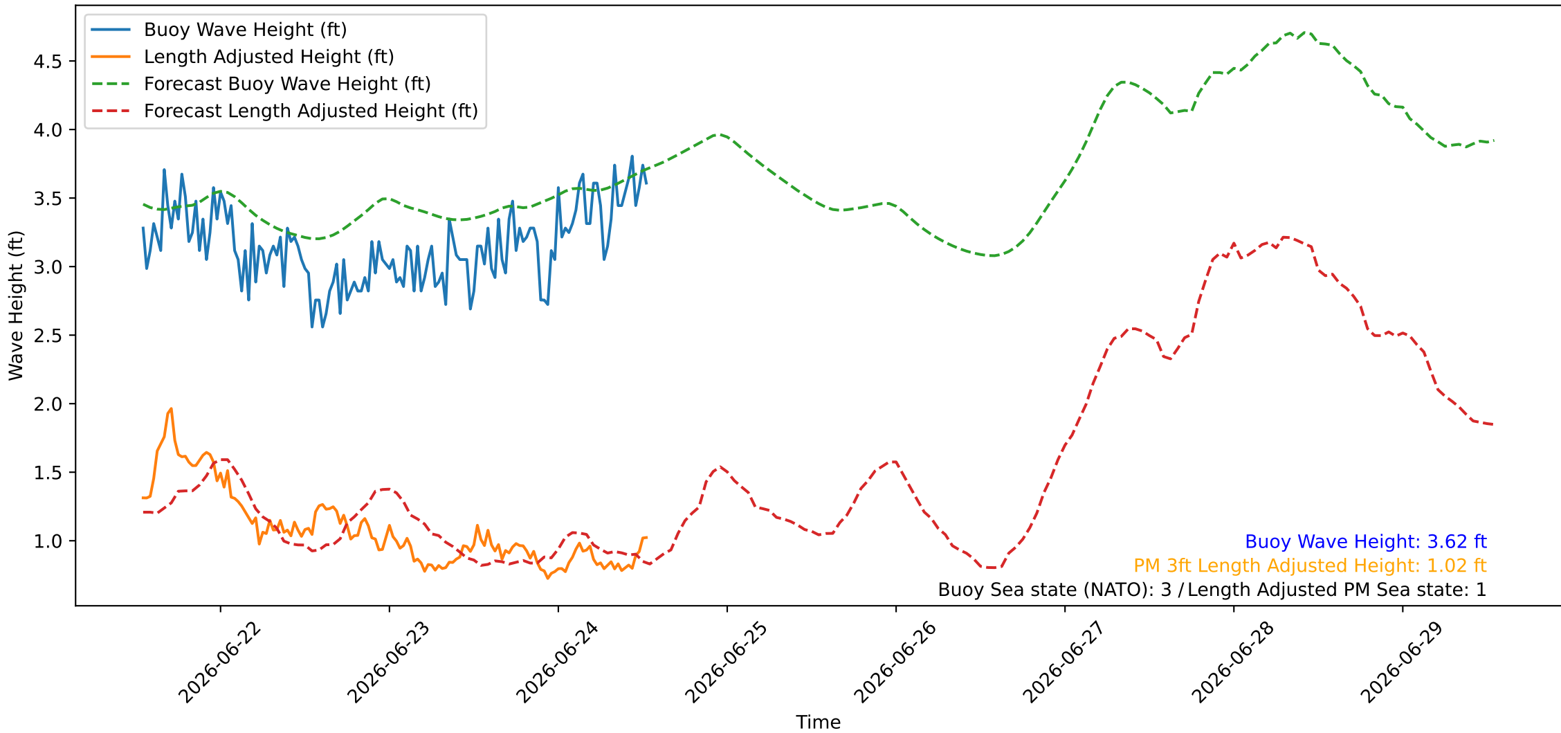
Wave Heights over Time for Oceanside Harbor at 2026-06-24 13:10:26
