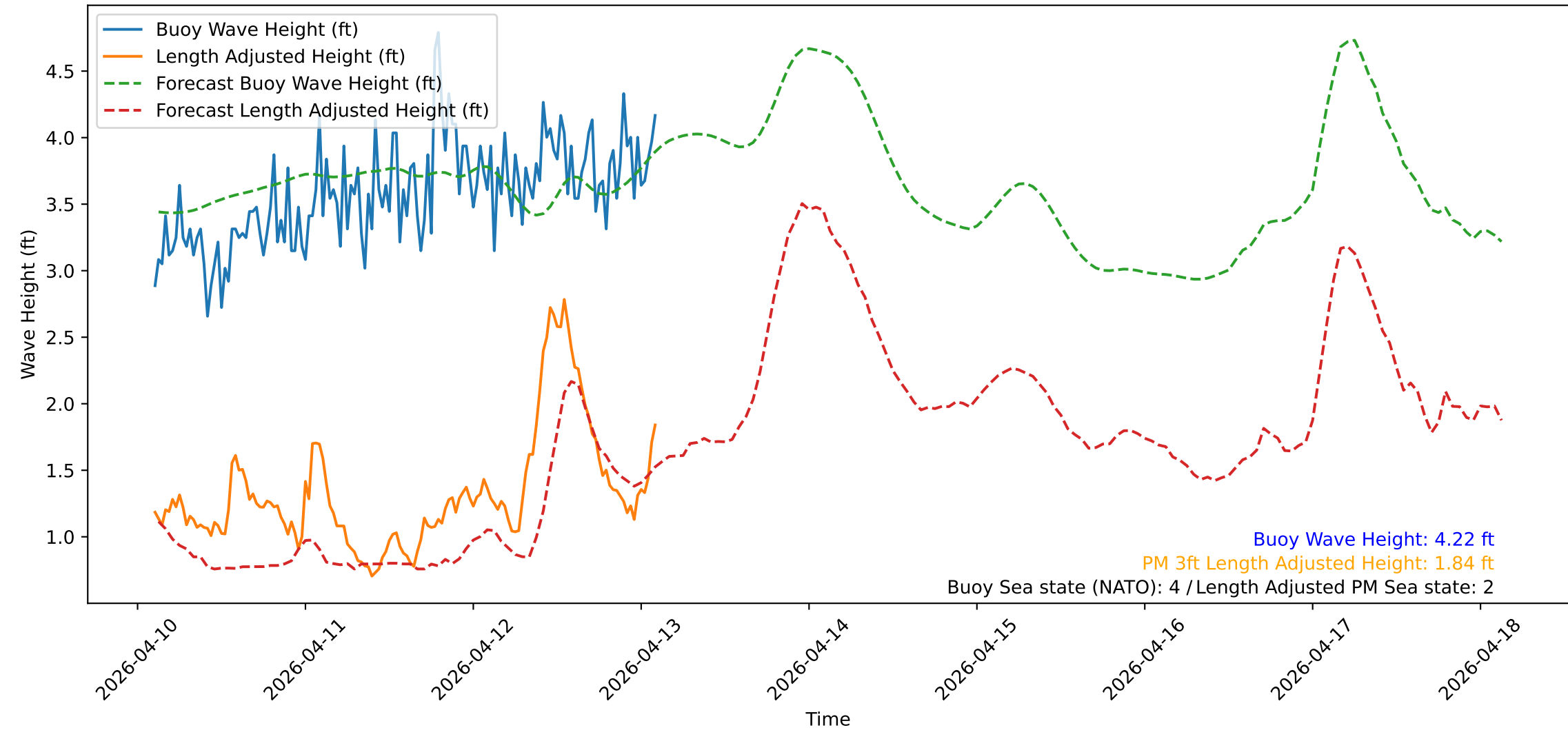
Wave Heights over Time for Oceanside Harbor at 2026-04-13 02:40:31
