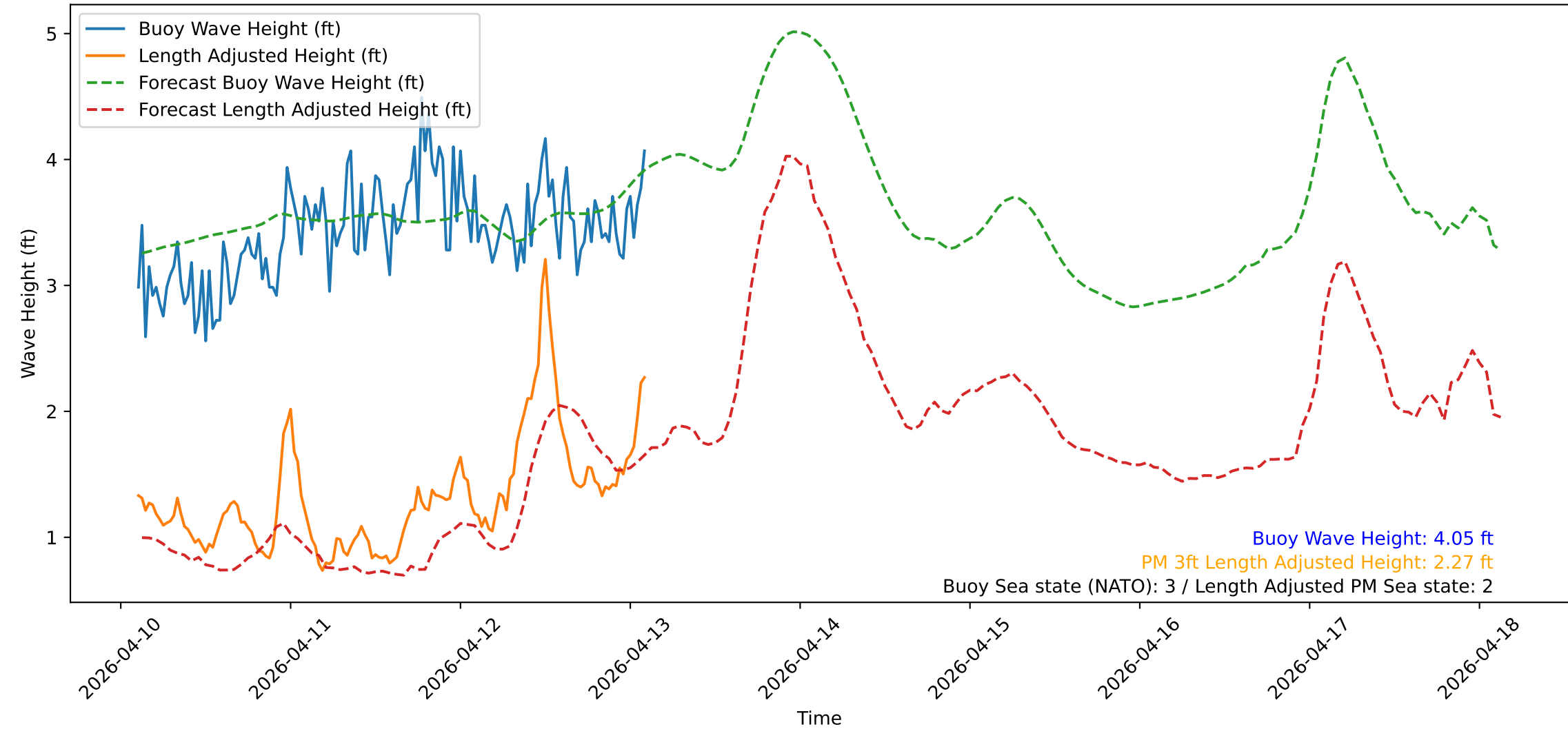
Wave Heights over Time for Green Beach at 2026-04-13 02:41:12
