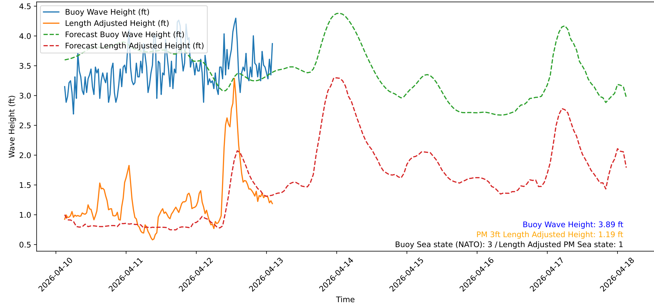
Wave Heights over Time for Red Beach at 2026-04-13 02:40:50
