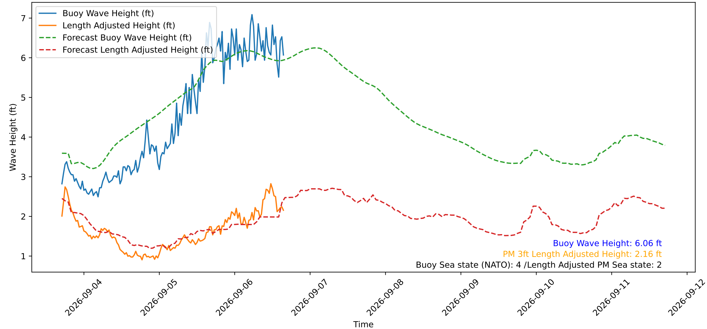
Wave Heights over Time for Green Beach at 2026-09-06 16:31:12
