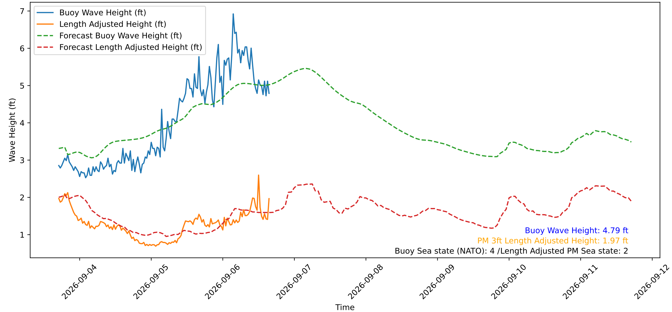
Wave Heights over Time for Red Beach at 2026-09-06 16:30:50
