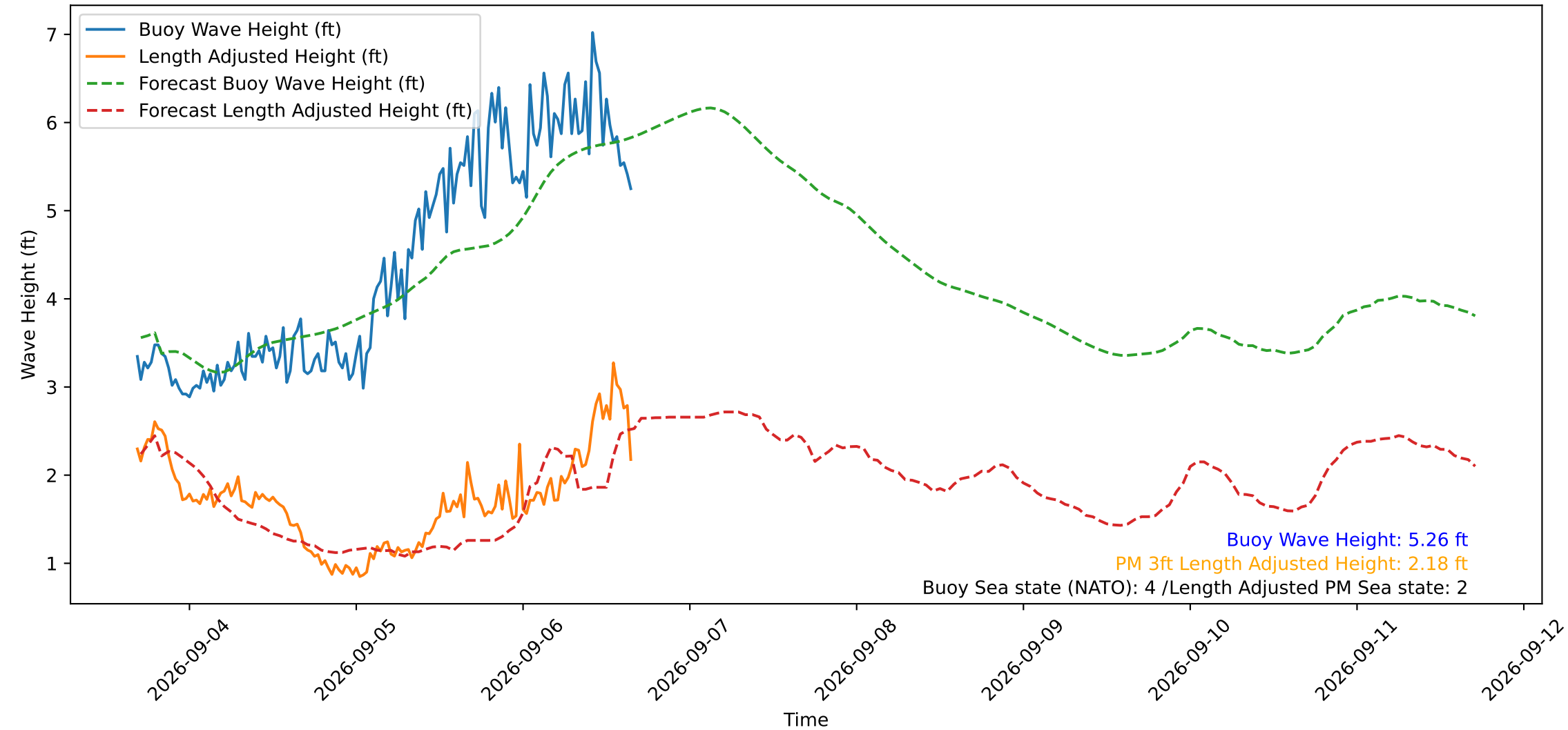
Wave Heights over Time for Oceanside Harbor at 2026-09-06 16:30:30
