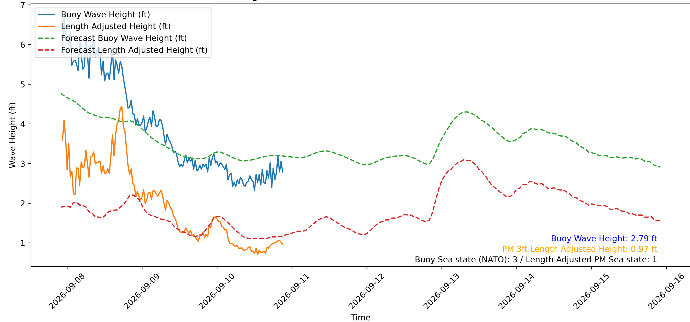
Wave Heights over Time for Red Beach at 2026-09-10 22:00:50
