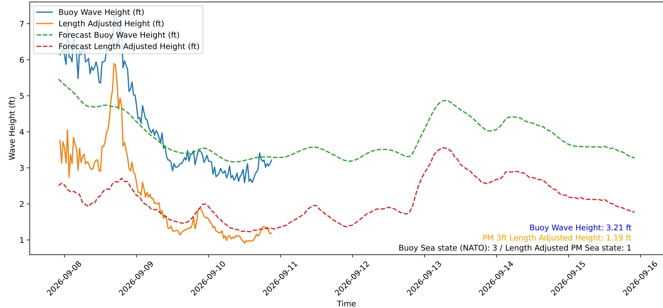
Wave Heights over Time for Green Beach at 2026-09-10 22:01:12
