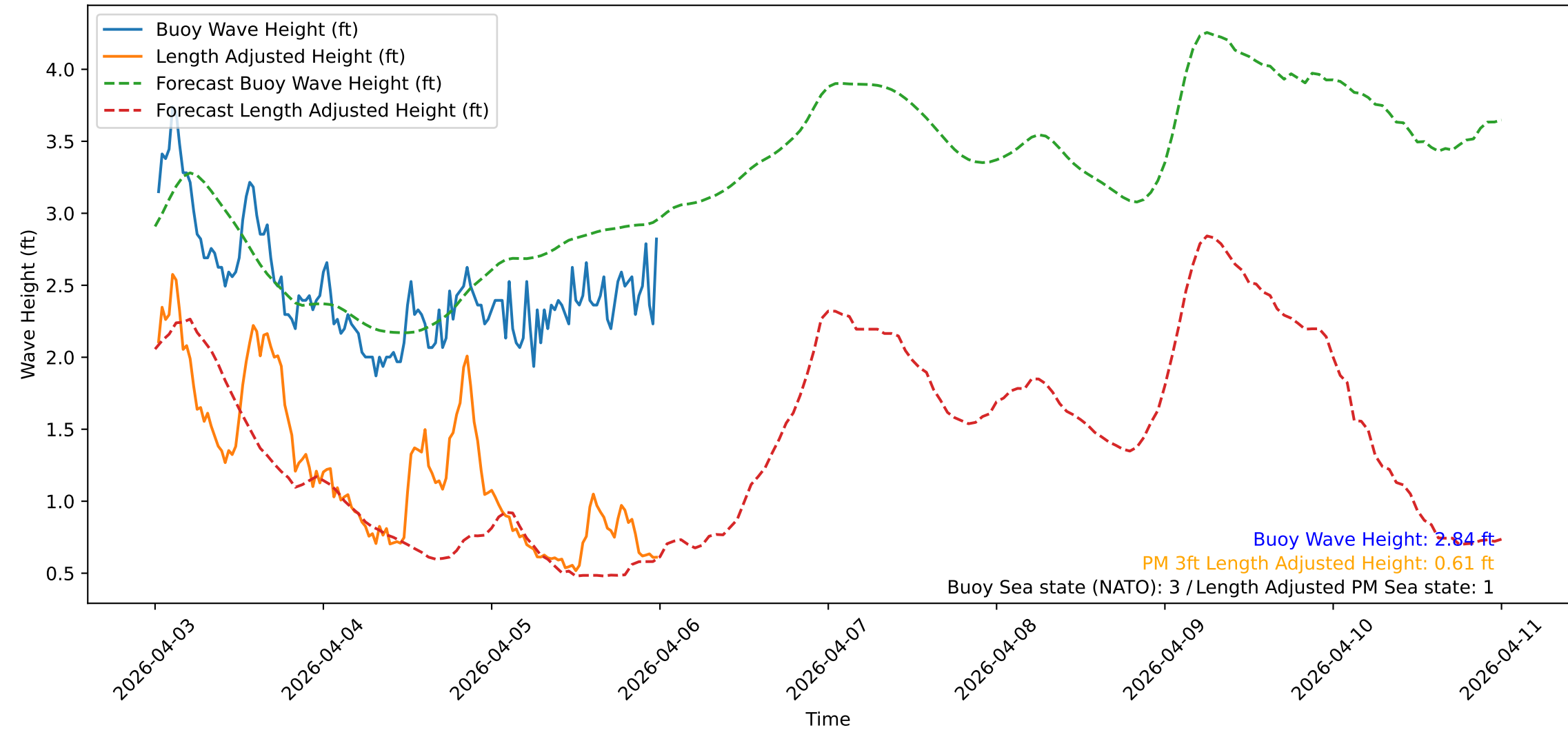
Wave Heights over Time for Red Beach at 2026-04-06 00:10:47
