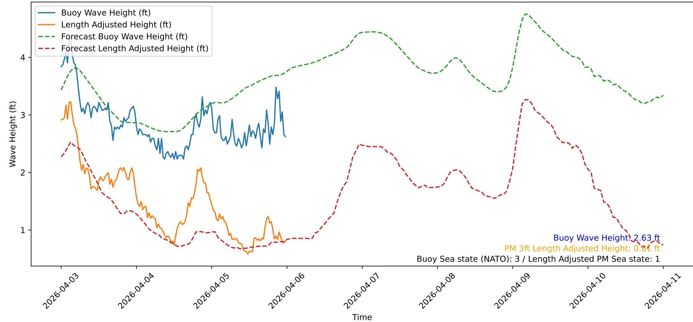
Wave Heights over Time for Green Beach at 2026-04-06 00:11:09
