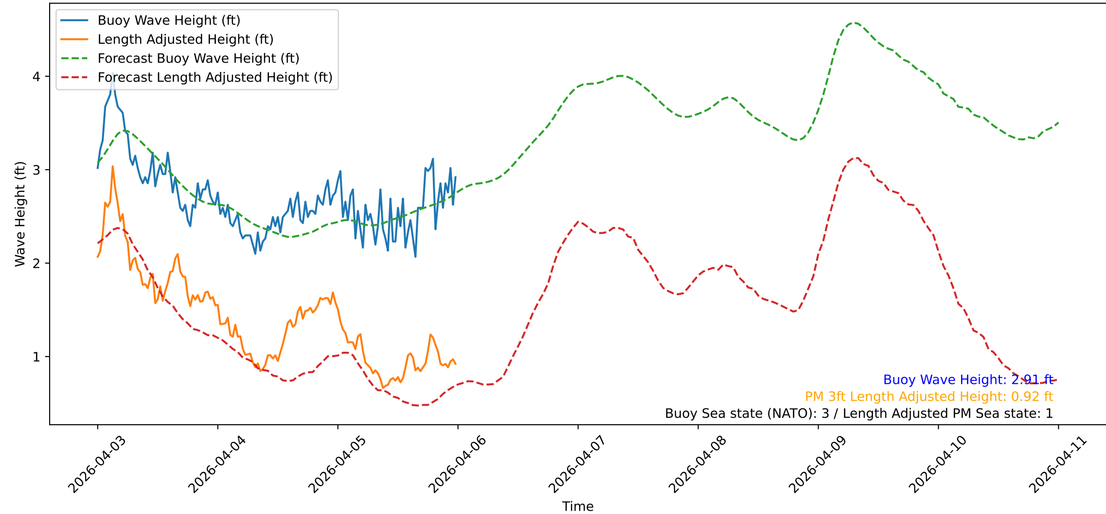
Wave Heights over Time for Oceanside Harbor at 2026-04-06 00:10:31
