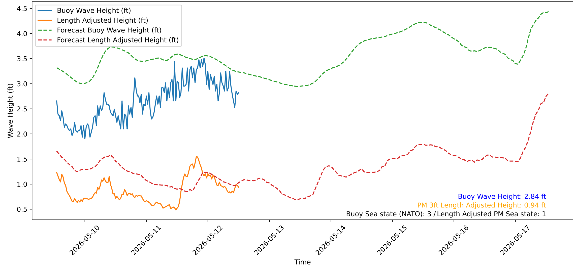
Wave Heights over Time for Green Beach at 2026-05-12 12:51:14
