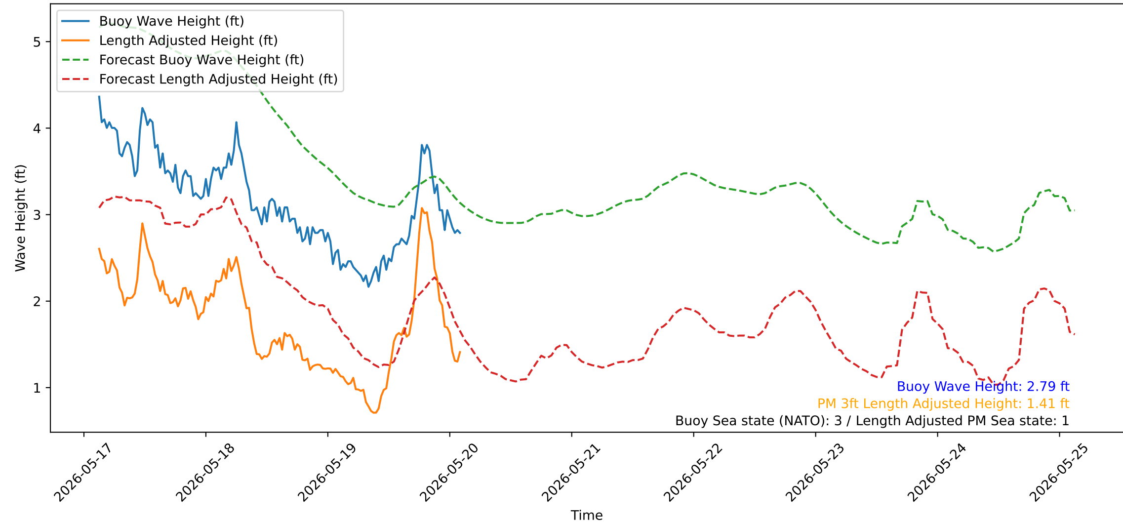
Wave Heights over Time for Green Beach at 2026-05-20 02:51:15
