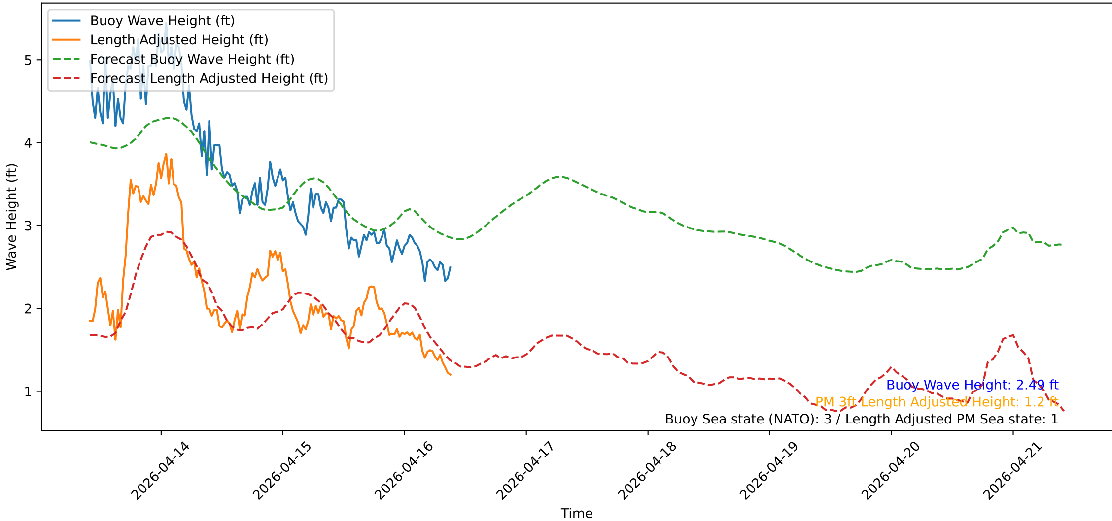
Wave Heights over Time for Oceanside Harbor at 2026-04-16 09:50:31
