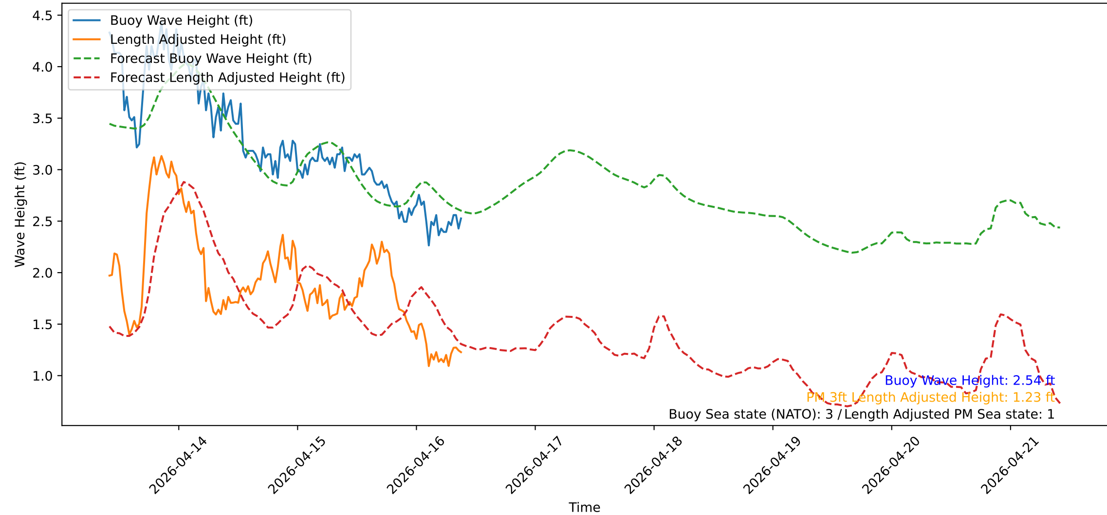
Wave Heights over Time for Red Beach at 2026-04-16 09:50:52
