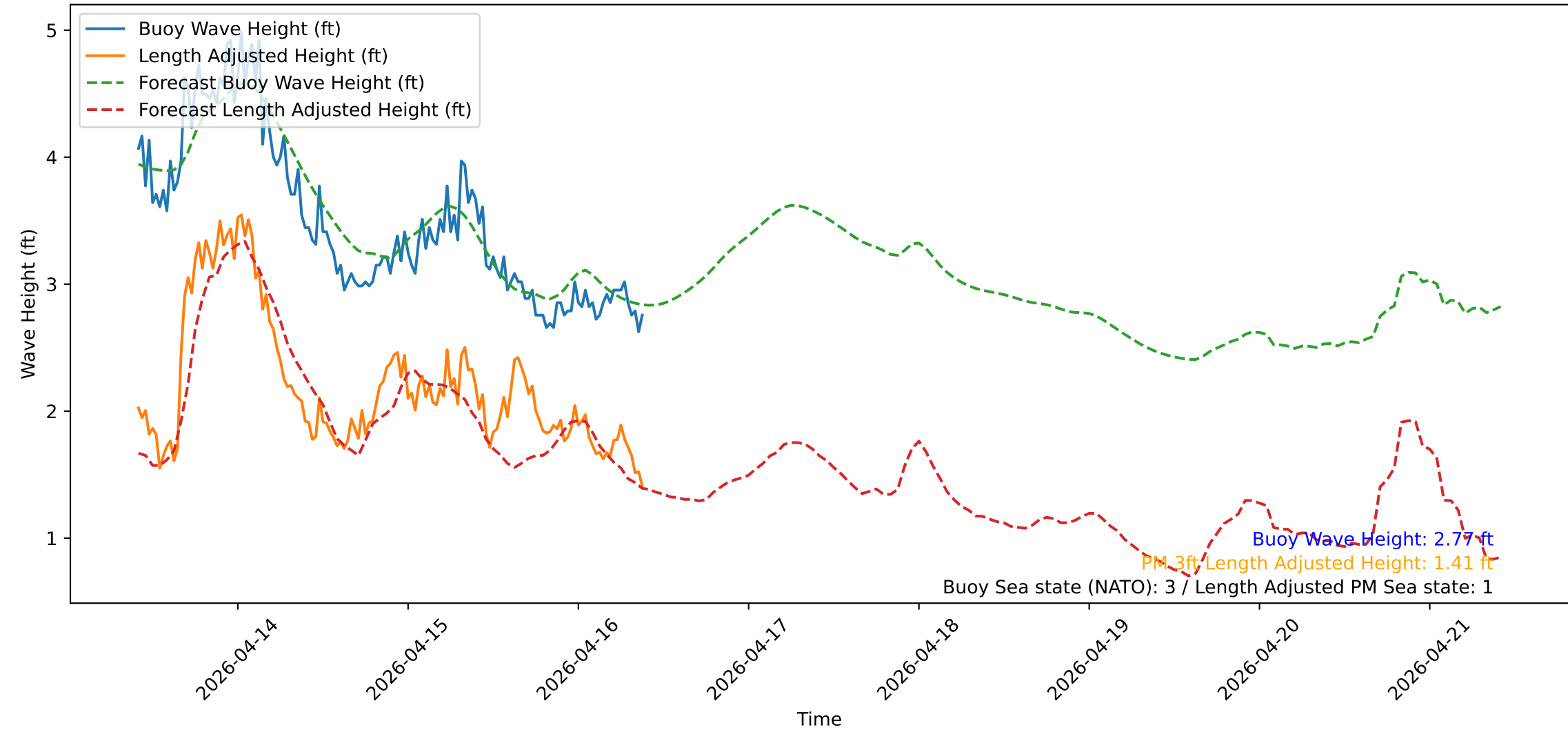
Wave Heights over Time for Green Beach at 2026-04-16 09:51:14
