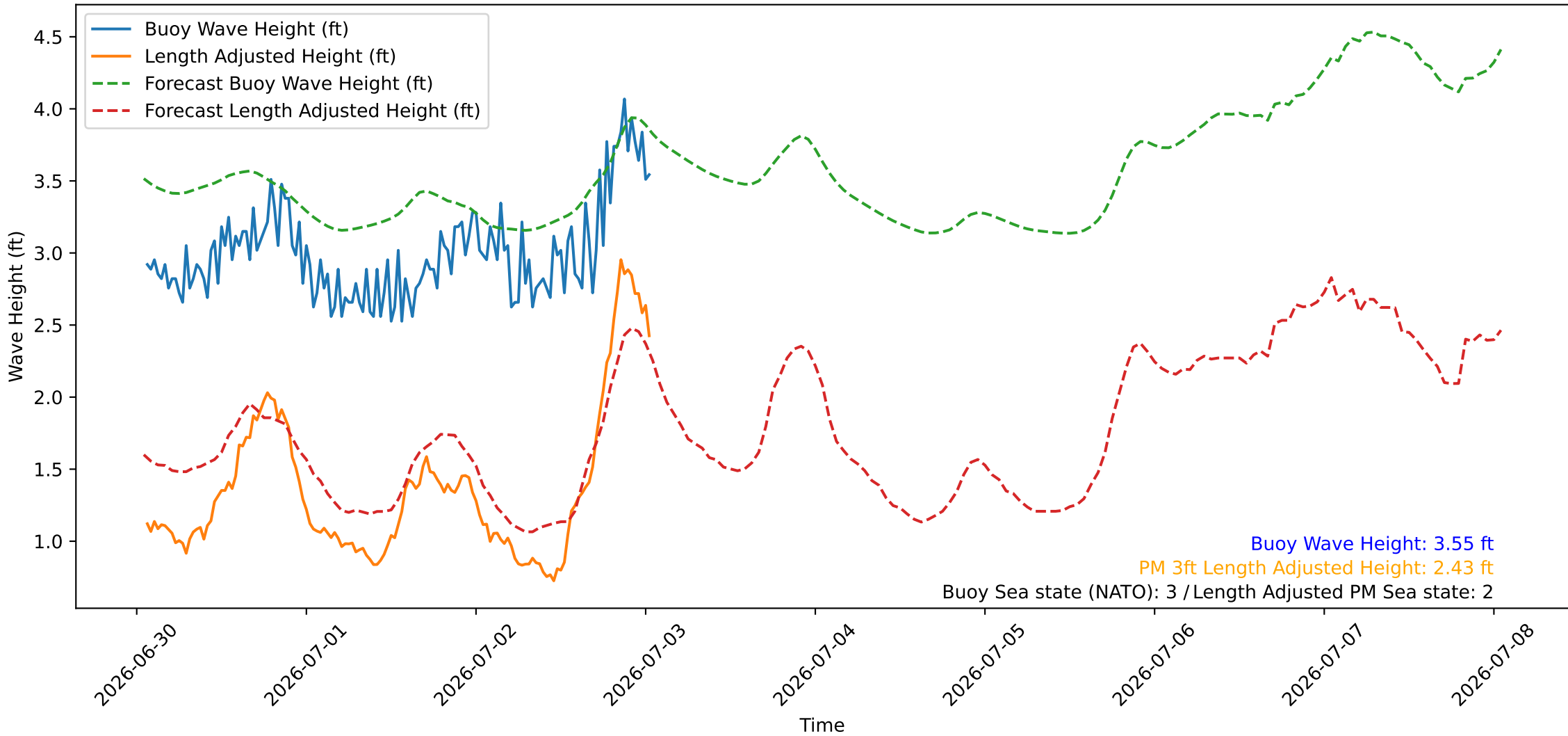
Wave Heights over Time for Green Beach at 2026-07-03 01:21:20
