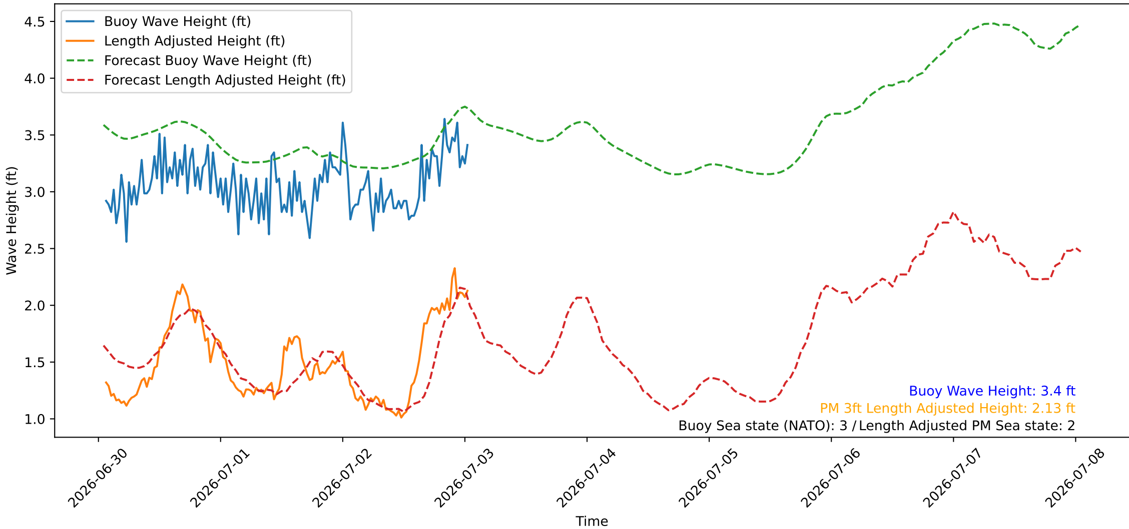
Wave Heights over Time for Oceanside Harbor at 2026-07-03 01:20:26
