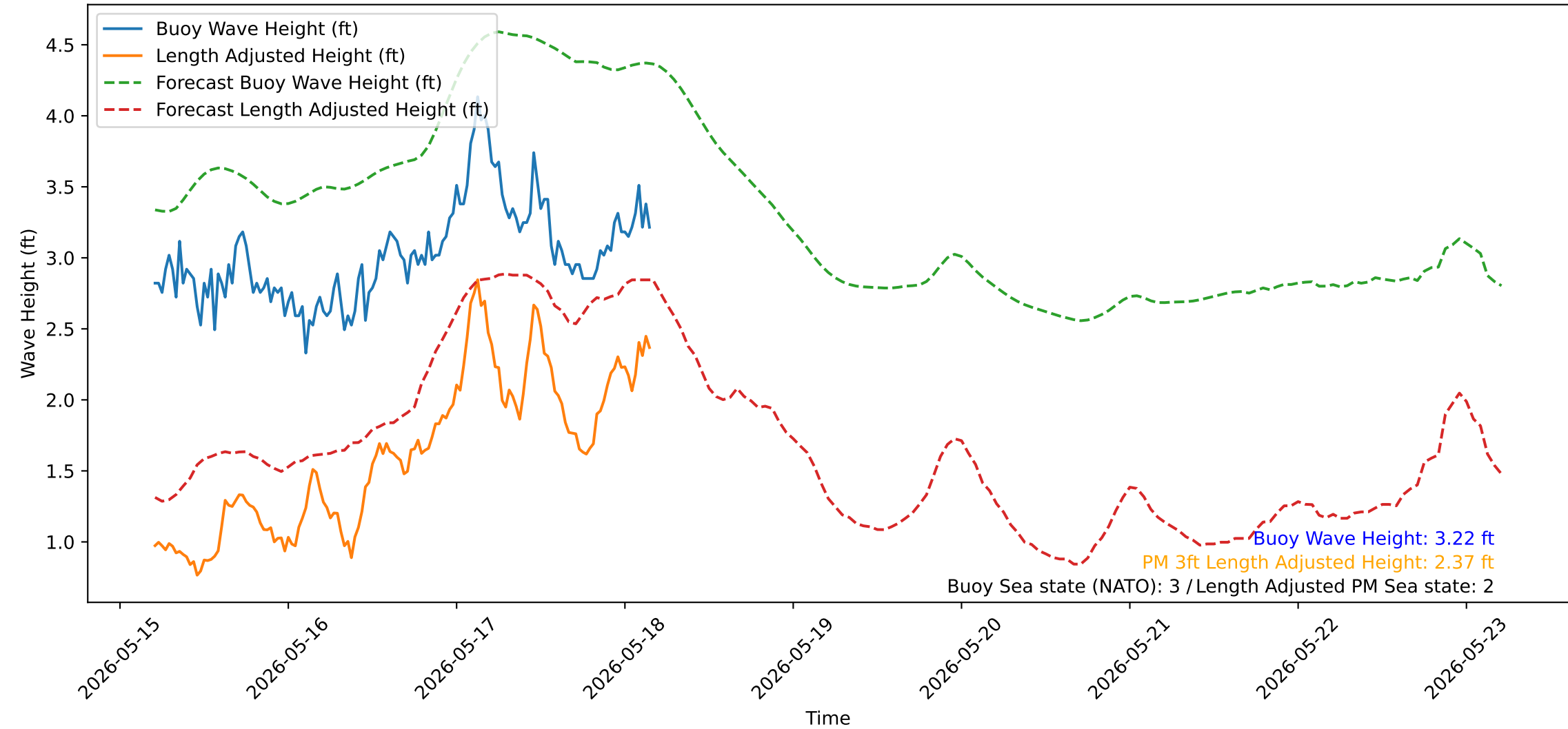
Wave Heights over Time for Red Beach at 2026-05-18 04:30:51
