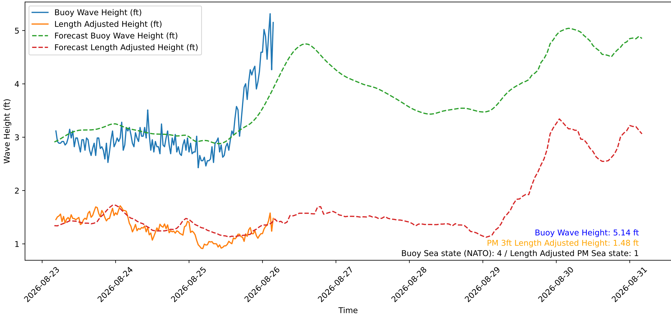
Wave Heights over Time for Oceanside Harbor at 2026-08-26 04:20:31
