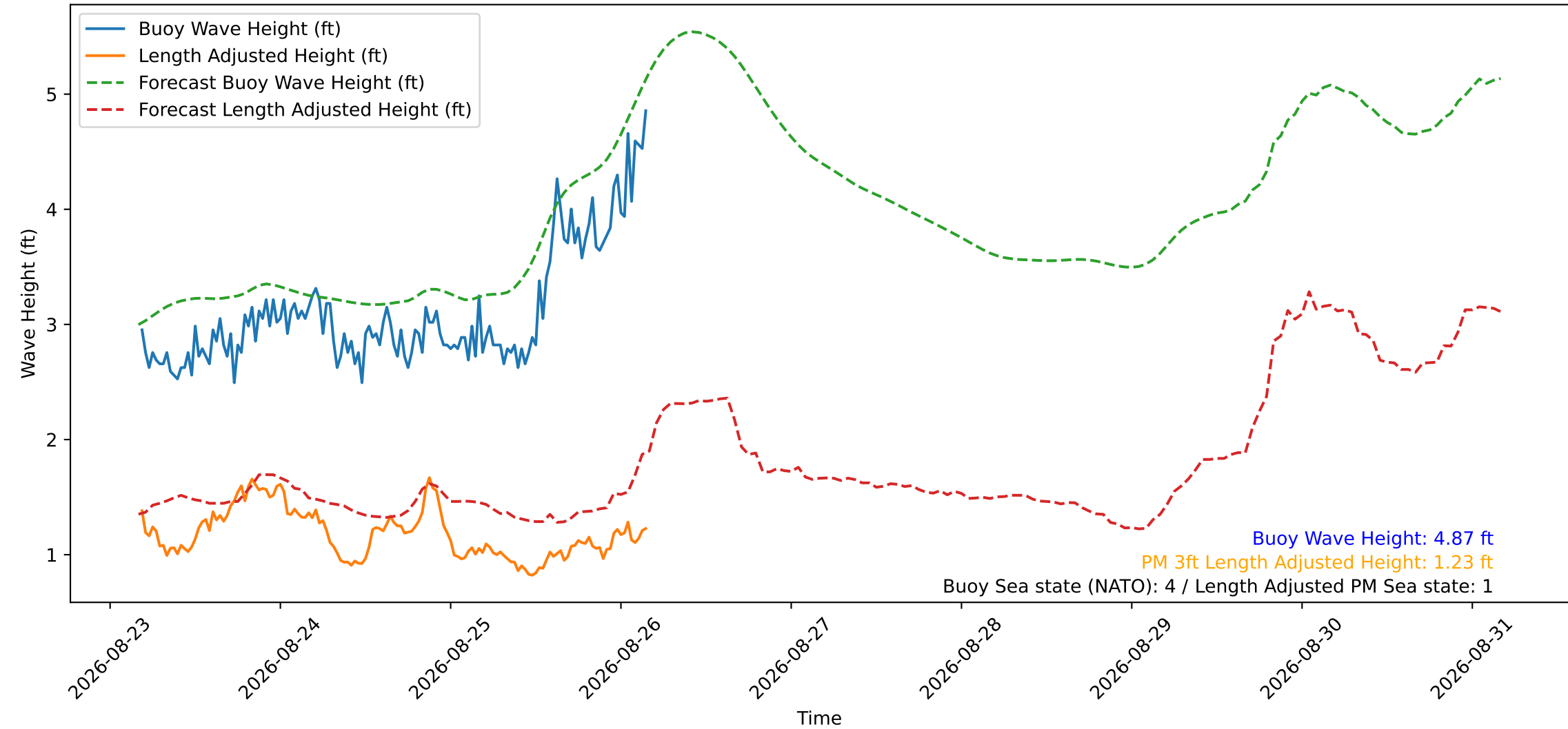
Wave Heights over Time for Green Beach at 2026-08-26 04:21:16
