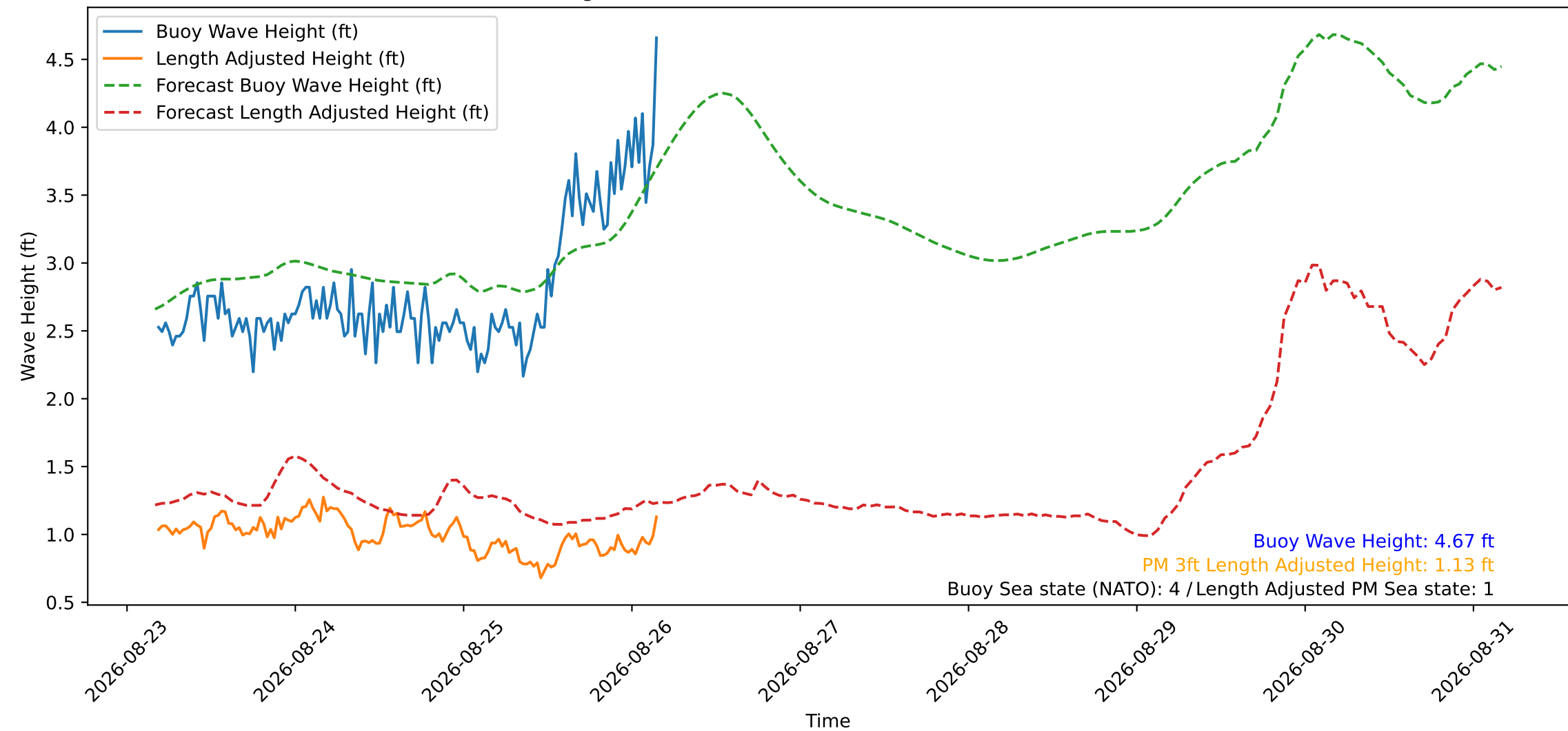
Wave Heights over Time for Red Beach at 2026-08-26 04:20:52
