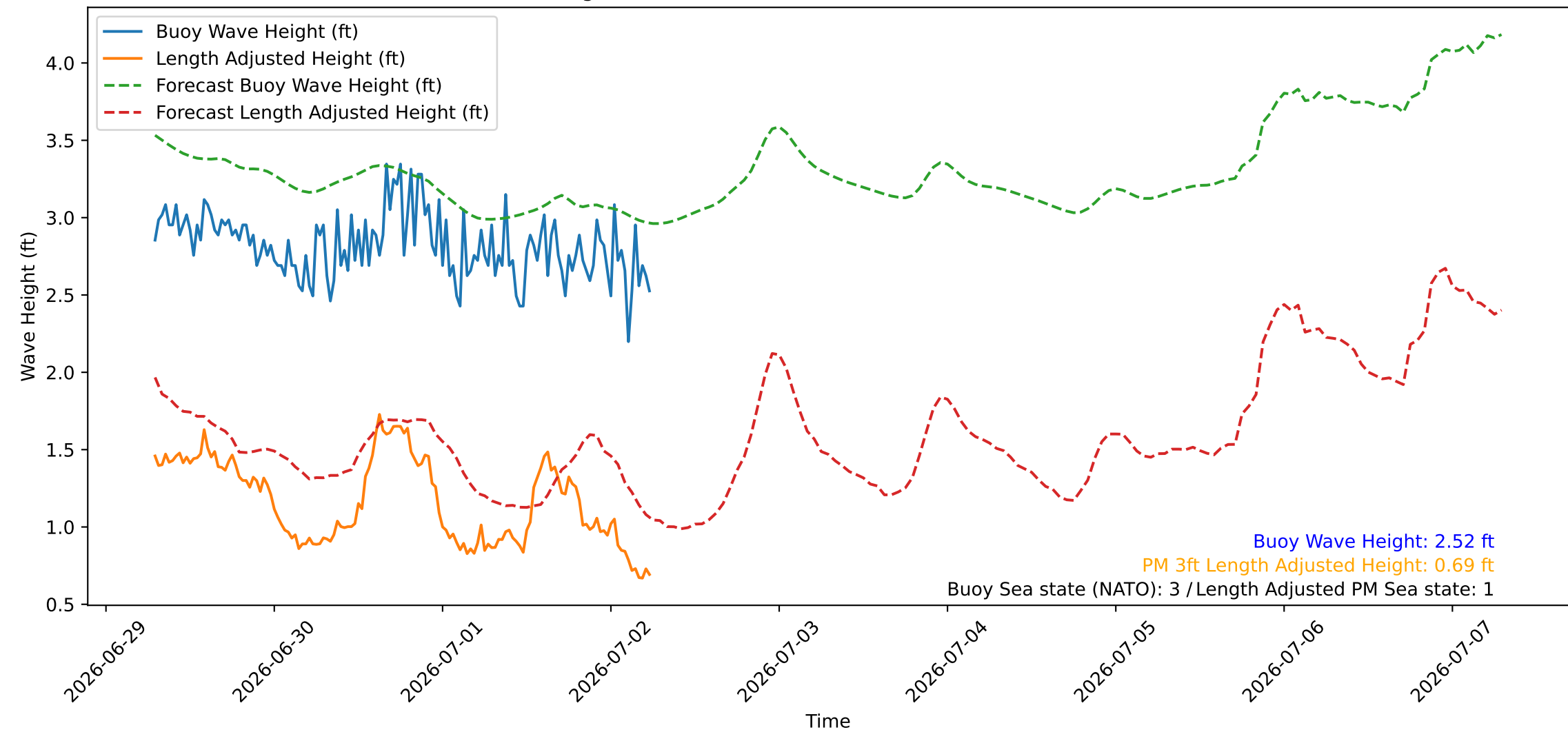
Wave Heights over Time for Red Beach at 2026-07-02 06:30:46
