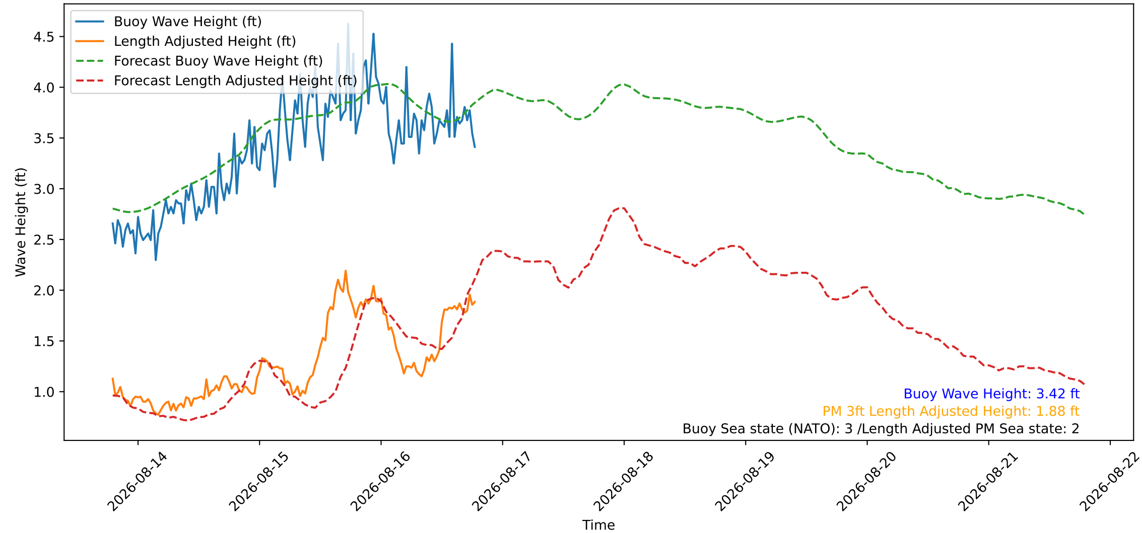
Wave Heights over Time for Oceanside Harbor at 2026-08-16 19:10:26
