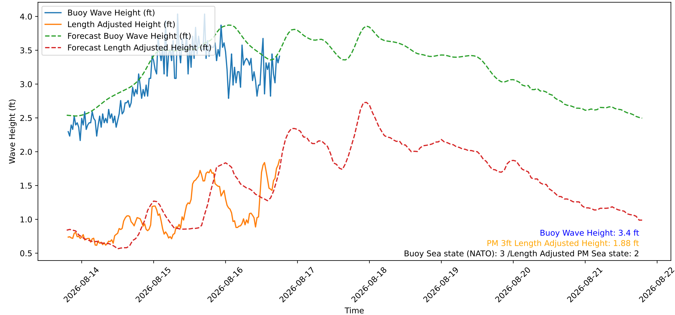
Wave Heights over Time for Red Beach at 2026-08-16 19:10:46
