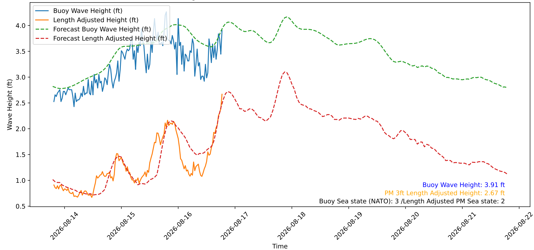
Wave Heights over Time for Green Beach at 2026-08-16 19:11:08
