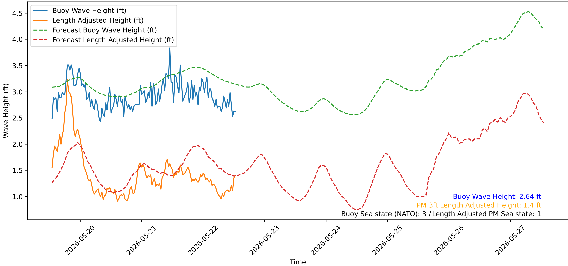
Wave Heights over Time for Oceanside Harbor at 2026-05-22 13:10:32
