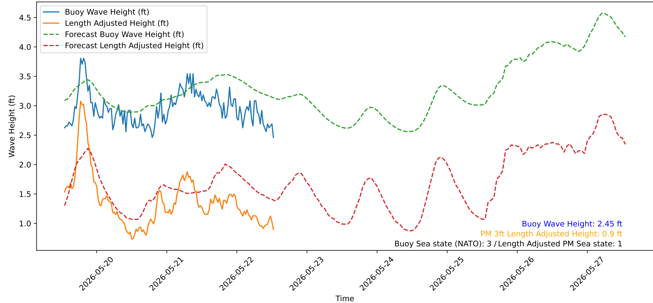
Wave Heights over Time for Green Beach at 2026-05-22 13:11:14
