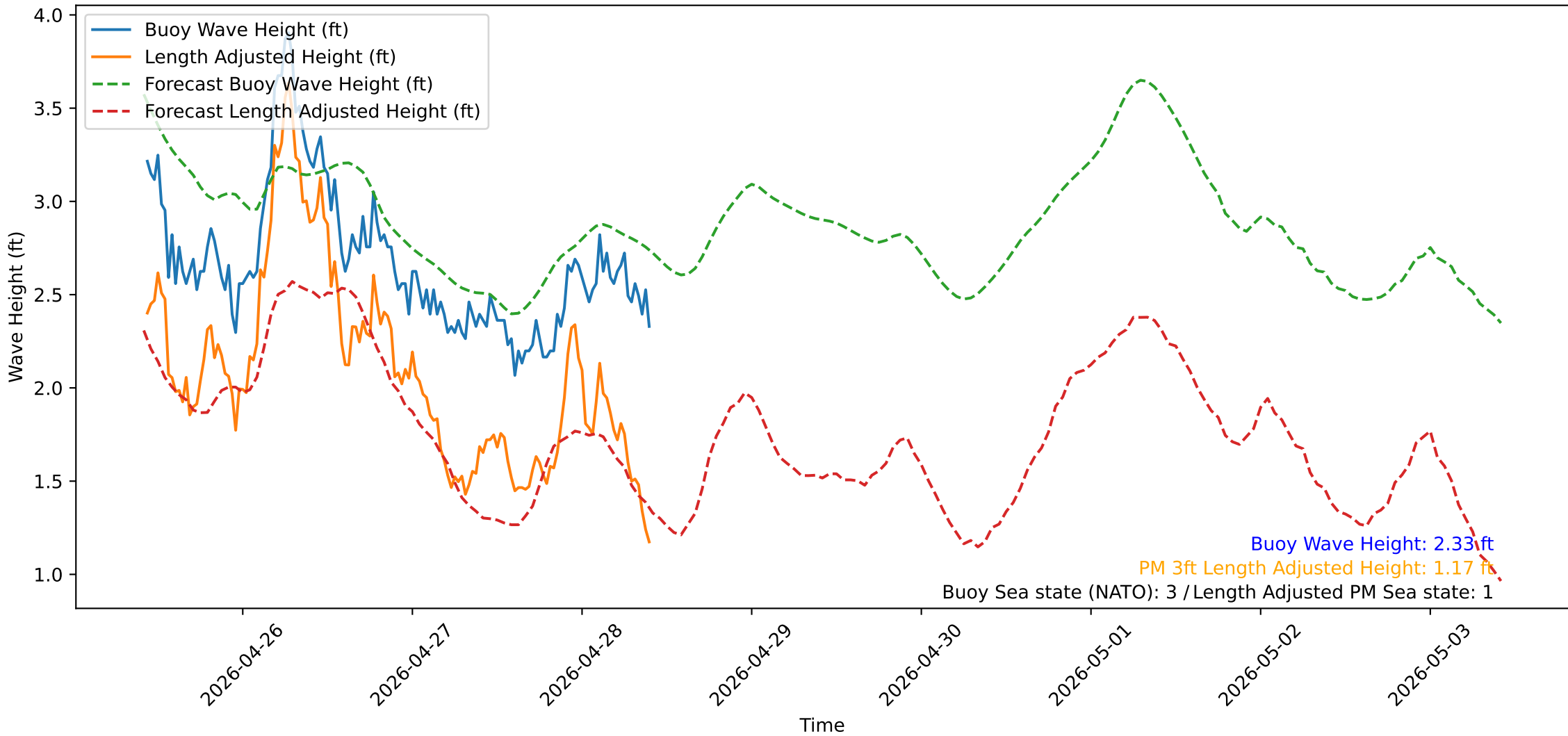
Wave Heights over Time for Oceanside Harbor at 2026-04-28 10:20:31
