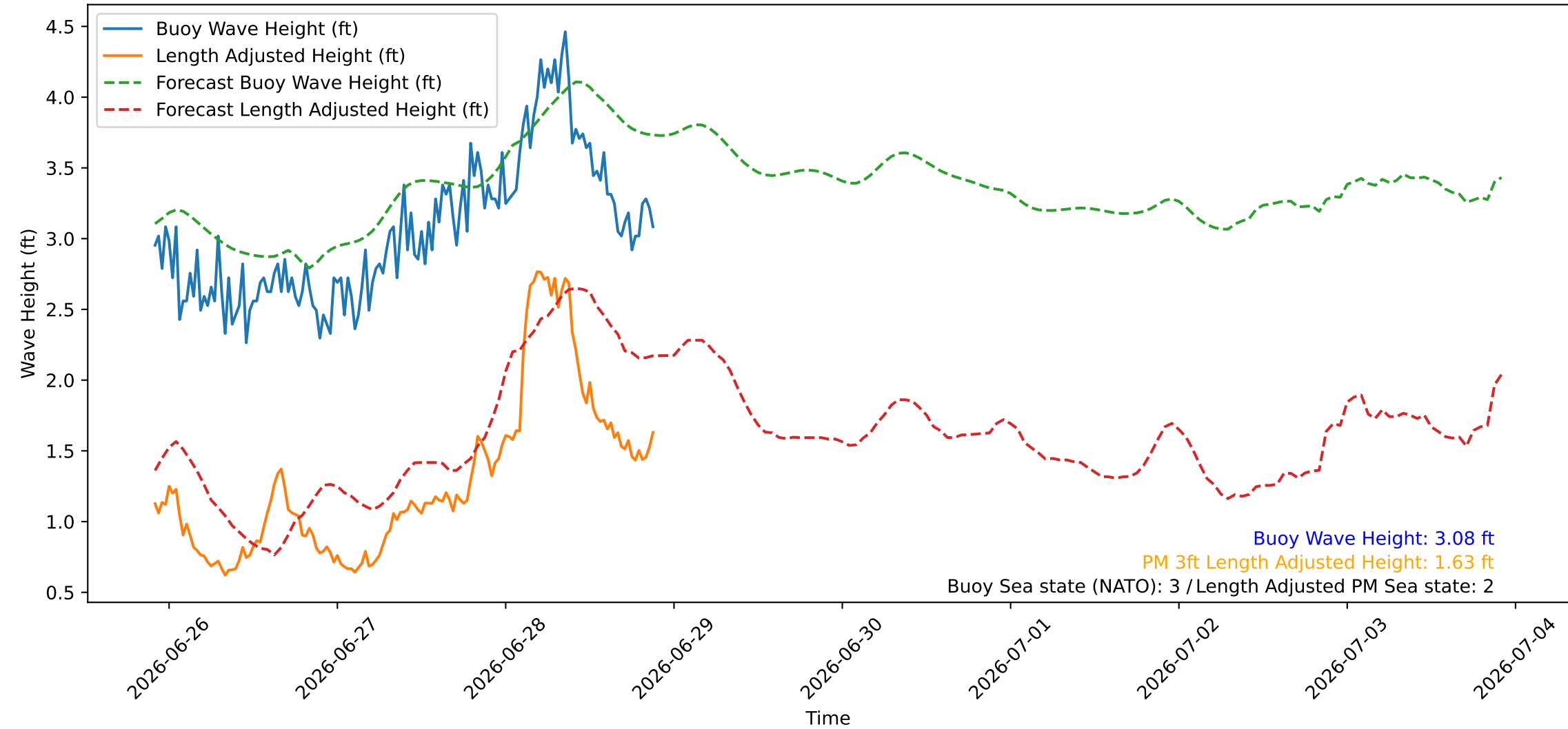
Wave Heights over Time for Red Beach at 2026-06-28 21:40:45
