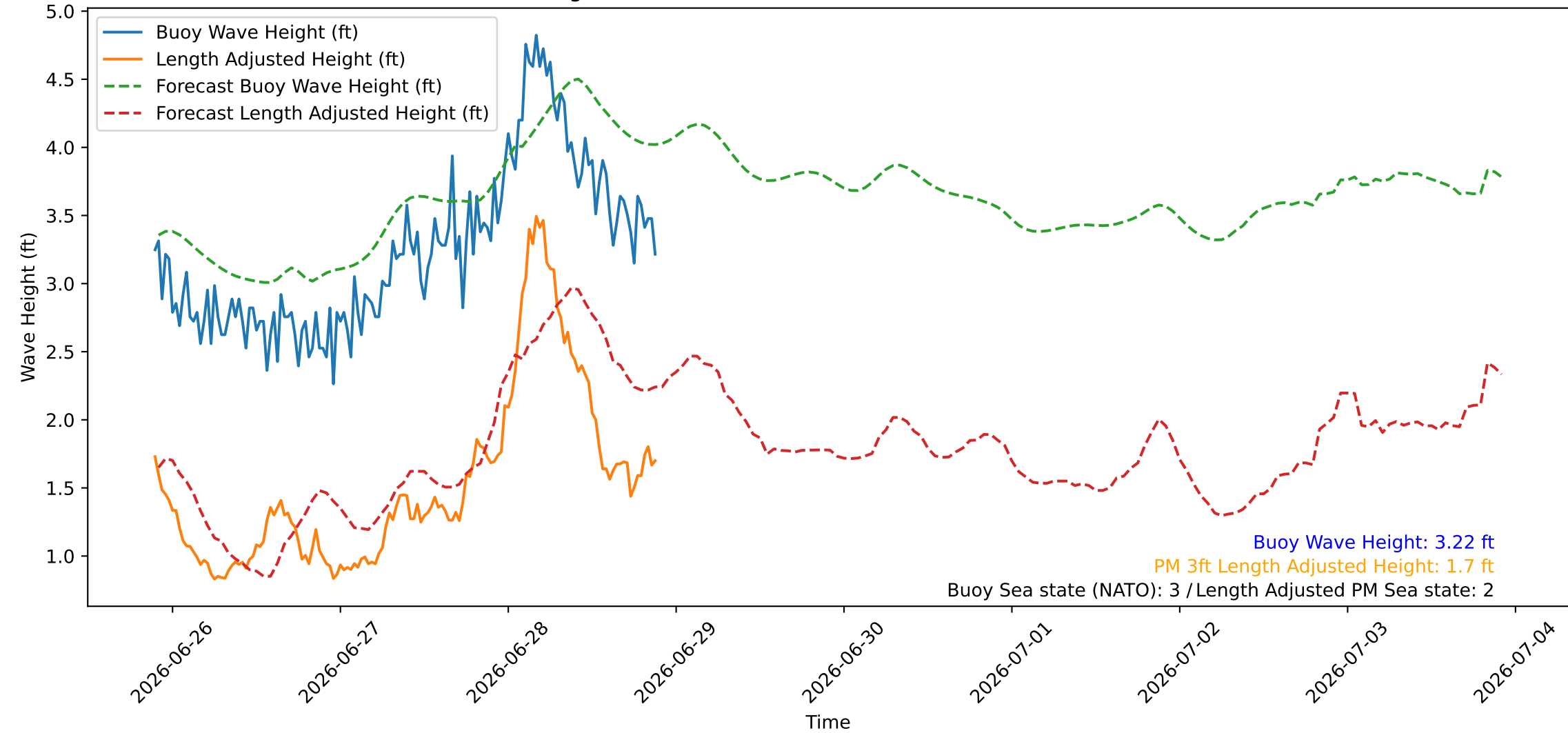
Wave Heights over Time for Green Beach at 2026-06-28 21:41:07
