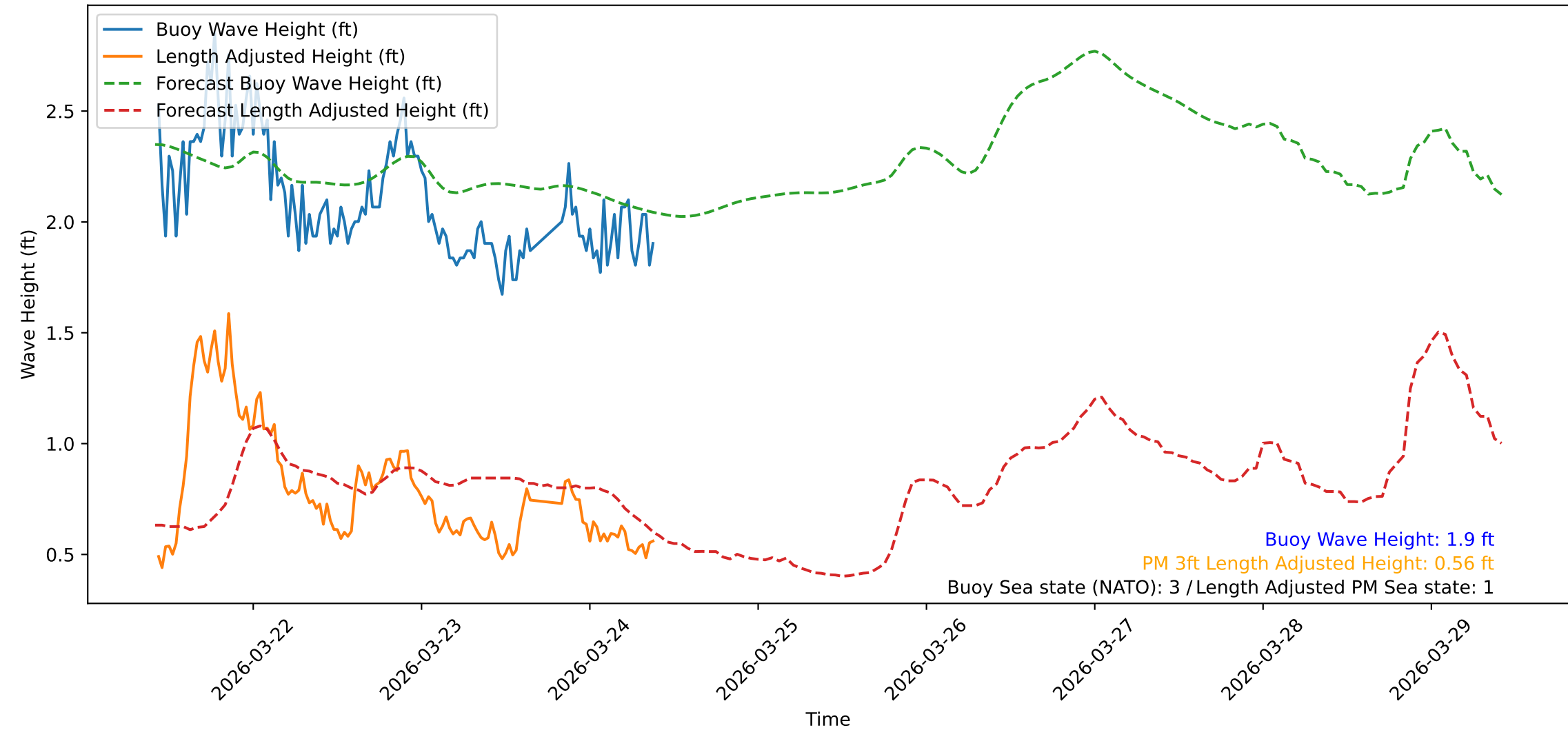
Wave Heights over Time for Red Beach at 2026-03-24 10:20:47
