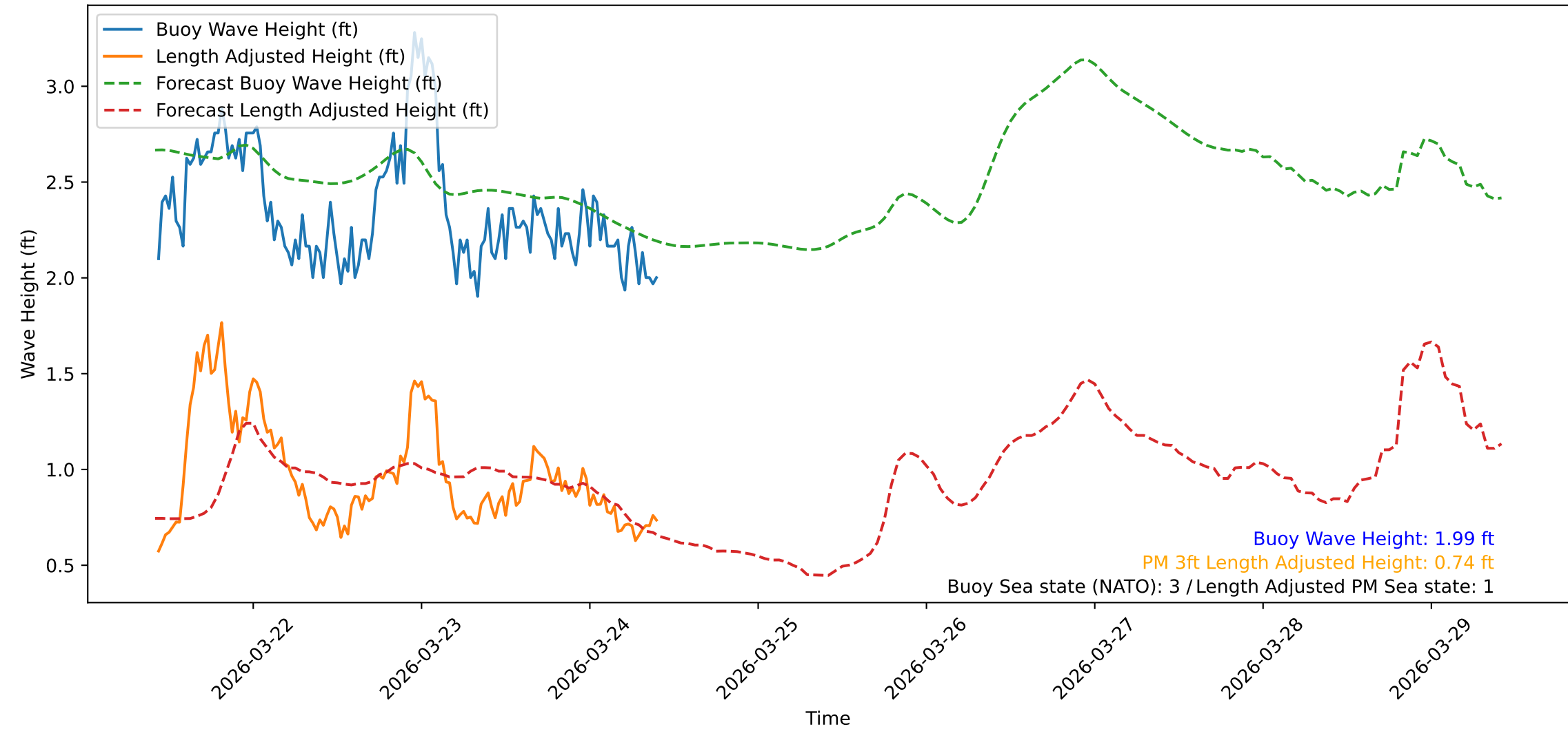
Wave Heights over Time for Green Beach at 2026-03-24 10:21:09
