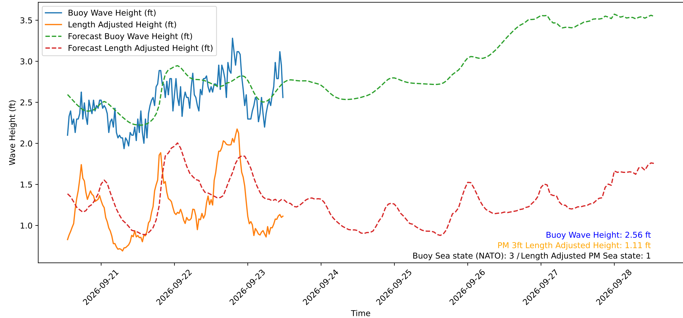
Wave Heights over Time for Red Beach at 2026-09-23 12:30:49
