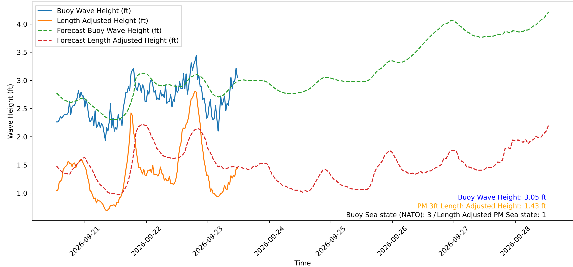
Wave Heights over Time for Green Beach at 2026-09-23 12:31:11
