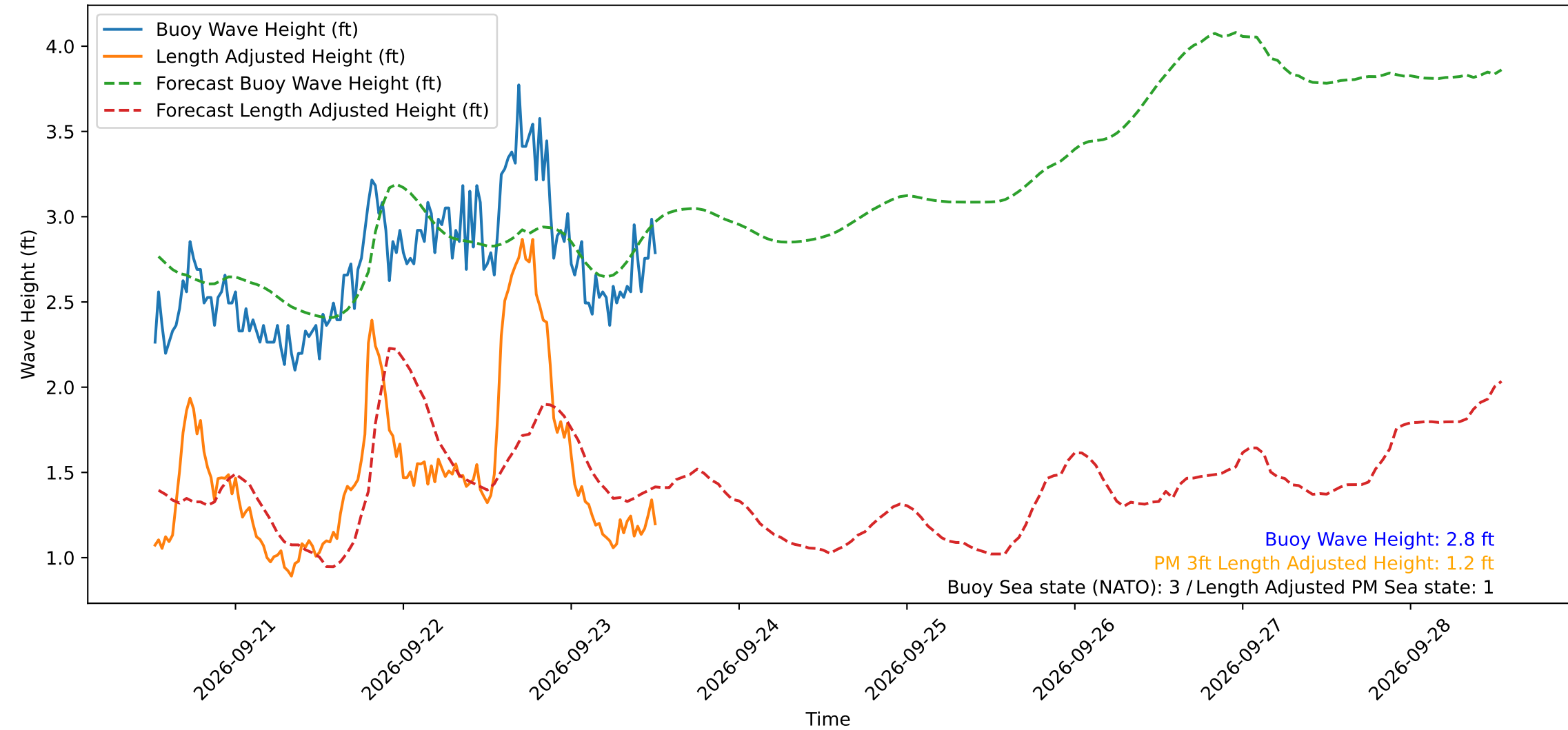
Wave Heights over Time for Oceanside Harbor at 2026-09-23 12:30:30
