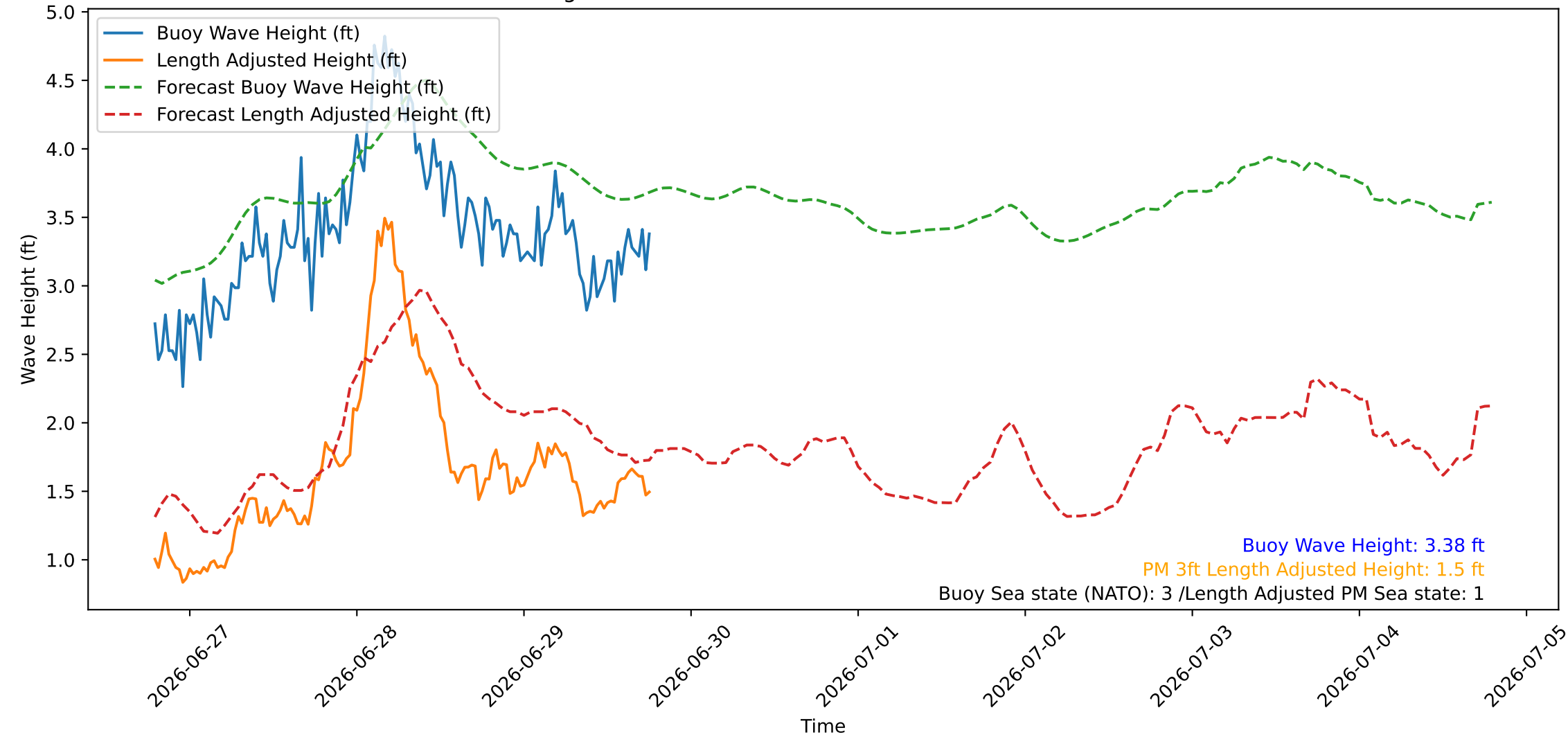
Wave Heights over Time for Green Beach at 2026-06-29 19:01:06
