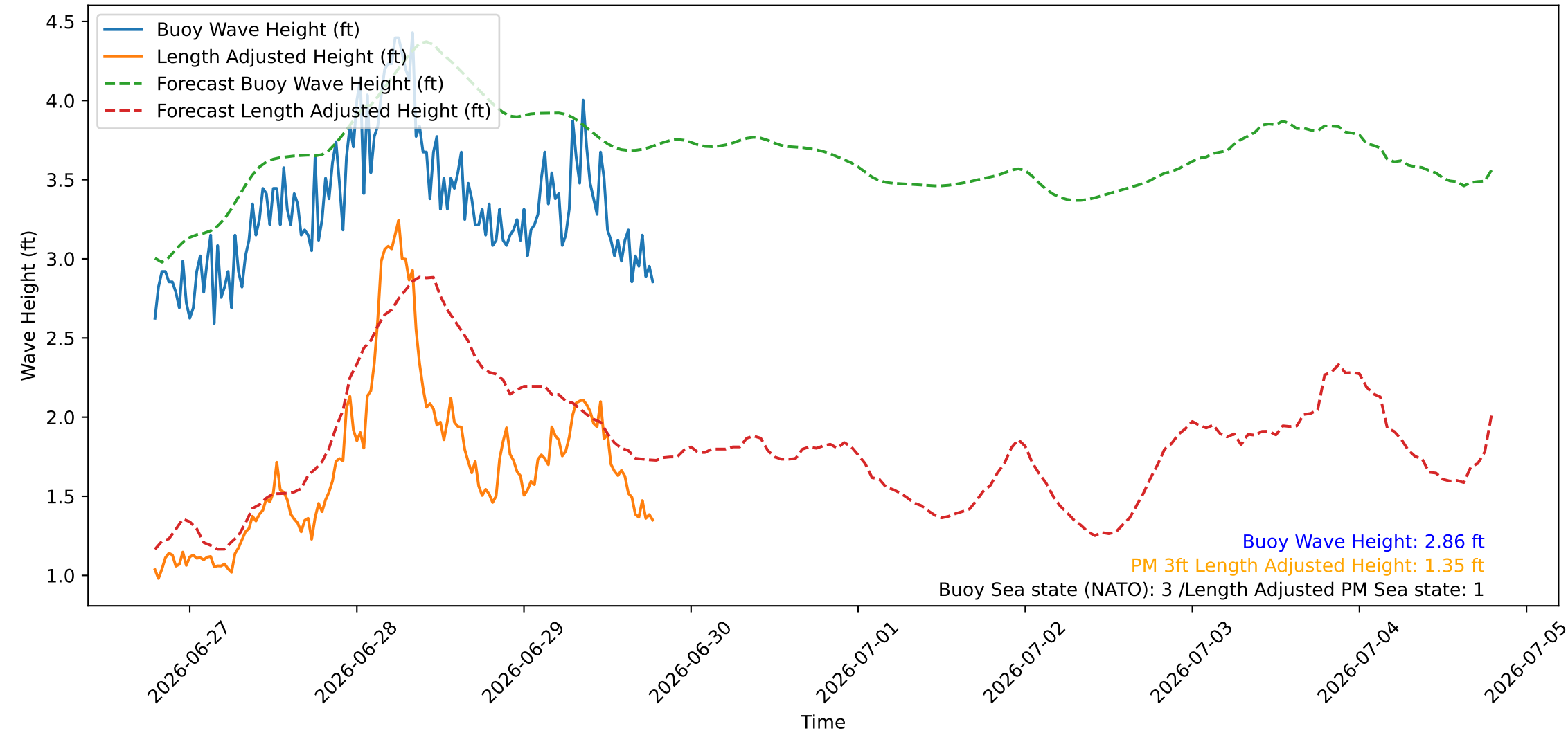
Wave Heights over Time for Oceanside Harbor at 2026-06-29 19:00:26
