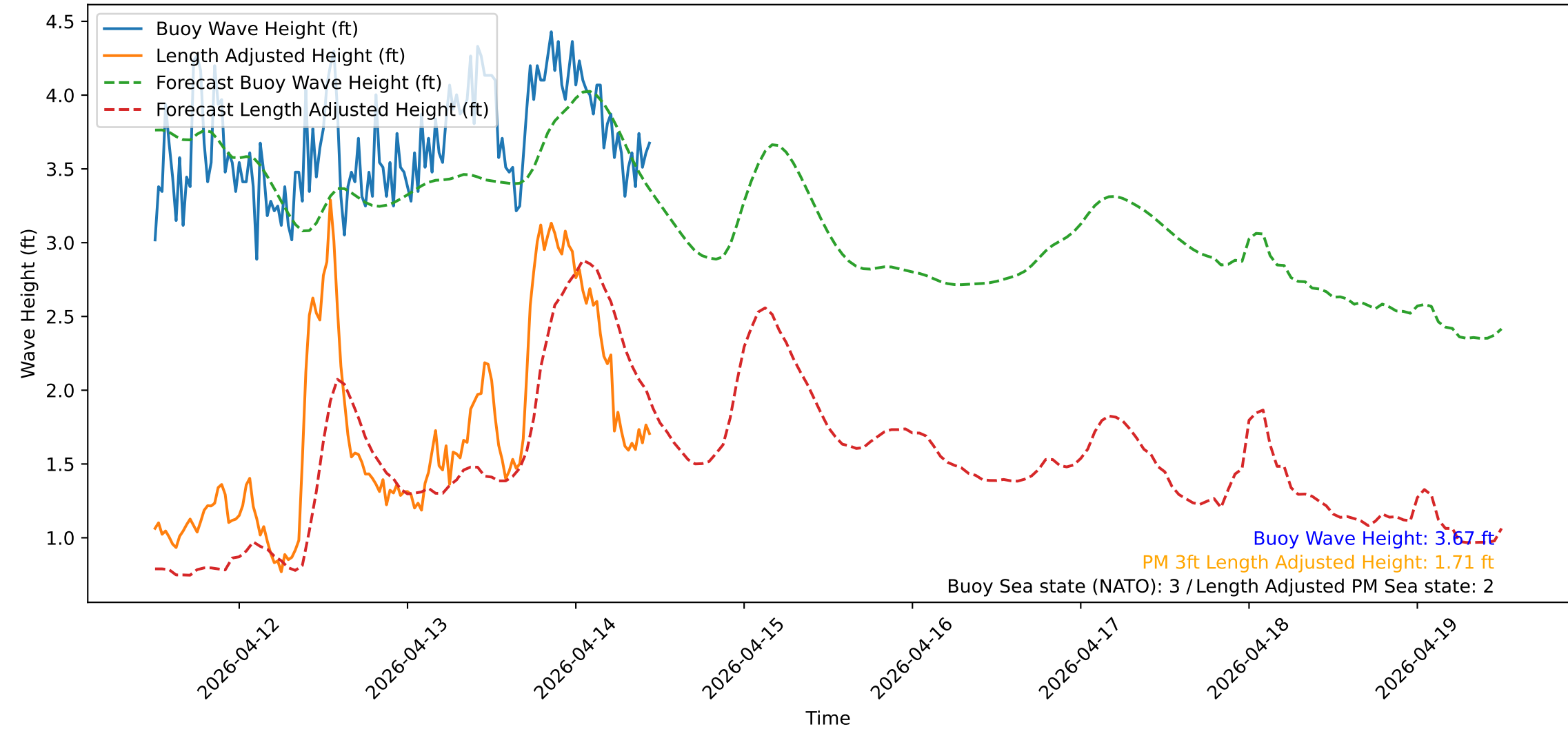
Wave Heights over Time for Red Beach at 2026-04-14 11:30:50
