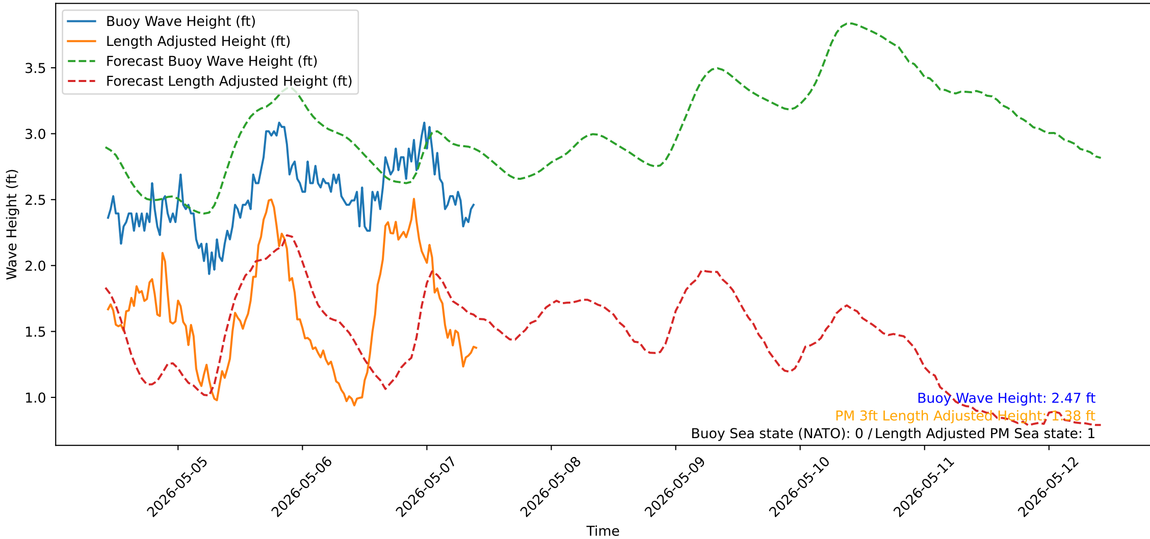
Wave Heights over Time for Red Beach at 2026-05-07 10:10:50
