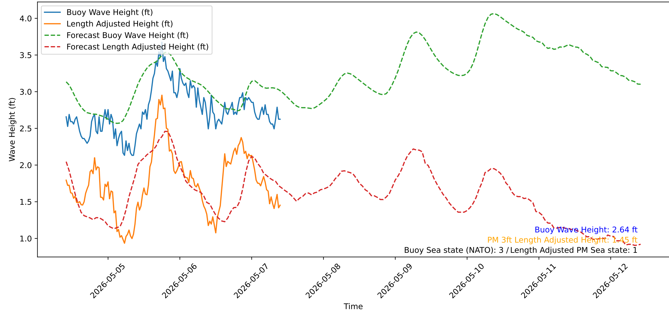
Wave Heights over Time for Green Beach at 2026-05-07 10:11:13
