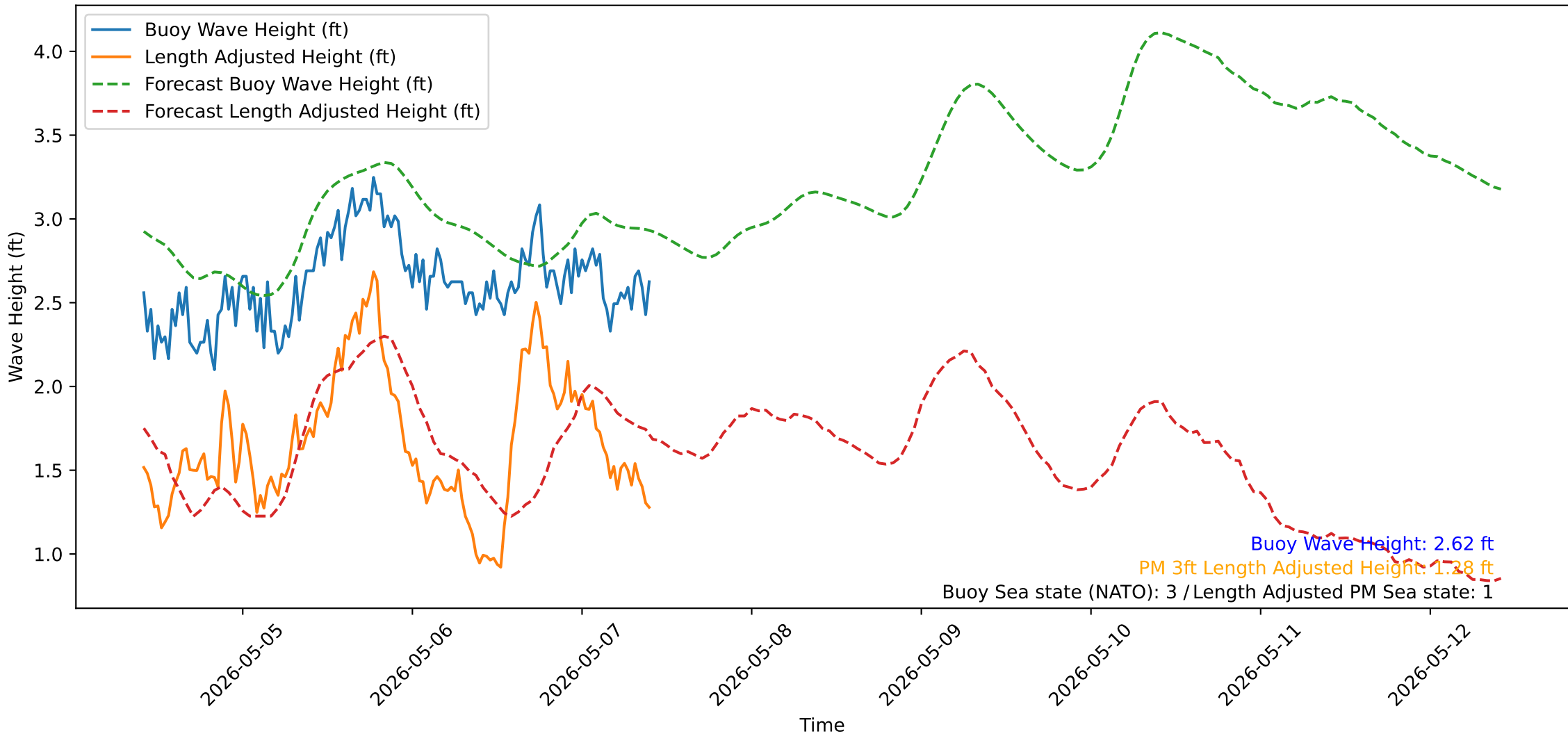
Wave Heights over Time for Oceanside Harbor at 2026-05-07 10:10:31
