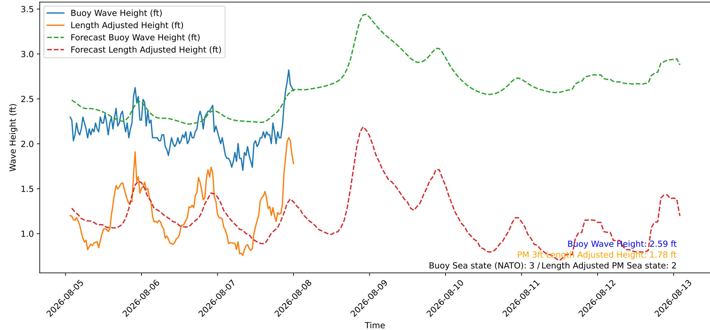
Wave Heights over Time for Green Beach at 2026-08-08 01:31:07
