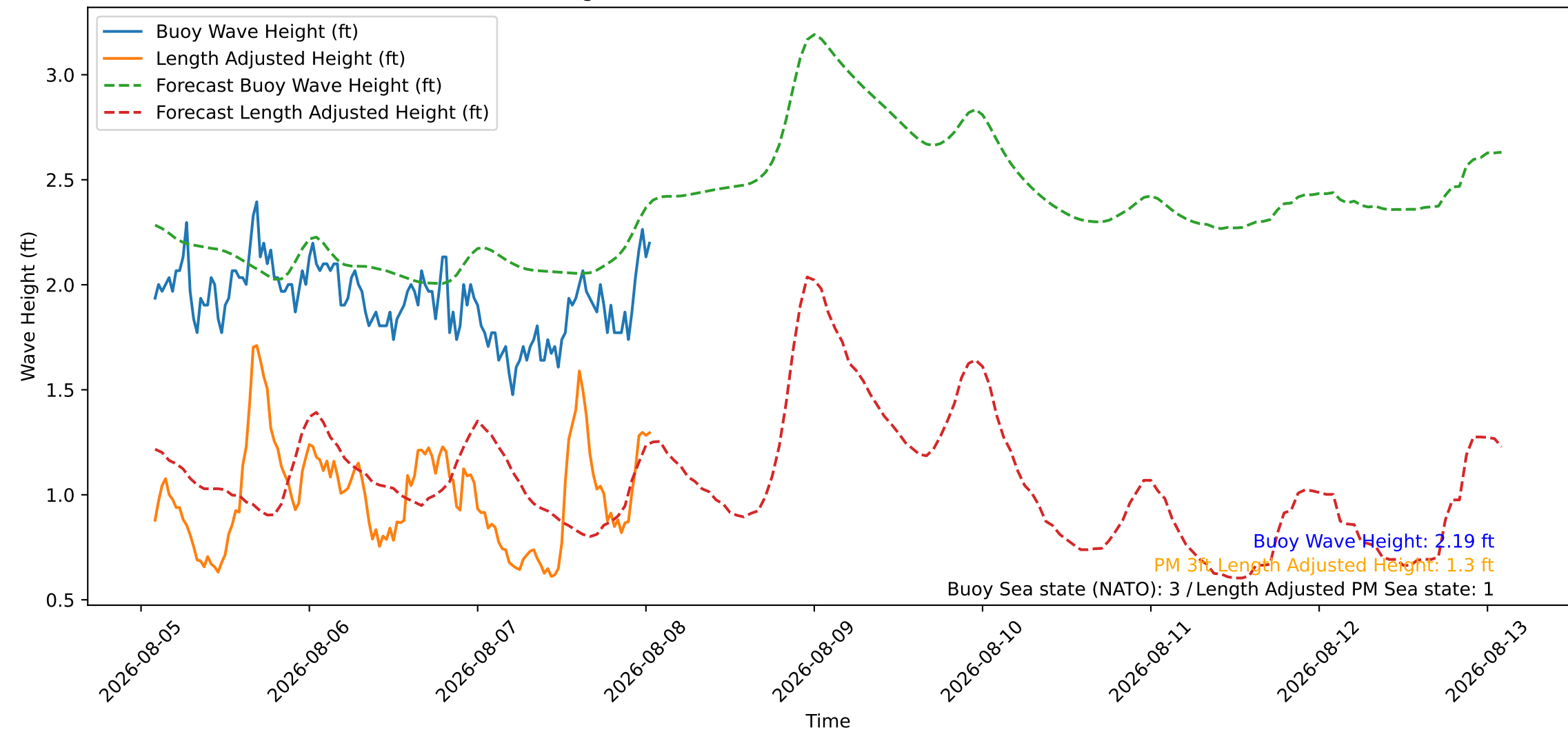
Wave Heights over Time for Red Beach at 2026-08-08 01:30:45
