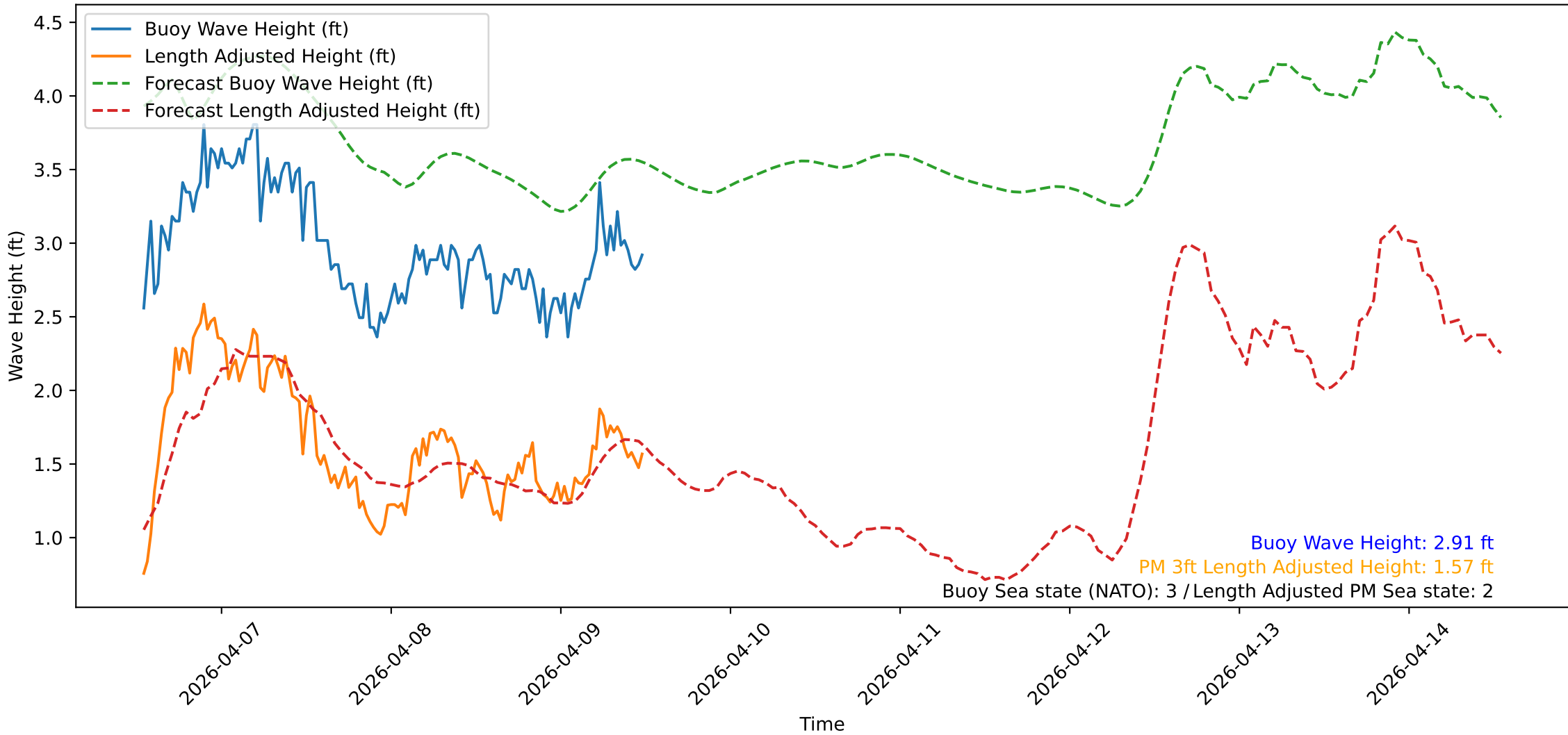
Wave Heights over Time for Green Beach at 2026-04-09 13:11:09
