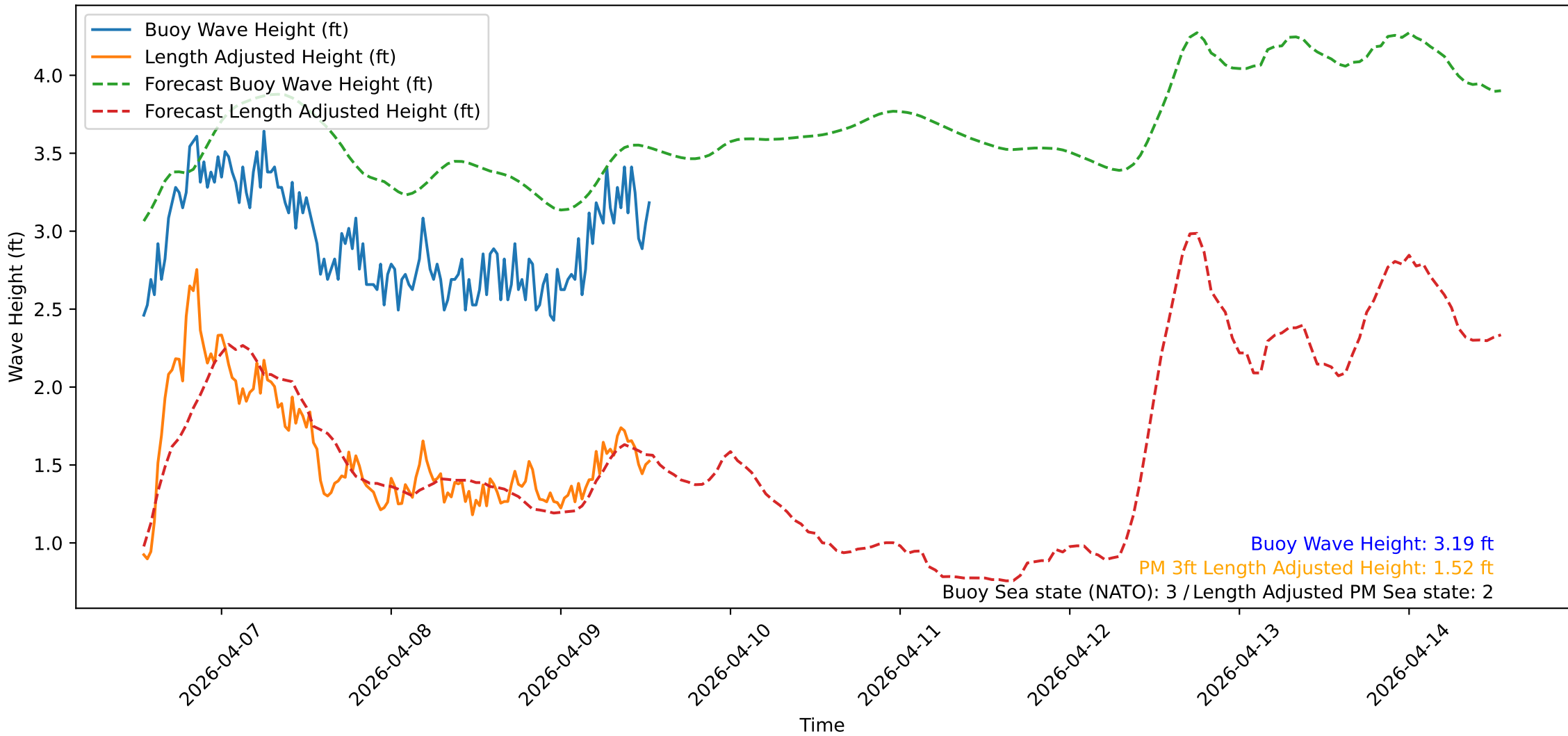
Wave Heights over Time for Oceanside Harbor at 2026-04-09 13:10:32
