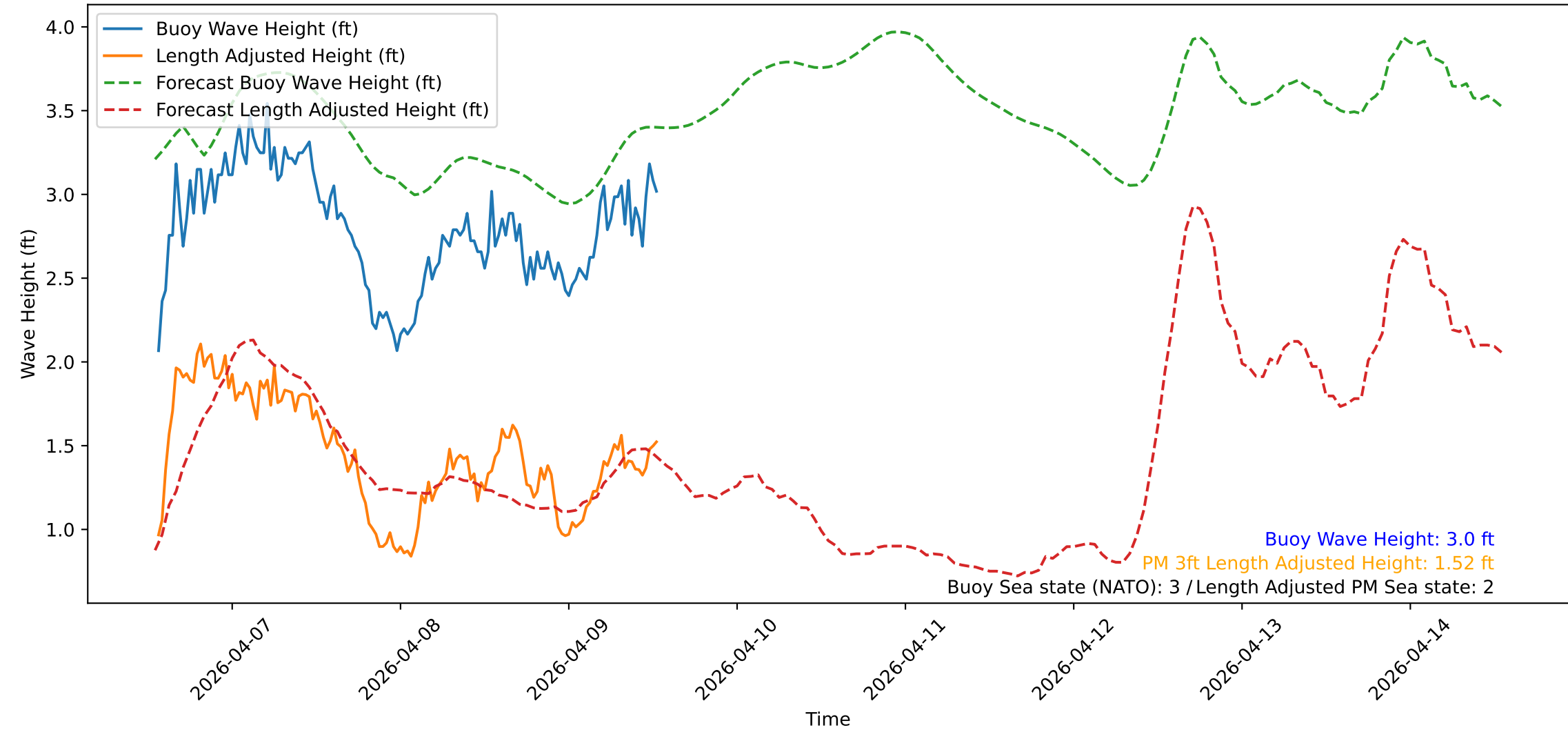
Wave Heights over Time for Red Beach at 2026-04-09 13:10:48
