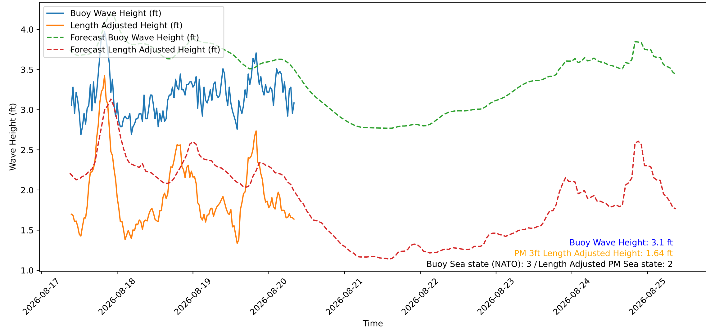
Wave Heights over Time for Green Beach at 2026-08-20 09:01:09
