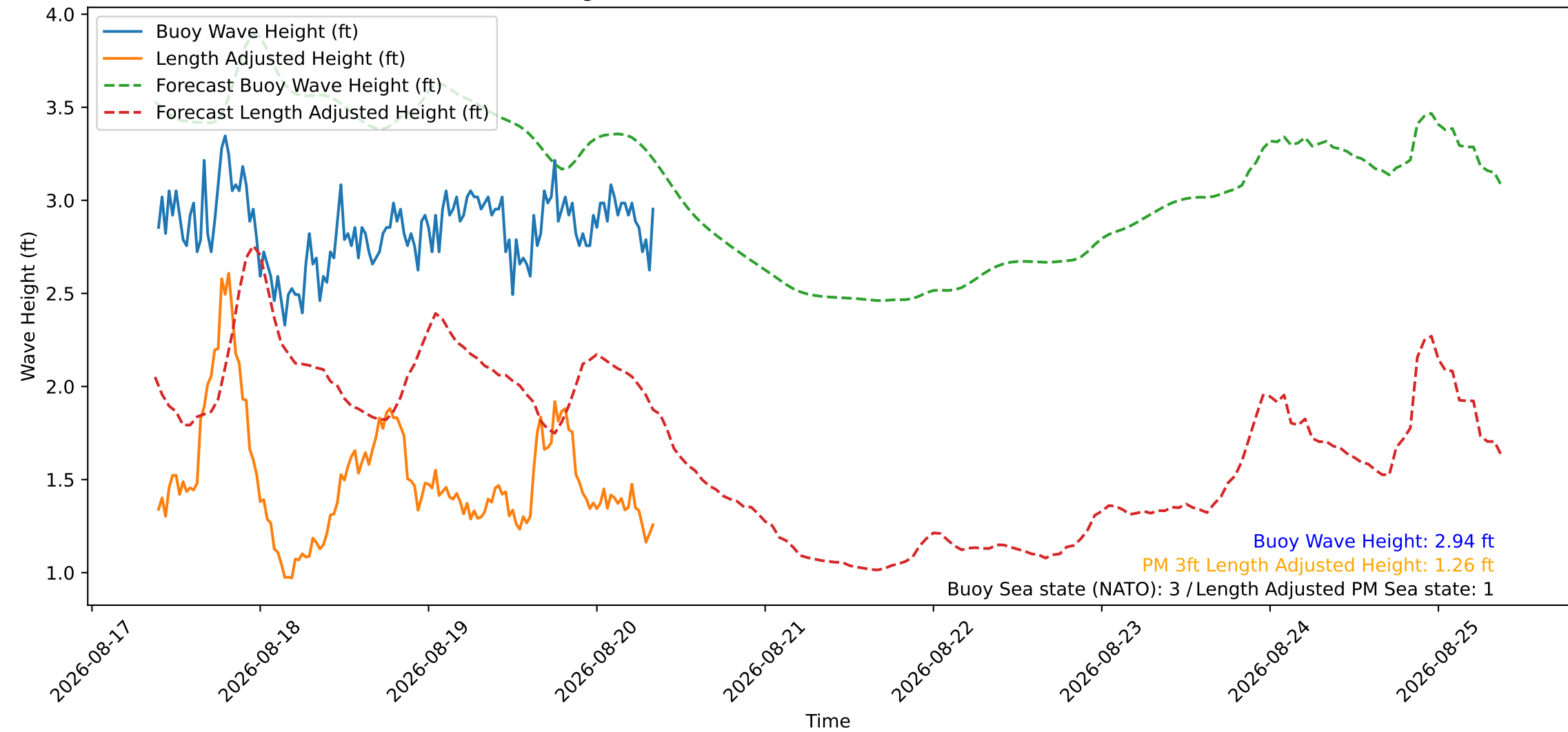
Wave Heights over Time for Red Beach at 2026-08-20 09:00:46
