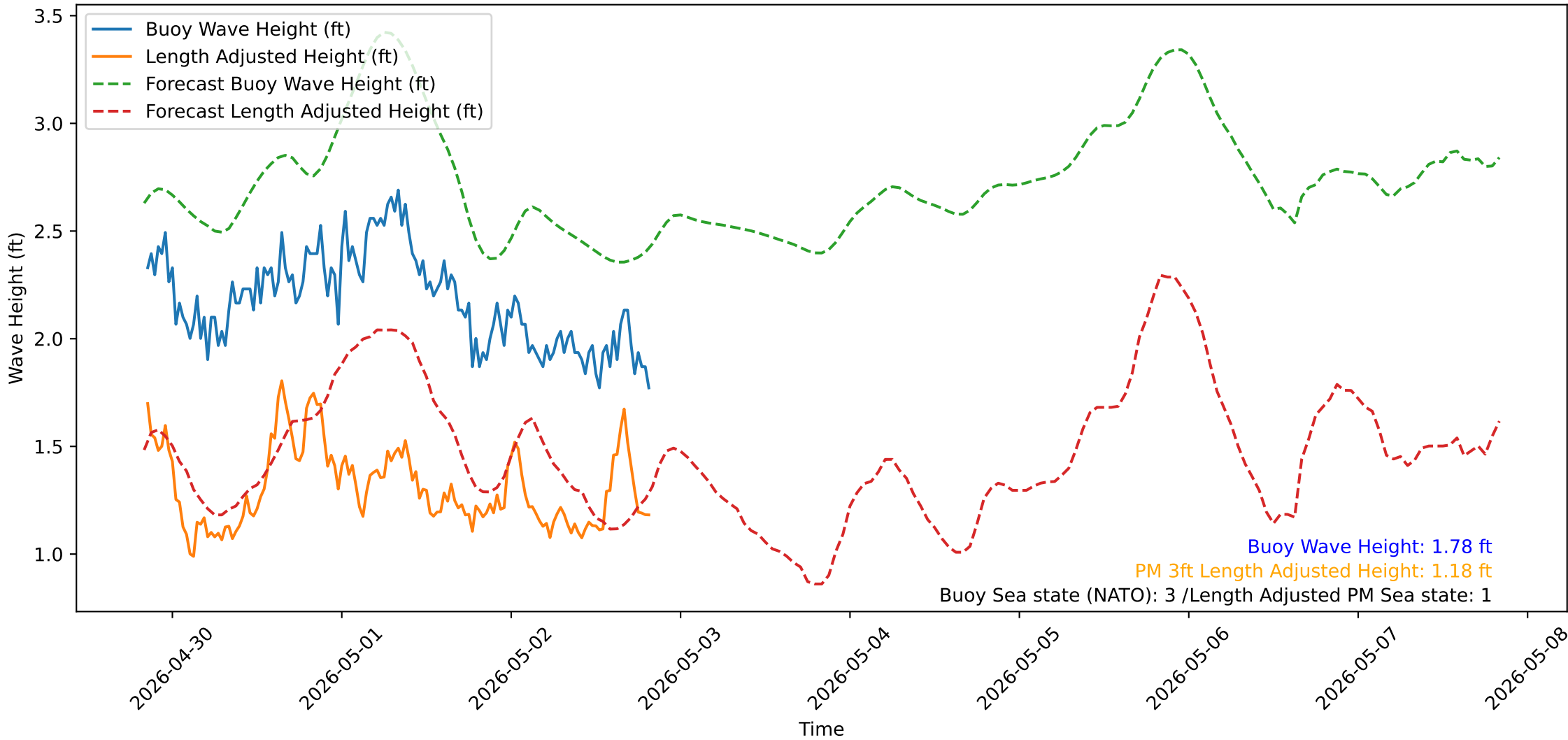
Wave Heights over Time for Oceanside Harbor at 2026-05-02 20:20:31
