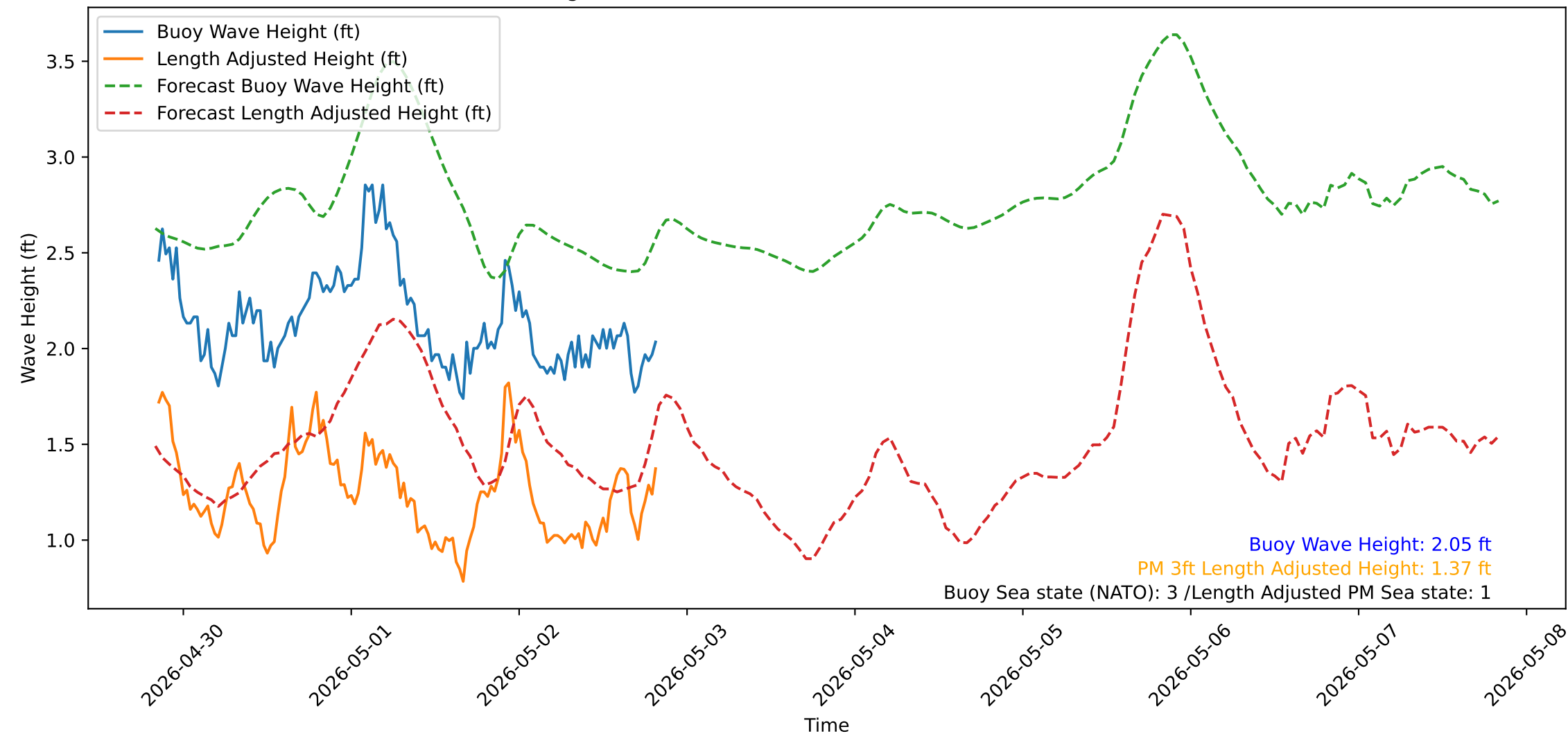
Wave Heights over Time for Green Beach at 2026-05-02 20:21:13
