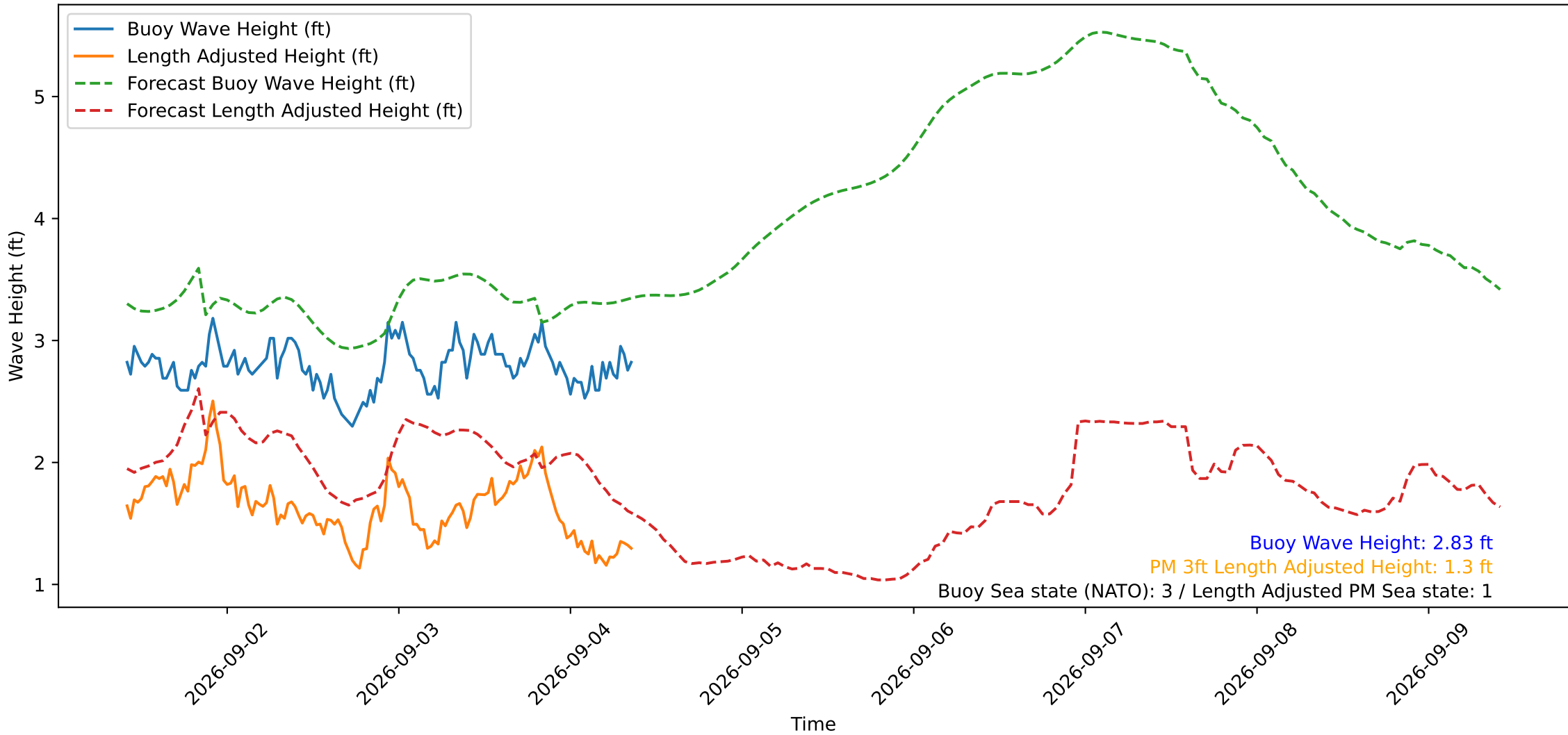
Wave Heights over Time for Red Beach at 2026-09-04 09:30:50
