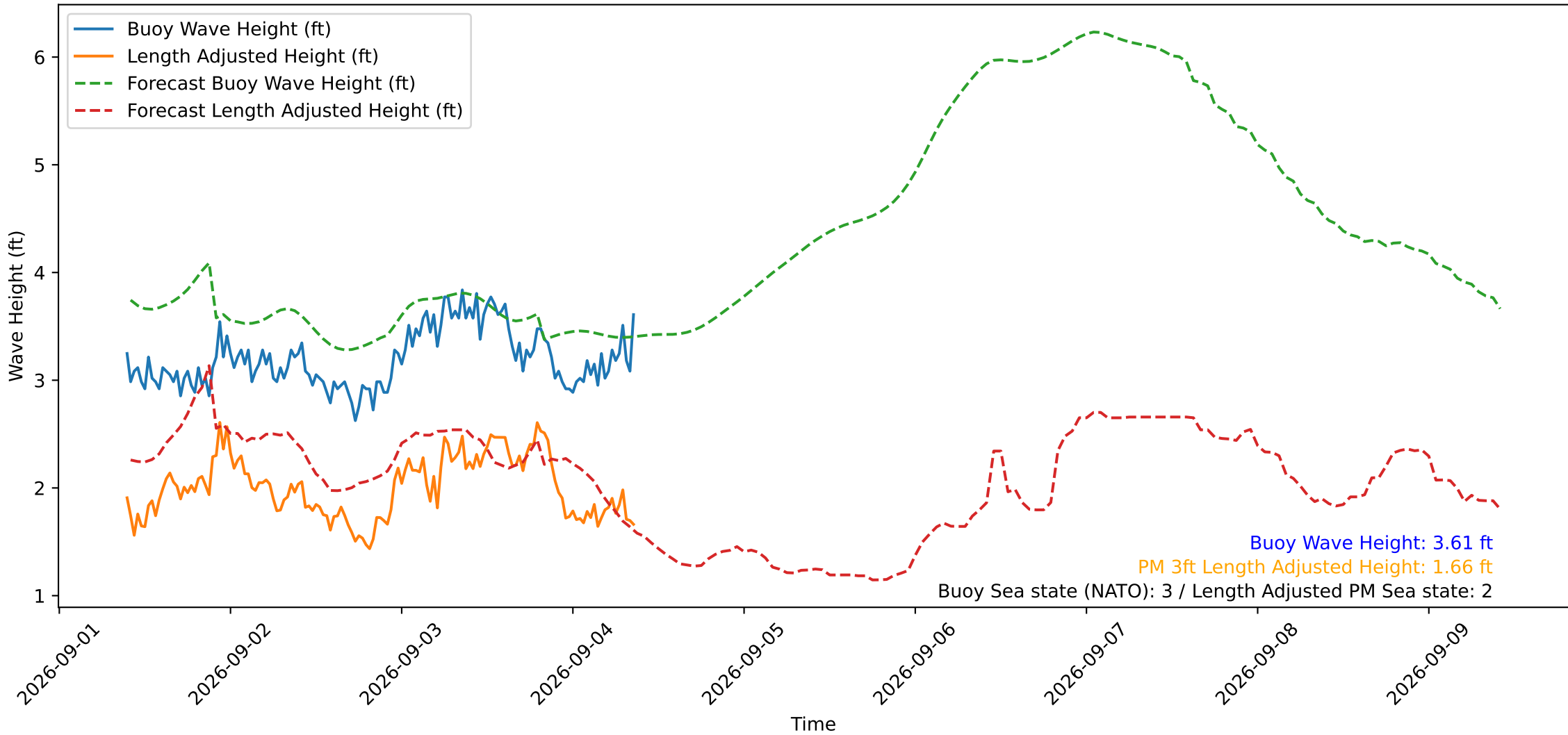
Wave Heights over Time for Oceanside Harbor at 2026-09-04 09:30:30
