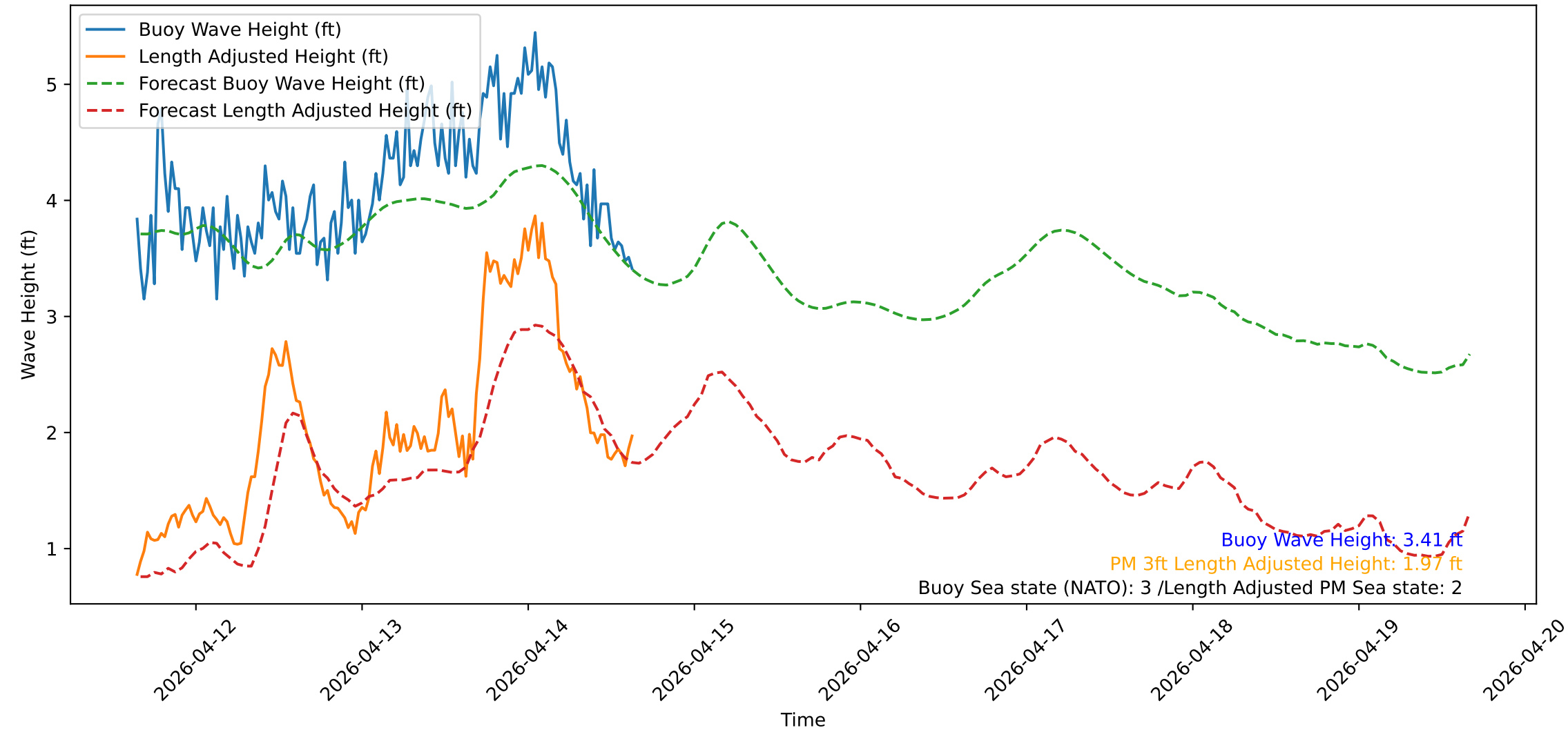
Wave Heights over Time for Oceanside Harbor at 2026-04-14 15:40:31
