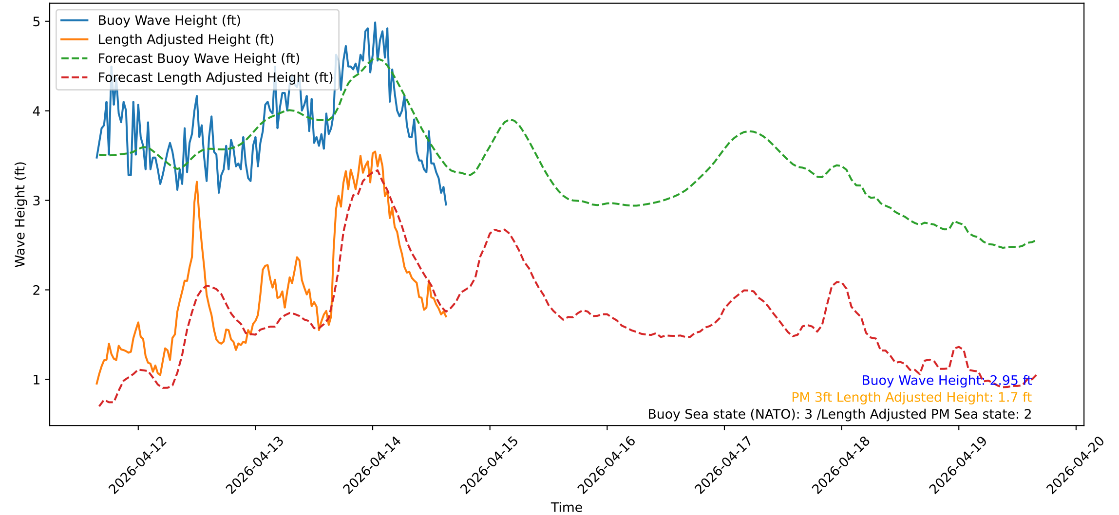
Wave Heights over Time for Green Beach at 2026-04-14 15:41:12
