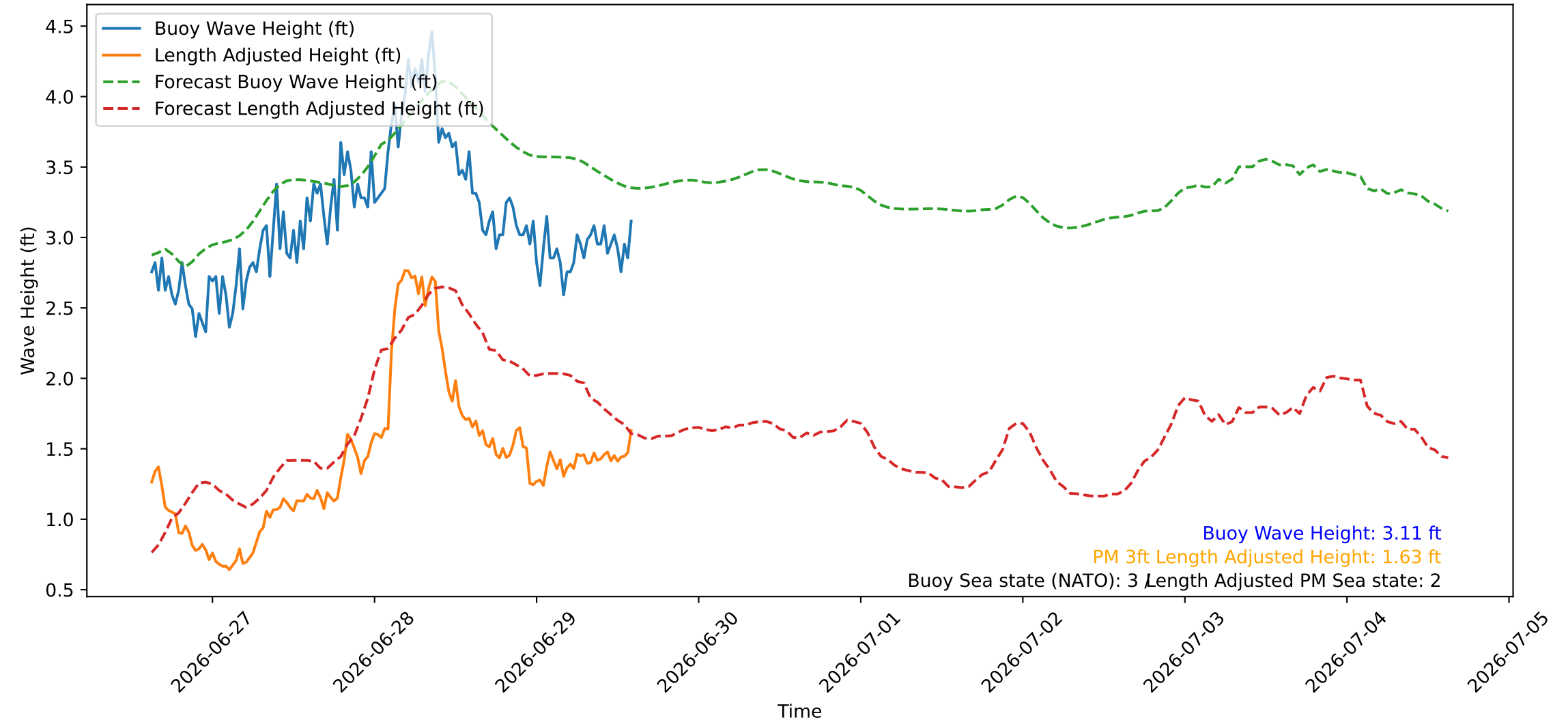
Wave Heights over Time for Red Beach at 2026-06-29 14:50:46
