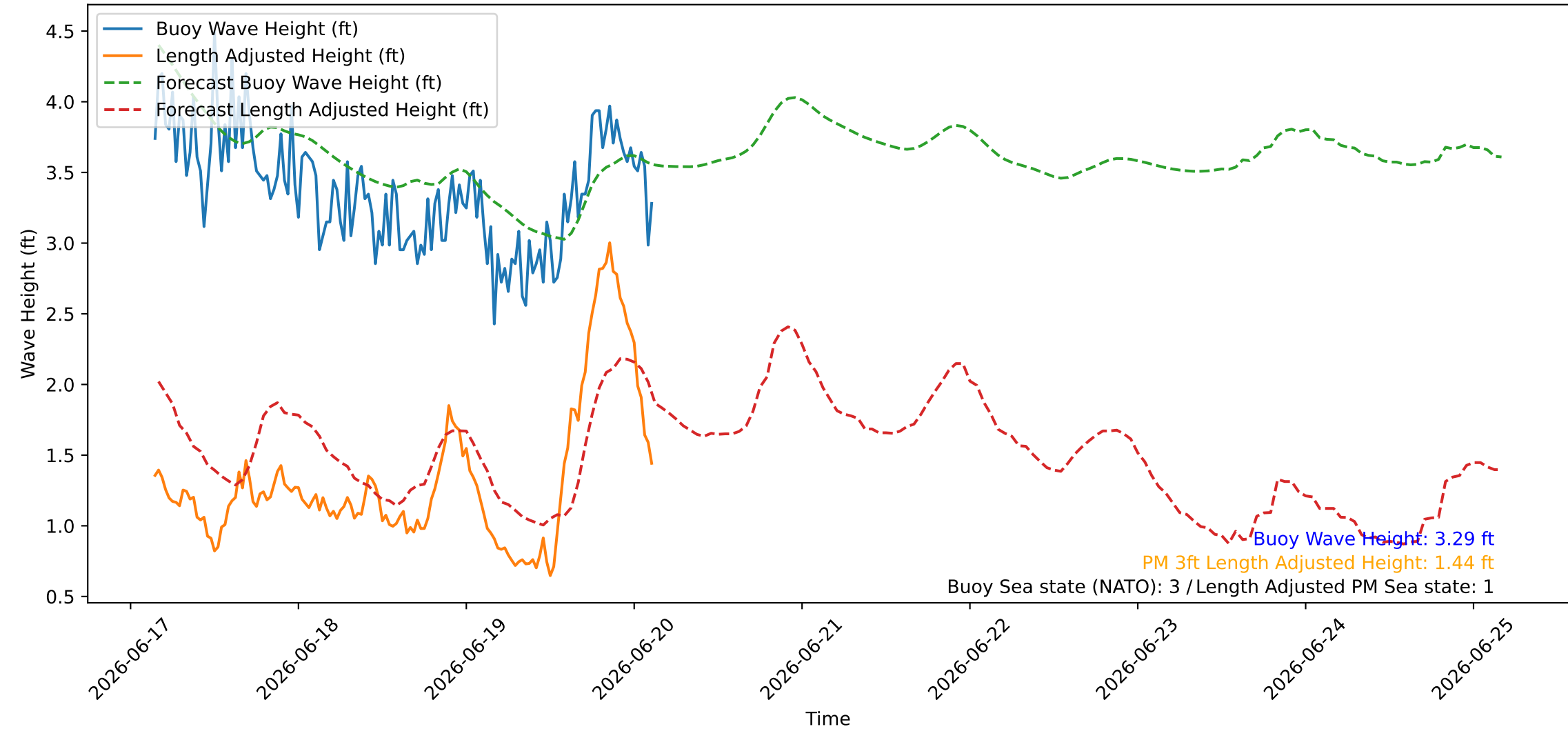
Wave Heights over Time for Green Beach at 2026-06-20 03:31:07
