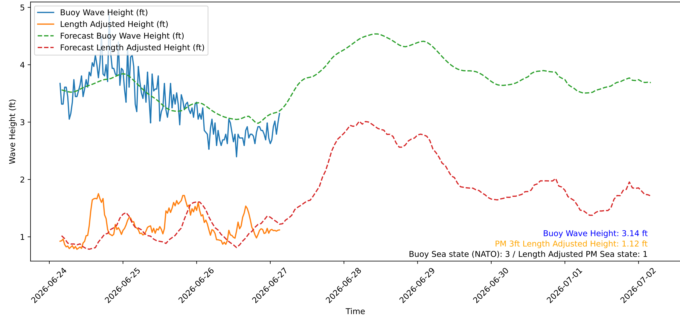
Wave Heights over Time for Oceanside Harbor at 2026-06-27 03:40:26
