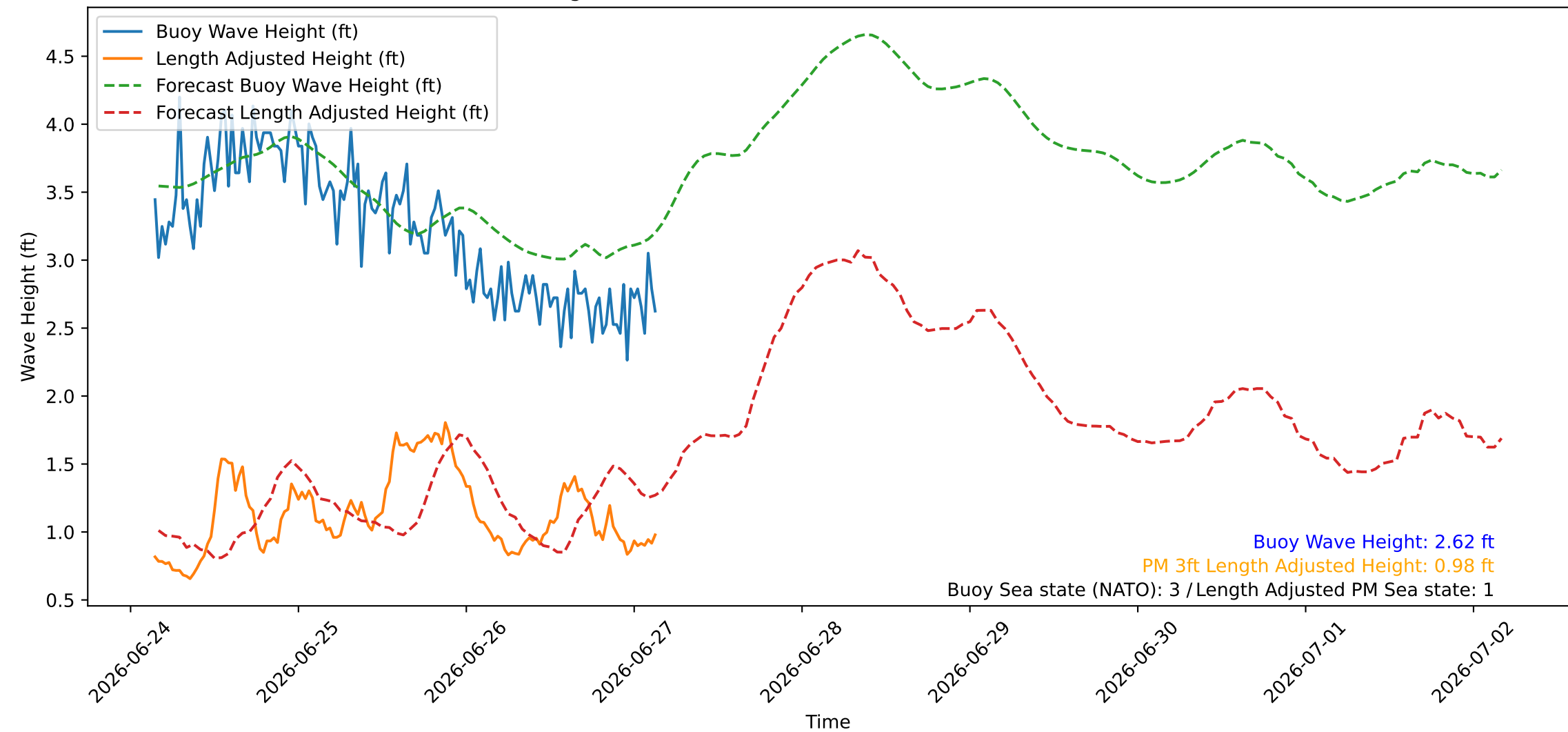
Wave Heights over Time for Green Beach at 2026-06-27 03:41:08
