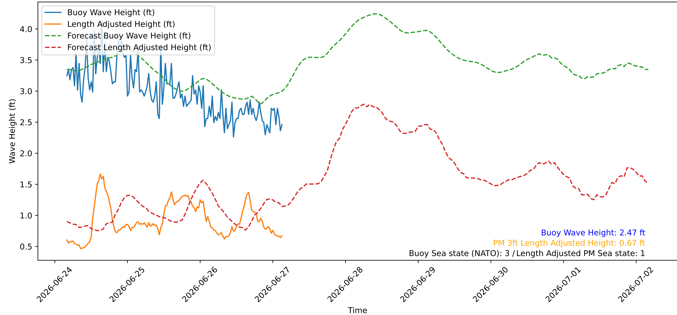
Wave Heights over Time for Red Beach at 2026-06-27 03:40:45
