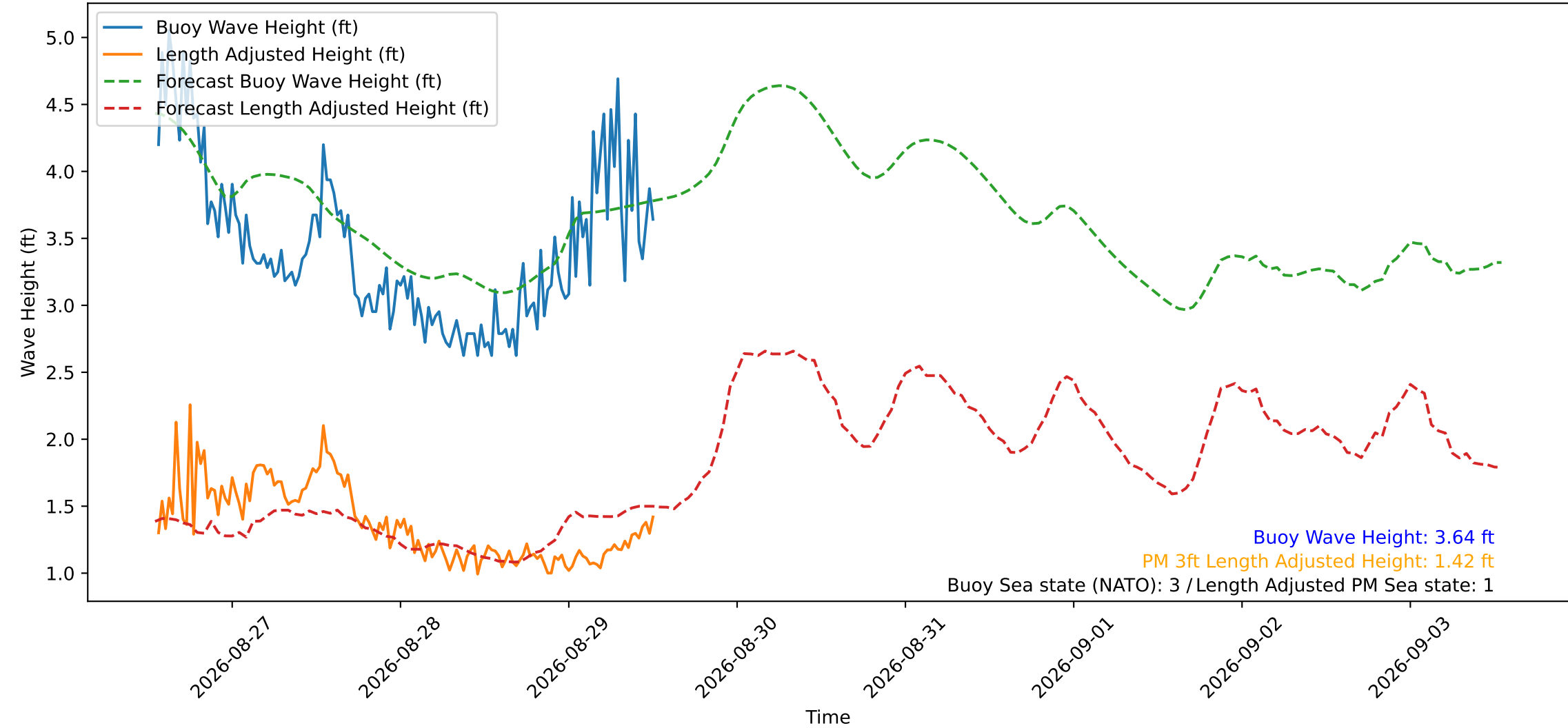
Wave Heights over Time for Red Beach at 2026-08-29 13:00:49
