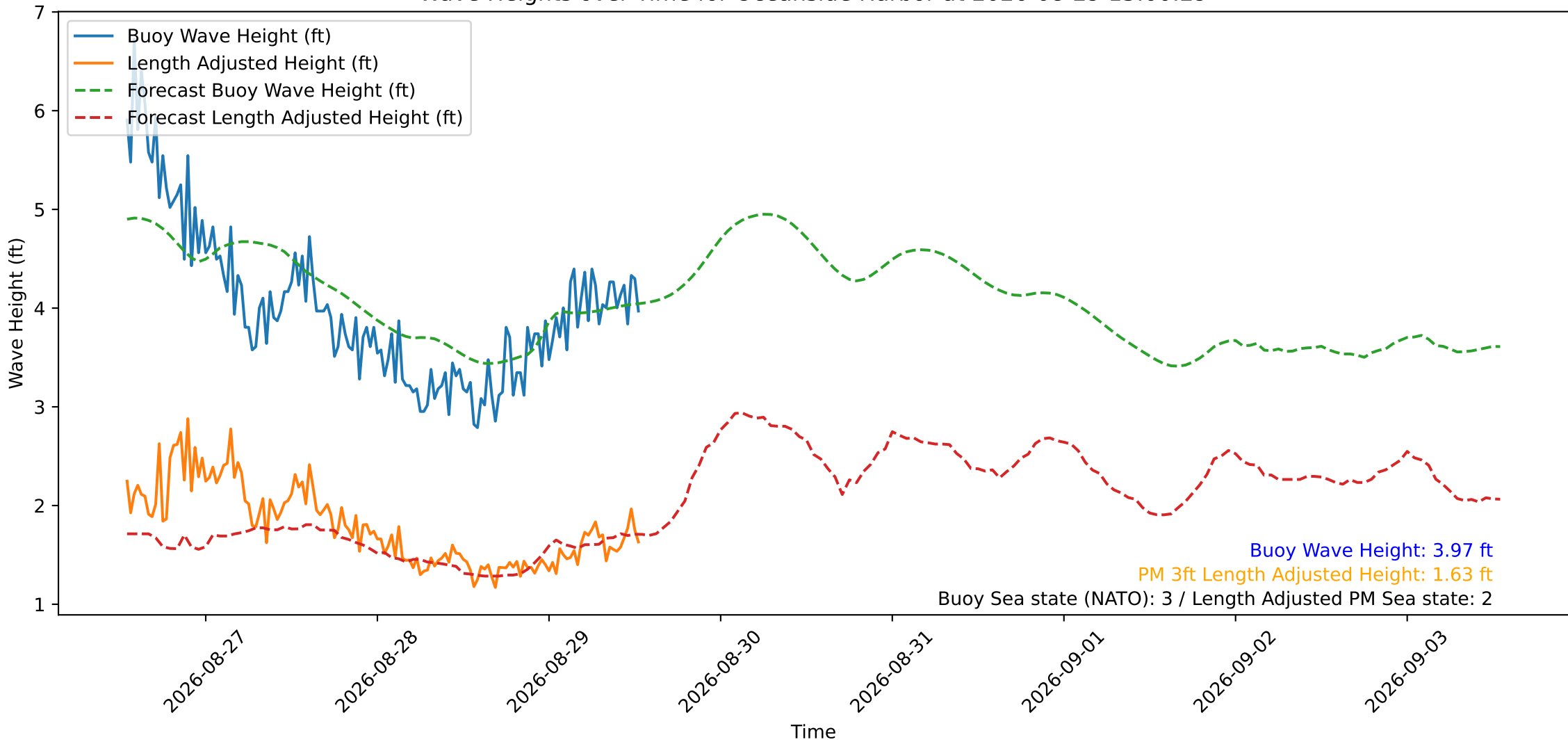
Wave Heights over Time for Oceanside Harbor at 2026-08-29 13:00:29
