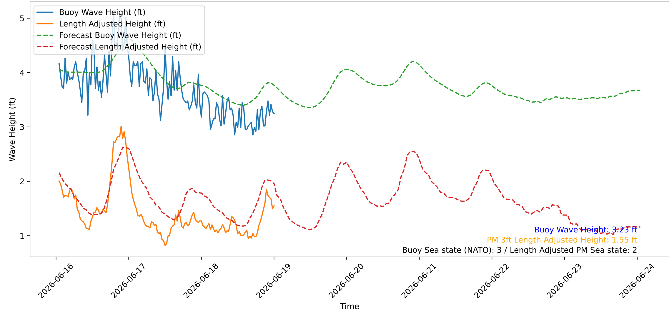
Wave Heights over Time for Green Beach at 2026-06-19 00:51:09
