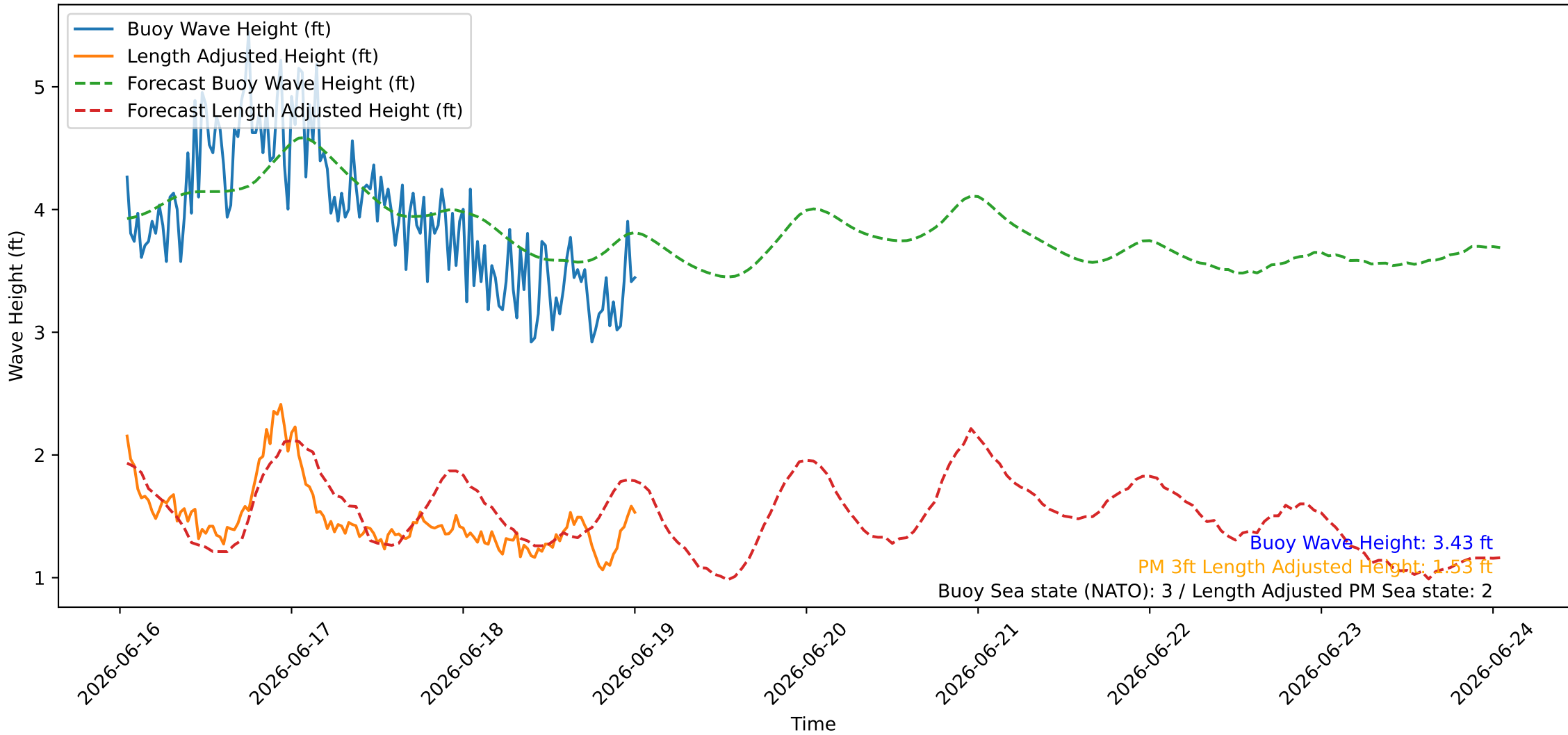
Wave Heights over Time for Oceanside Harbor at 2026-06-19 00:50:26
