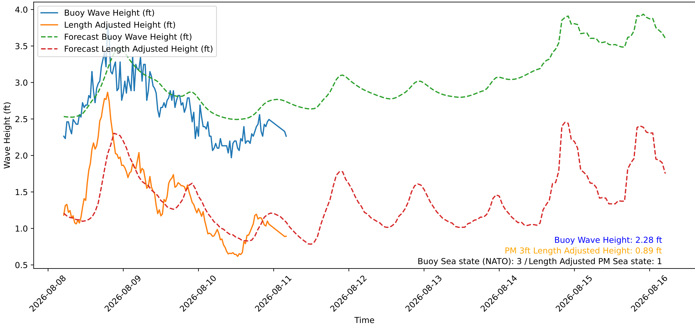
Wave Heights over Time for Green Beach at 2026-08-11 05:01:09
