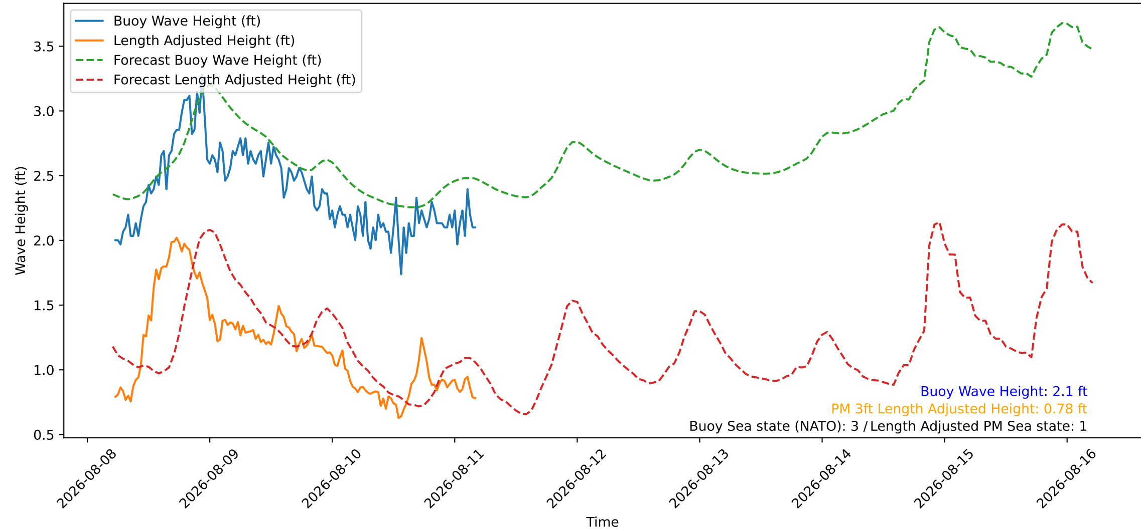
Wave Heights over Time for Red Beach at 2026-08-11 05:00:46
