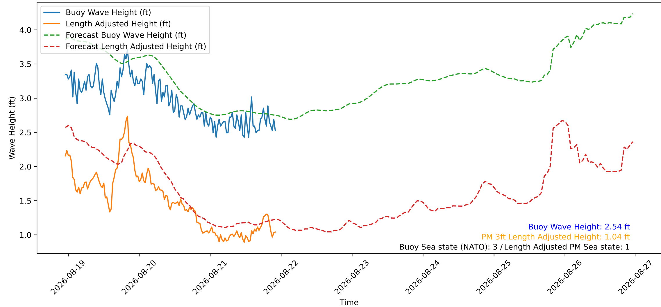
Wave Heights over Time for Green Beach at 2026-08-21 22:41:11
