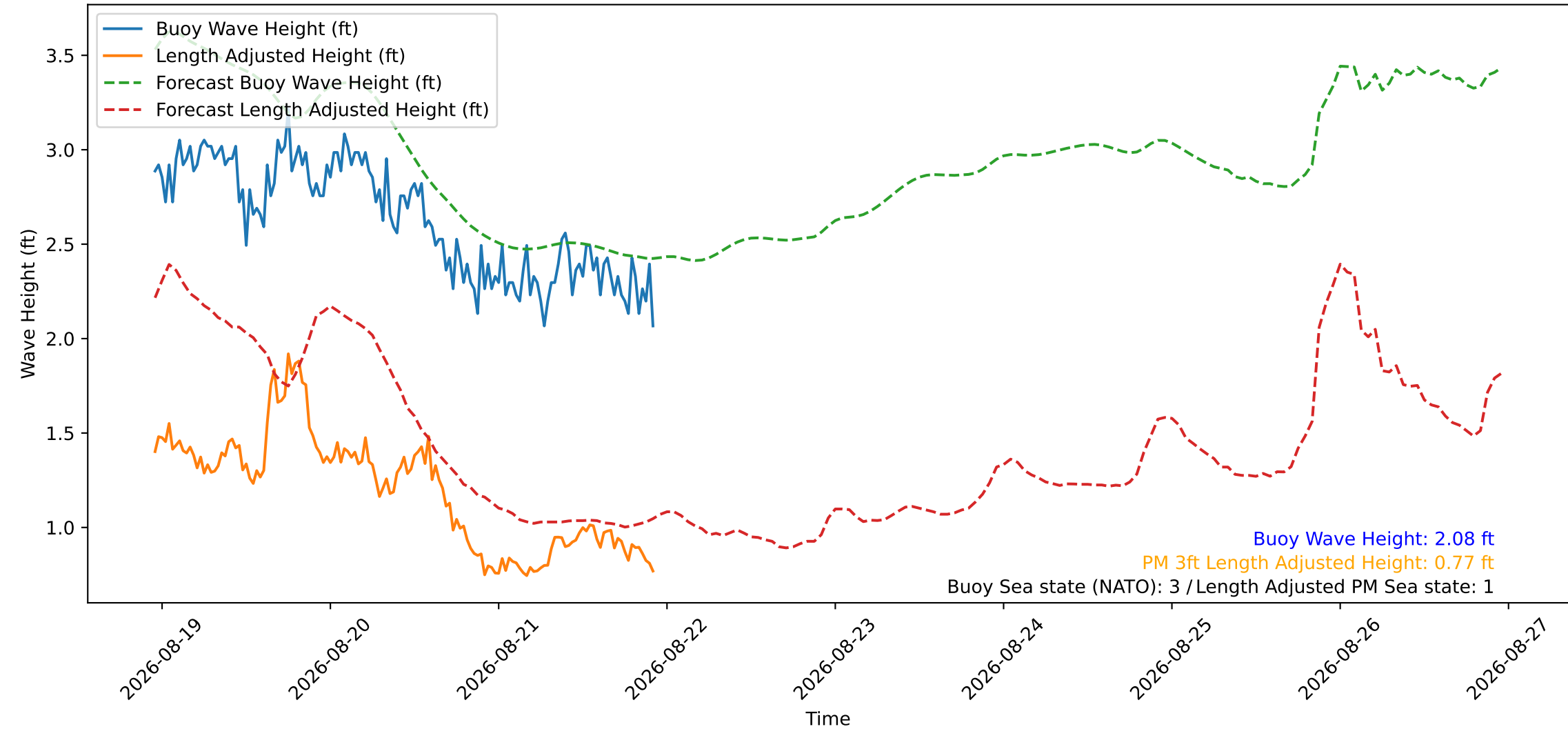
Wave Heights over Time for Red Beach at 2026-08-21 22:40:48
