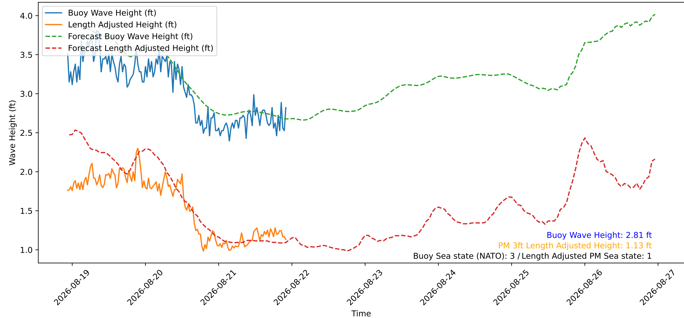
Wave Heights over Time for Oceanside Harbor at 2026-08-21 22:40:29
