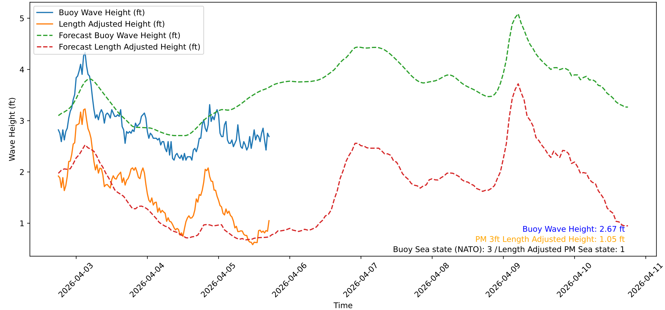
Wave Heights over Time for Green Beach at 2026-04-05 18:01:17
