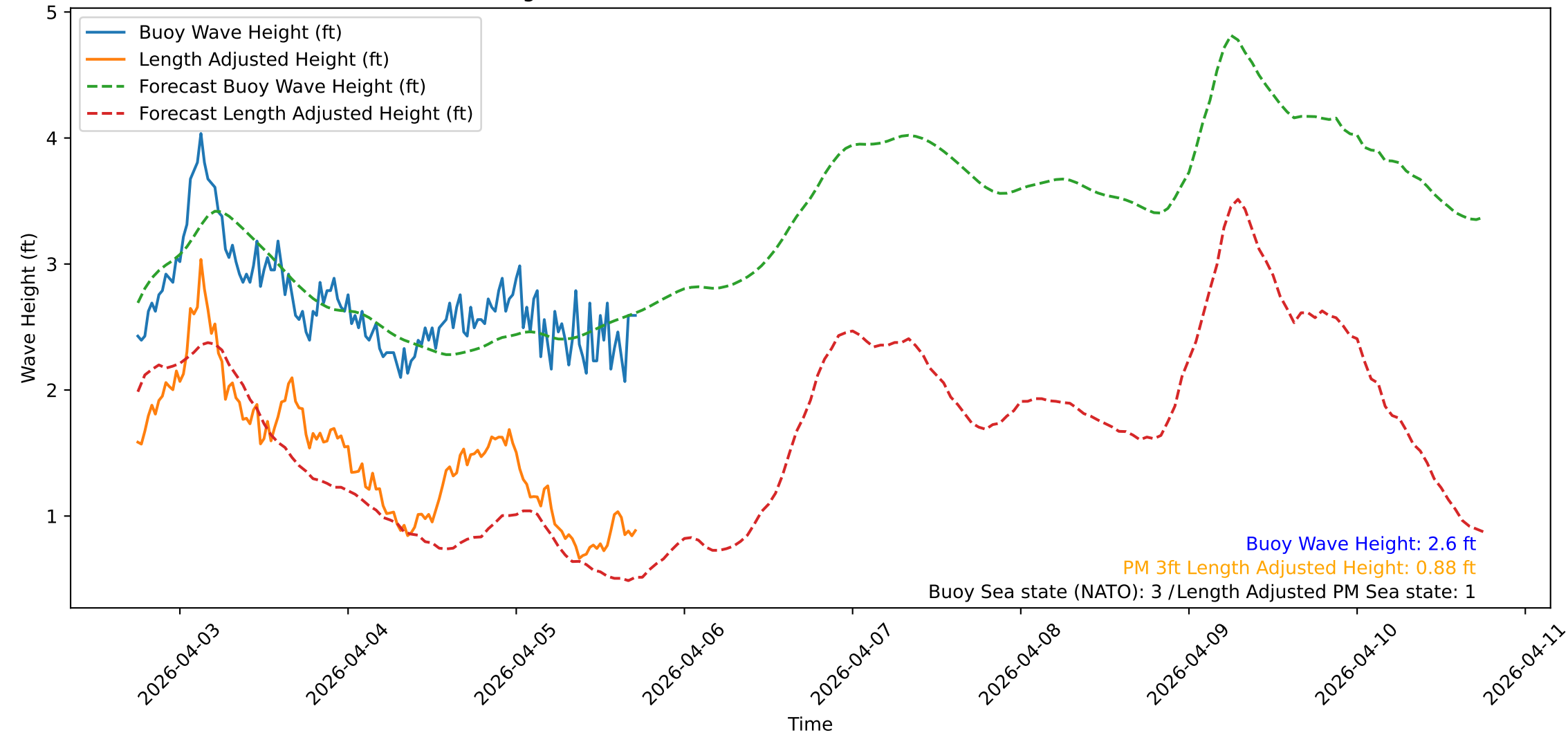
Wave Heights over Time for Oceanside Harbor at 2026-04-05 18:00:34
