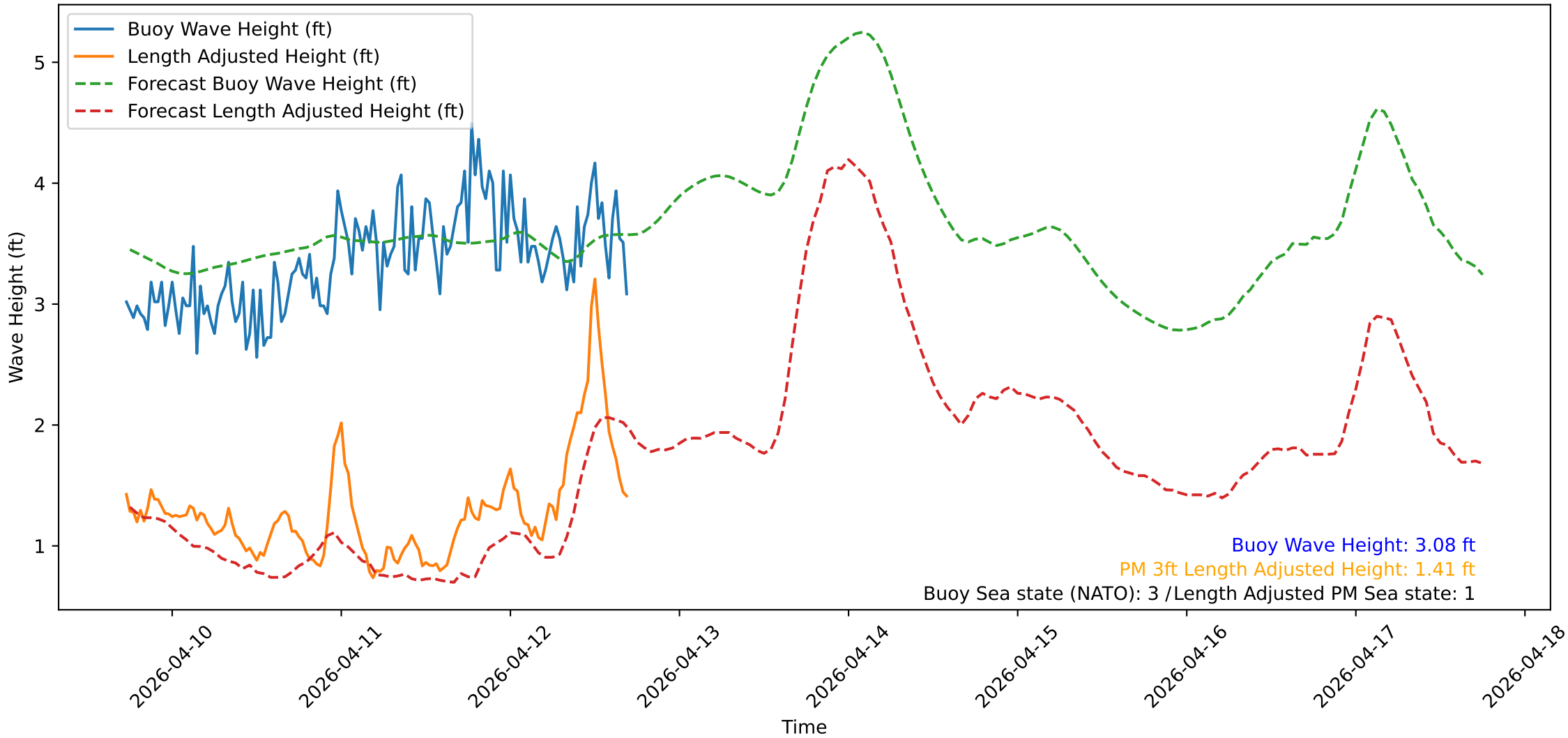
Wave Heights over Time for Green Beach at 2026-04-12 17:31:11
