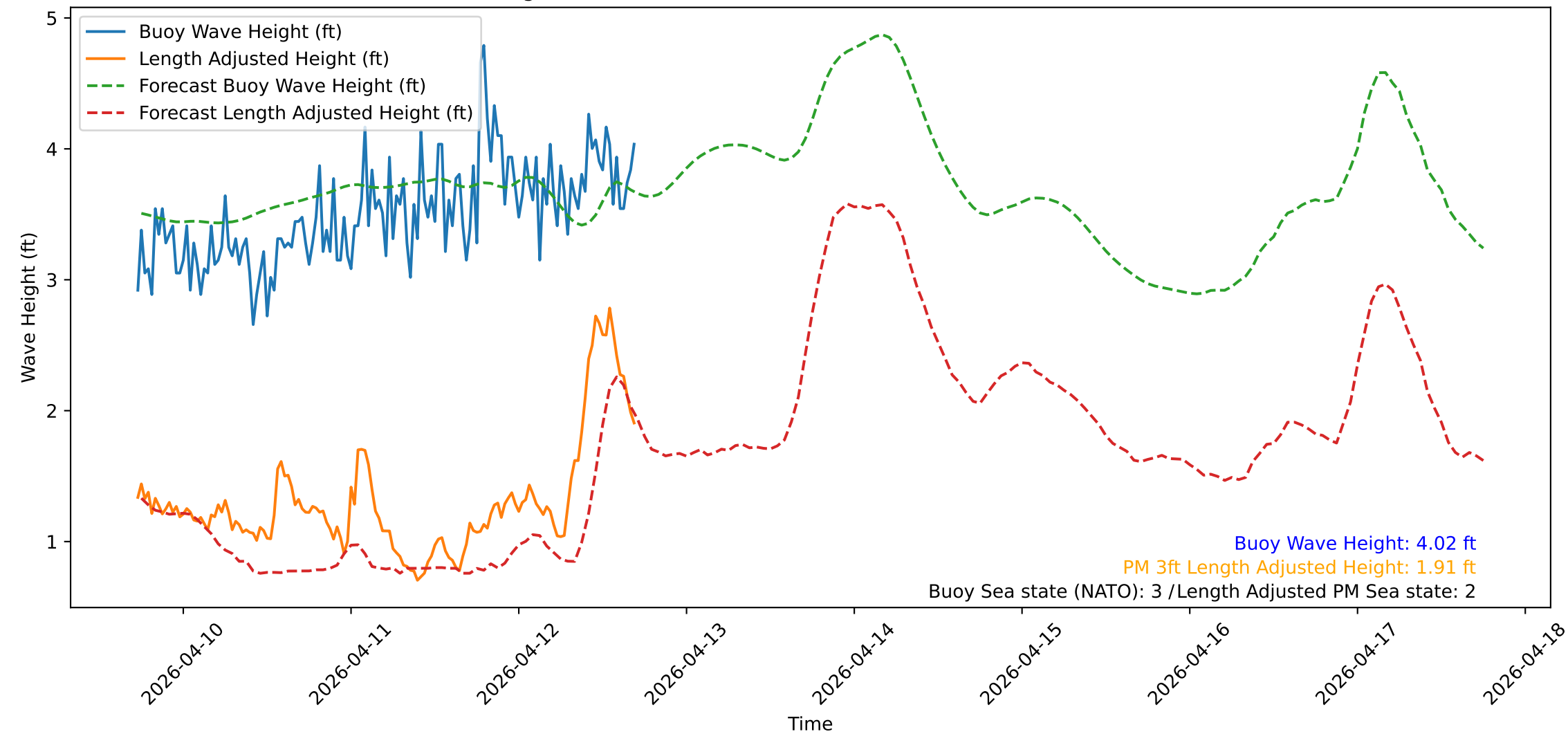
Wave Heights over Time for Oceanside Harbor at 2026-04-12 17:30:31
