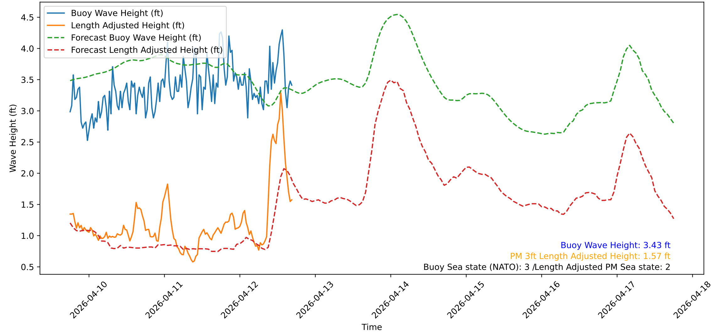
Wave Heights over Time for Red Beach at 2026-04-12 17:30:49
