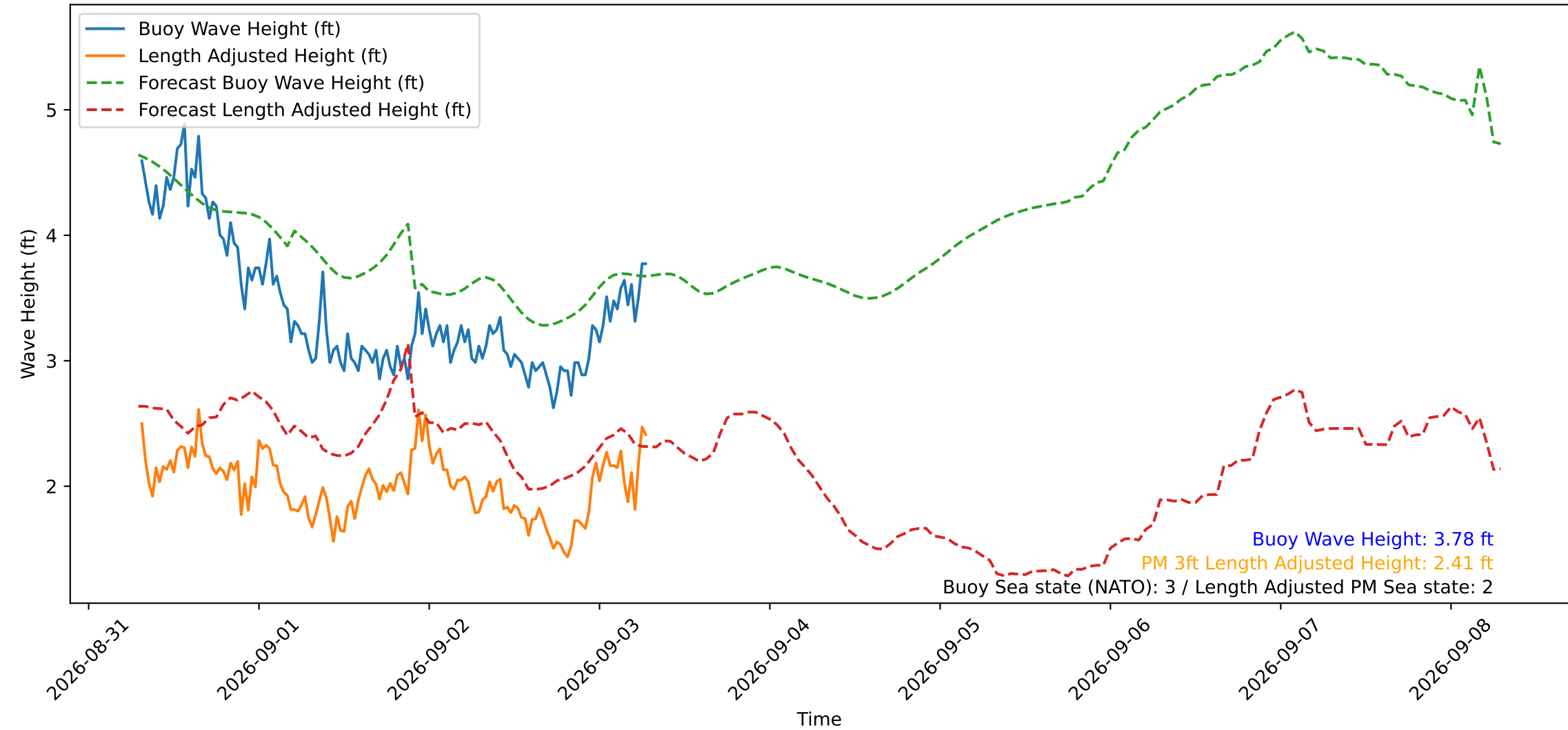
Wave Heights over Time for Oceanside Harbor at 2026-09-03 07:20:29
