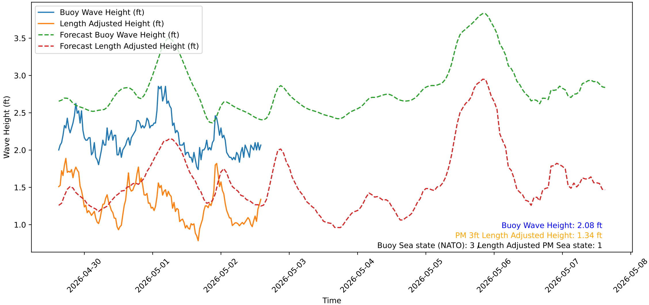
Wave Heights over Time for Green Beach at 2026-05-02 15:01:13
