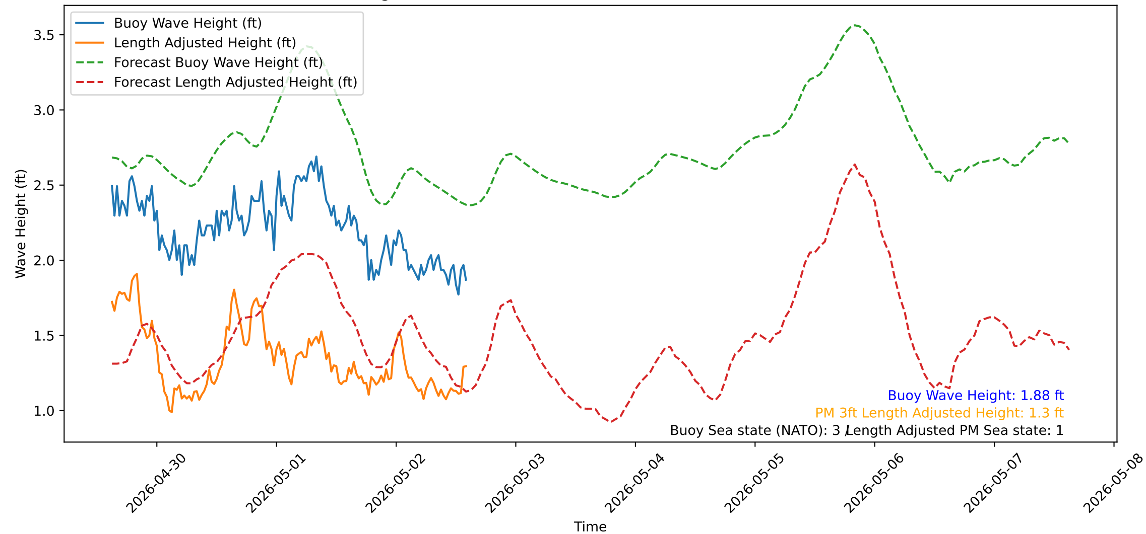
Wave Heights over Time for Oceanside Harbor at 2026-05-02 15:00:31
