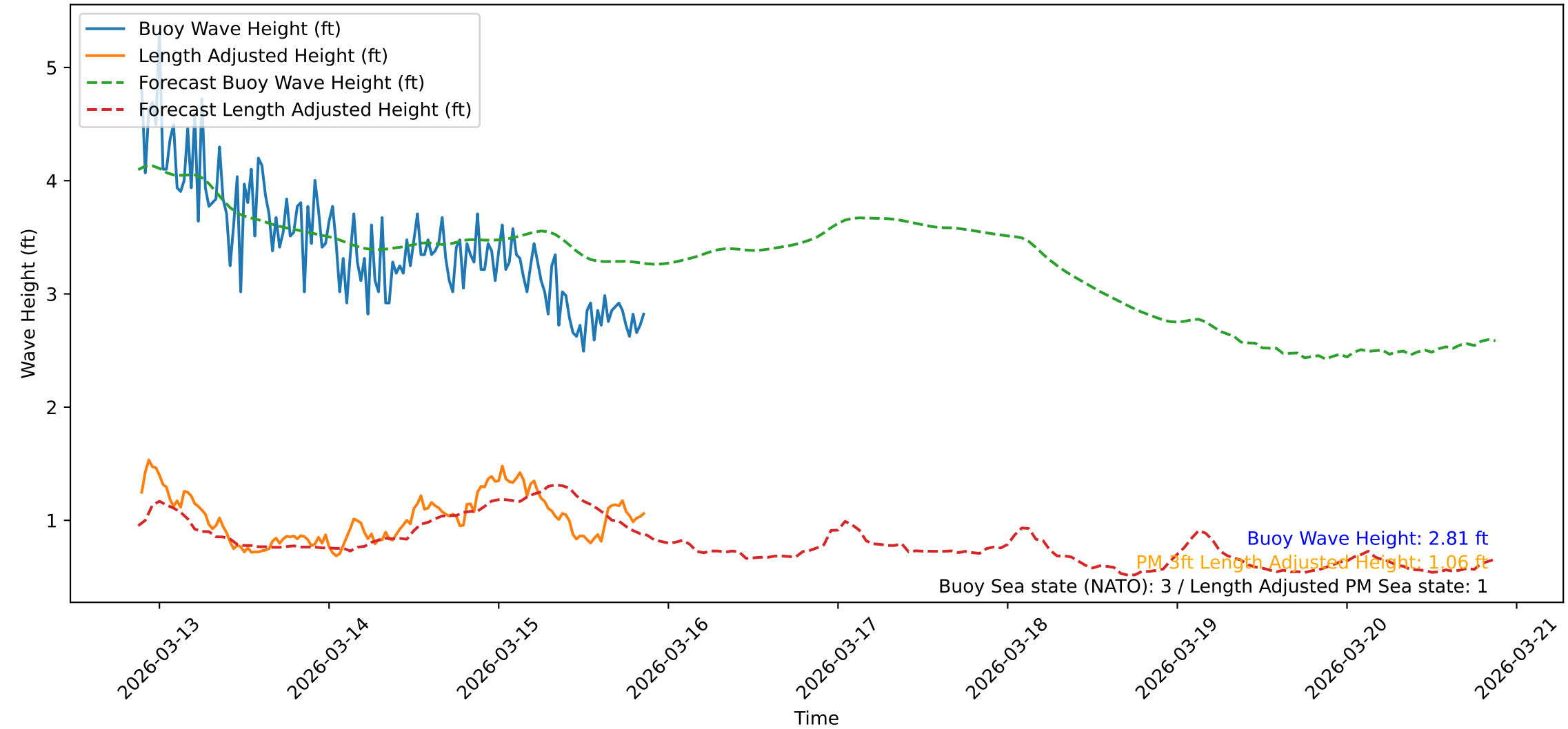
Wave Heights over Time for Oceanside Harbor at 2026-03-15 21:20:47
