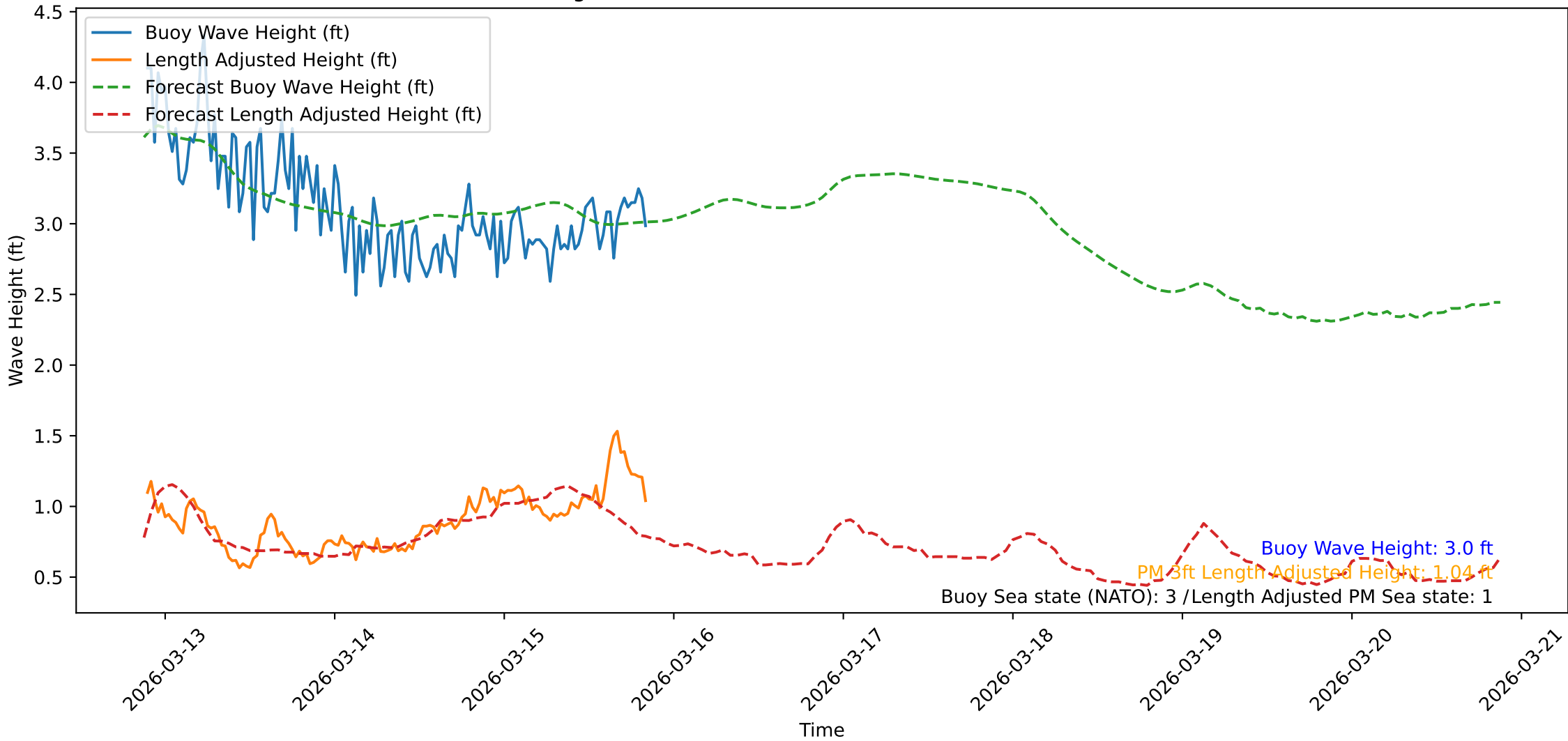
Wave Heights over Time for Red Beach at 2026-03-15 21:21:12
