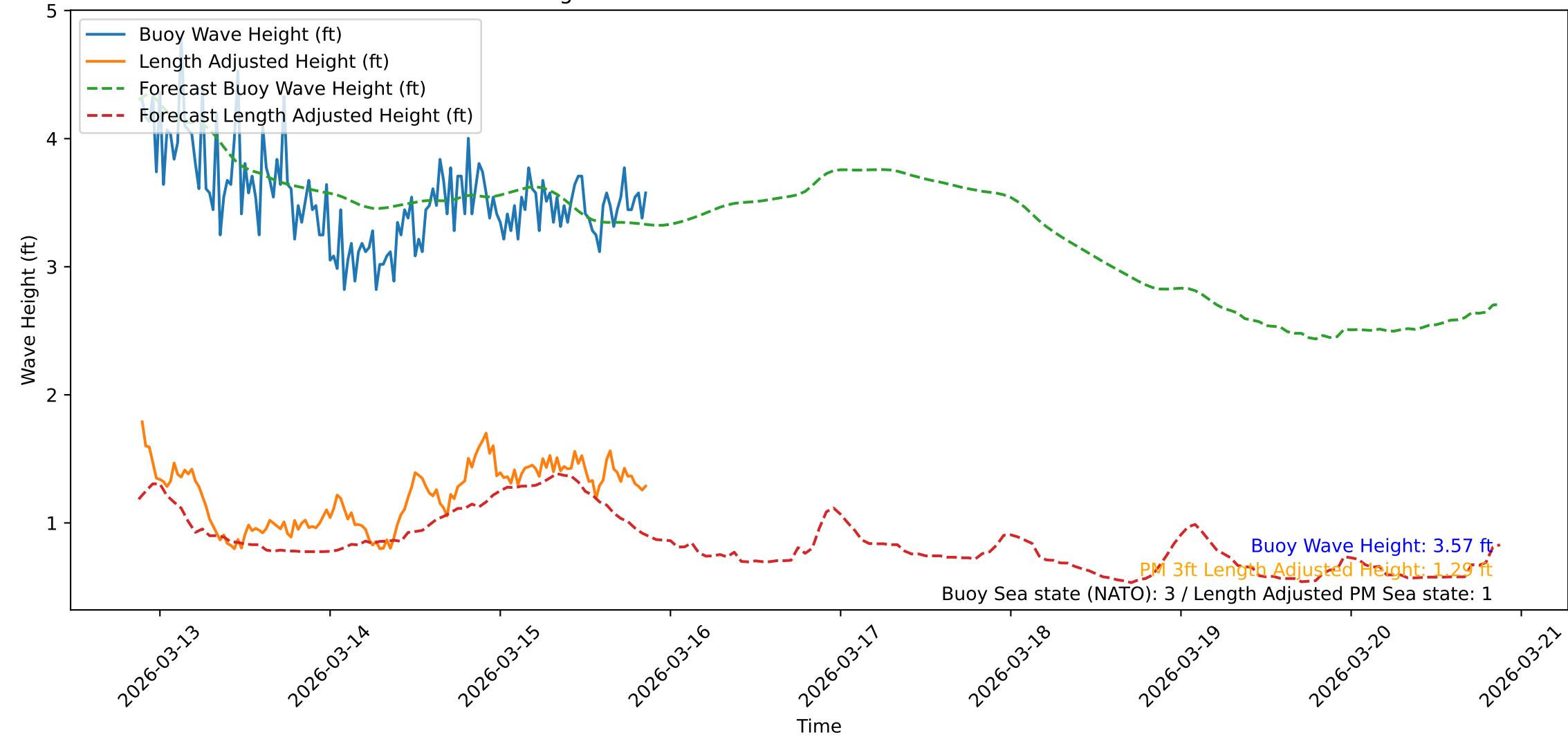
Wave Heights over Time for Green Beach at 2026-03-15 21:21:51
