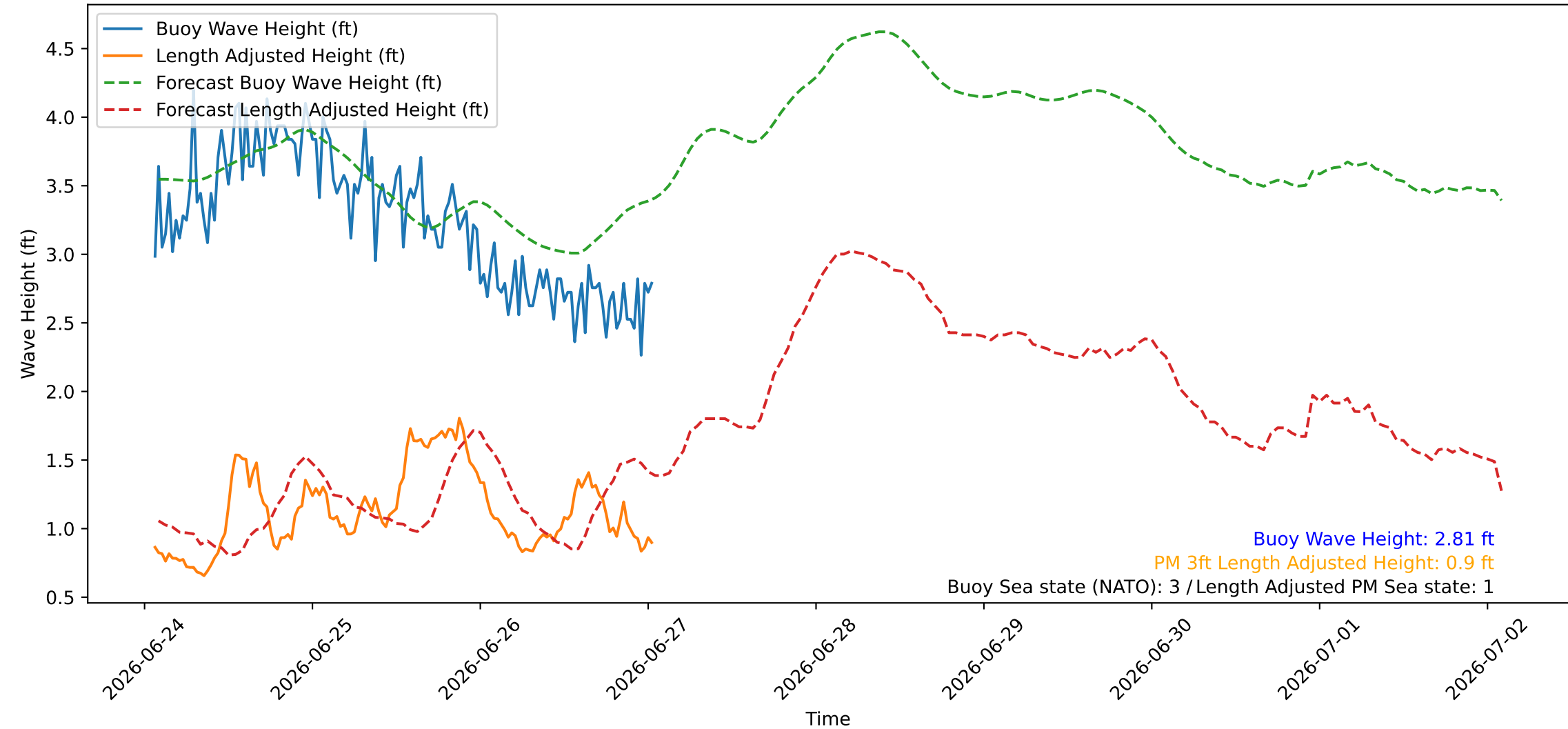
Wave Heights over Time for Green Beach at 2026-06-27 01:31:08
