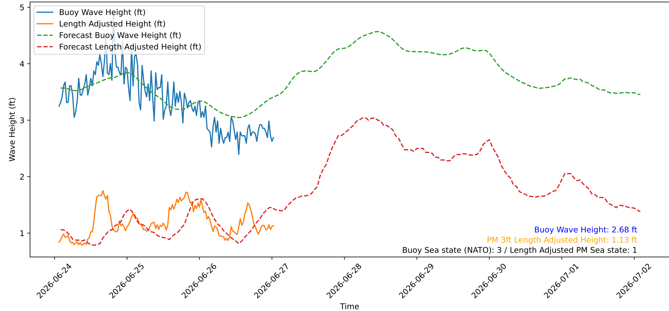
Wave Heights over Time for Oceanside Harbor at 2026-06-27 01:30:26
