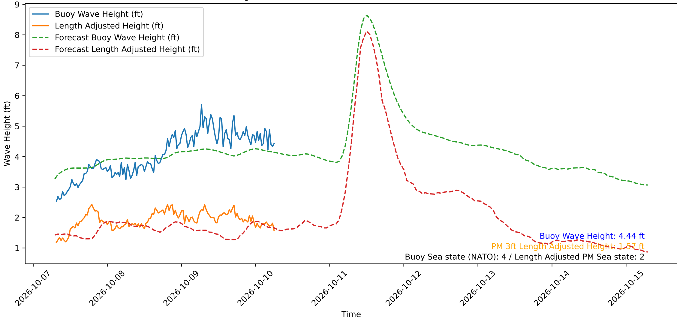
Wave Heights over Time for Red Beach at 2026-10-10 07:00:49
