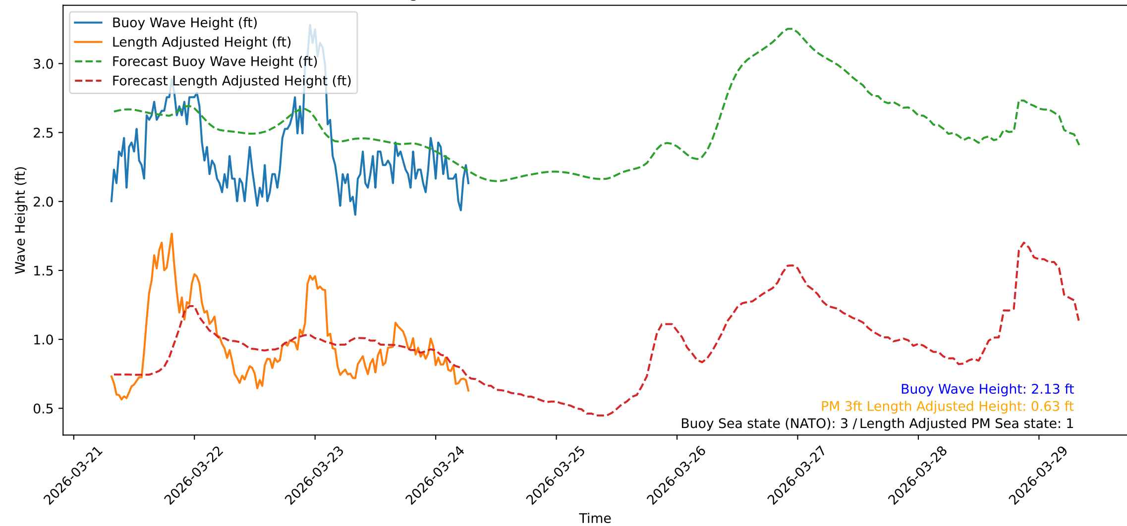
Wave Heights over Time for Green Beach at 2026-03-24 07:31:09
