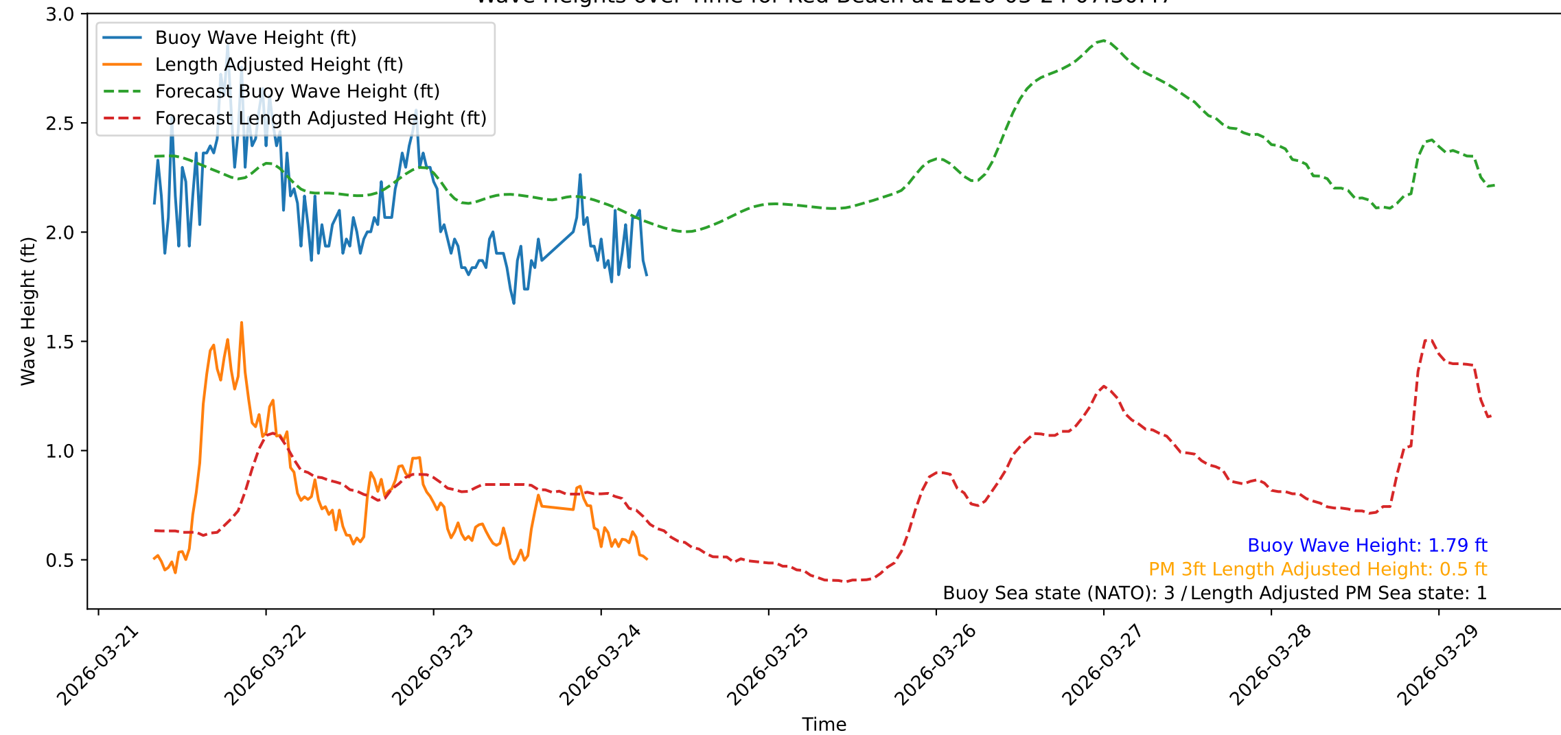
Wave Heights over Time for Red Beach at 2026-03-24 07:30:47
