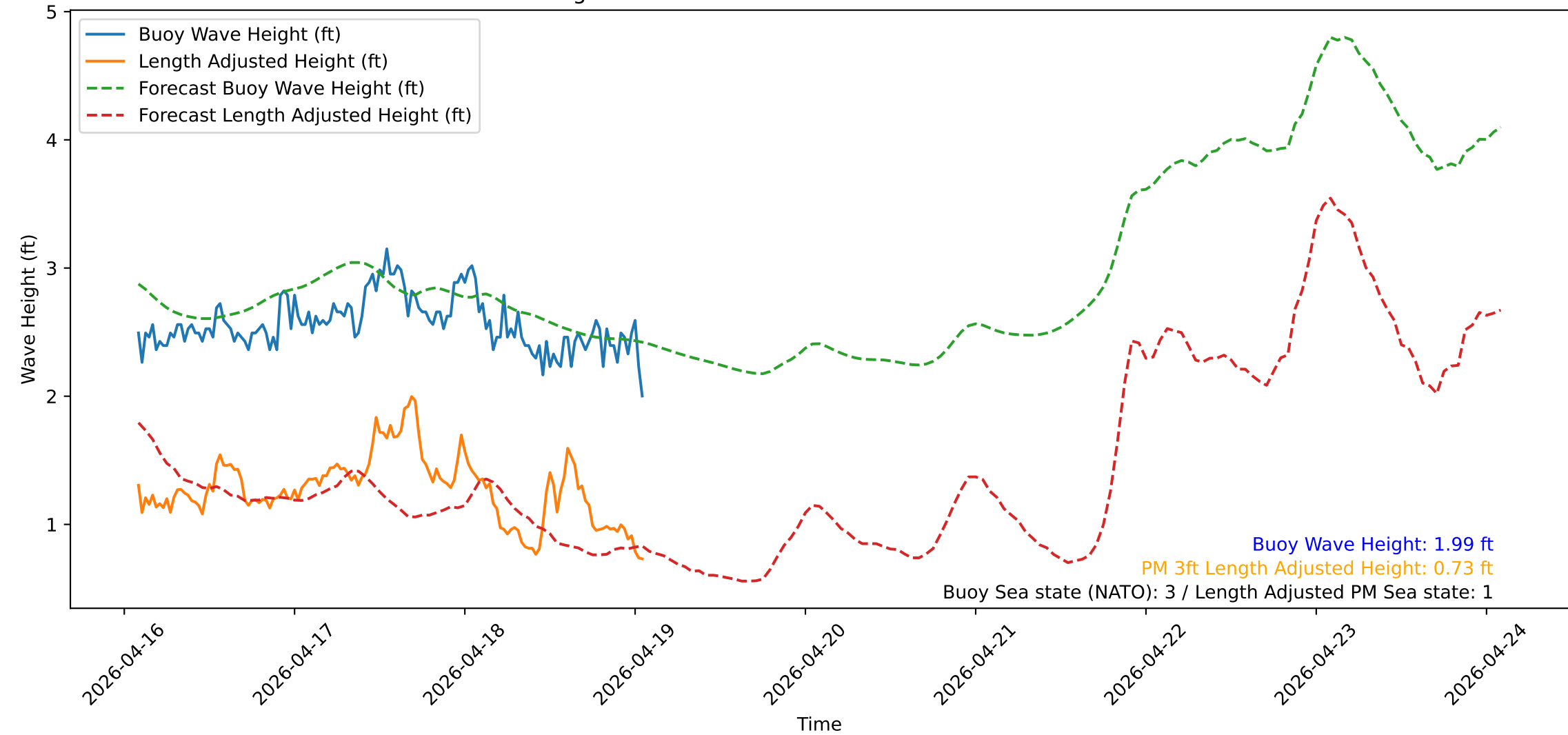
Wave Heights over Time for Red Beach at 2026-04-19 01:50:51
