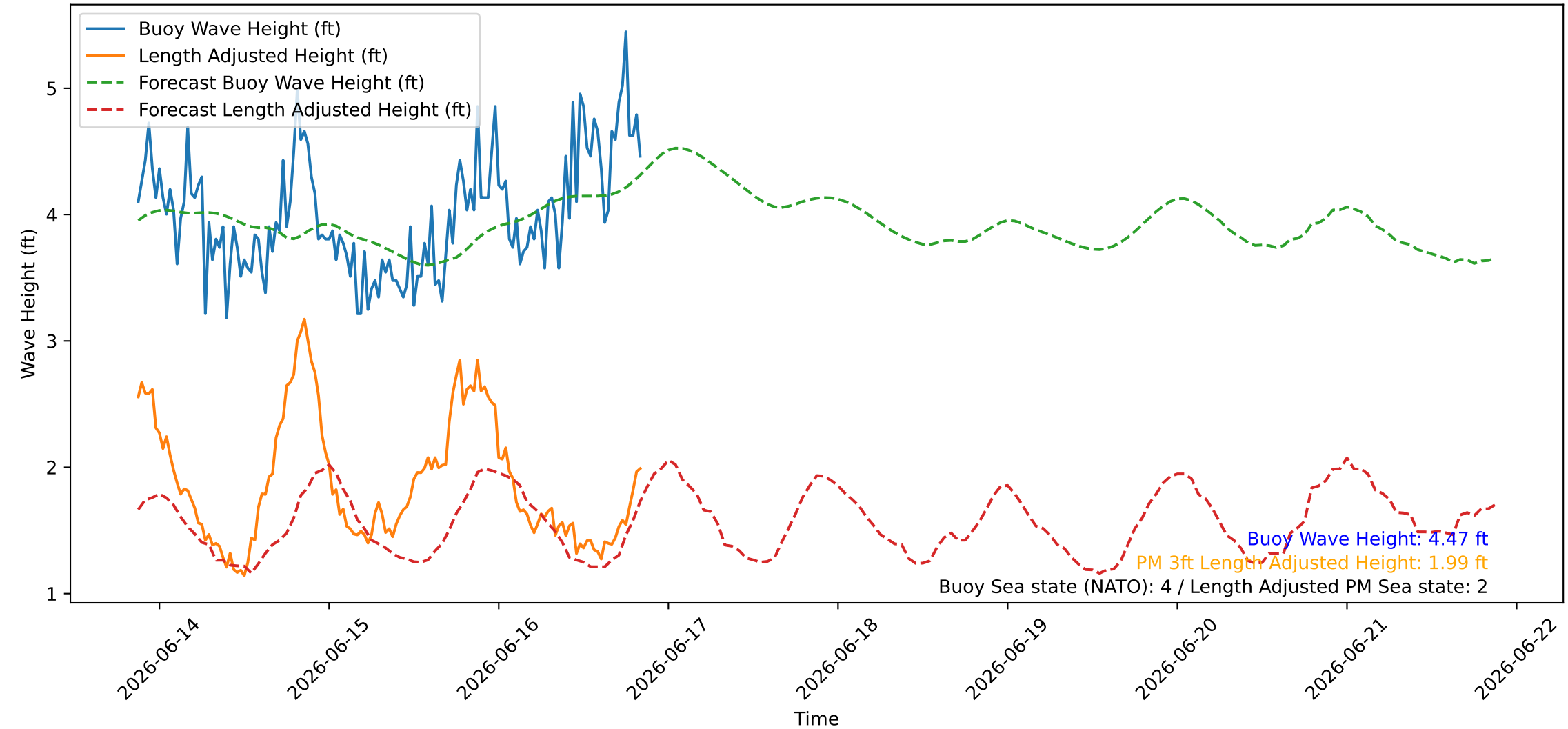
Wave Heights over Time for Oceanside Harbor at 2026-06-16 20:50:27
