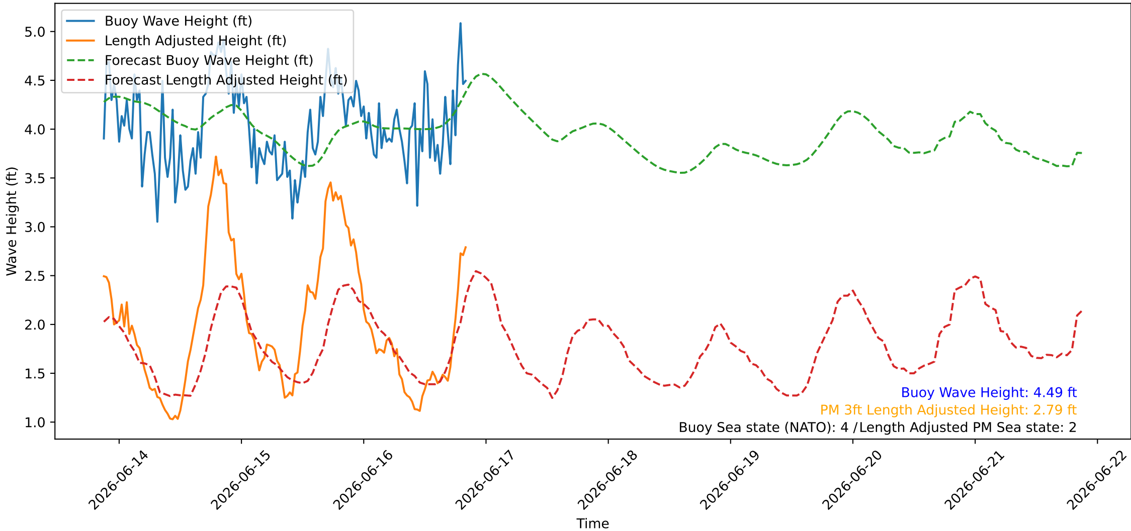
Wave Heights over Time for Green Beach at 2026-06-16 20:51:15
