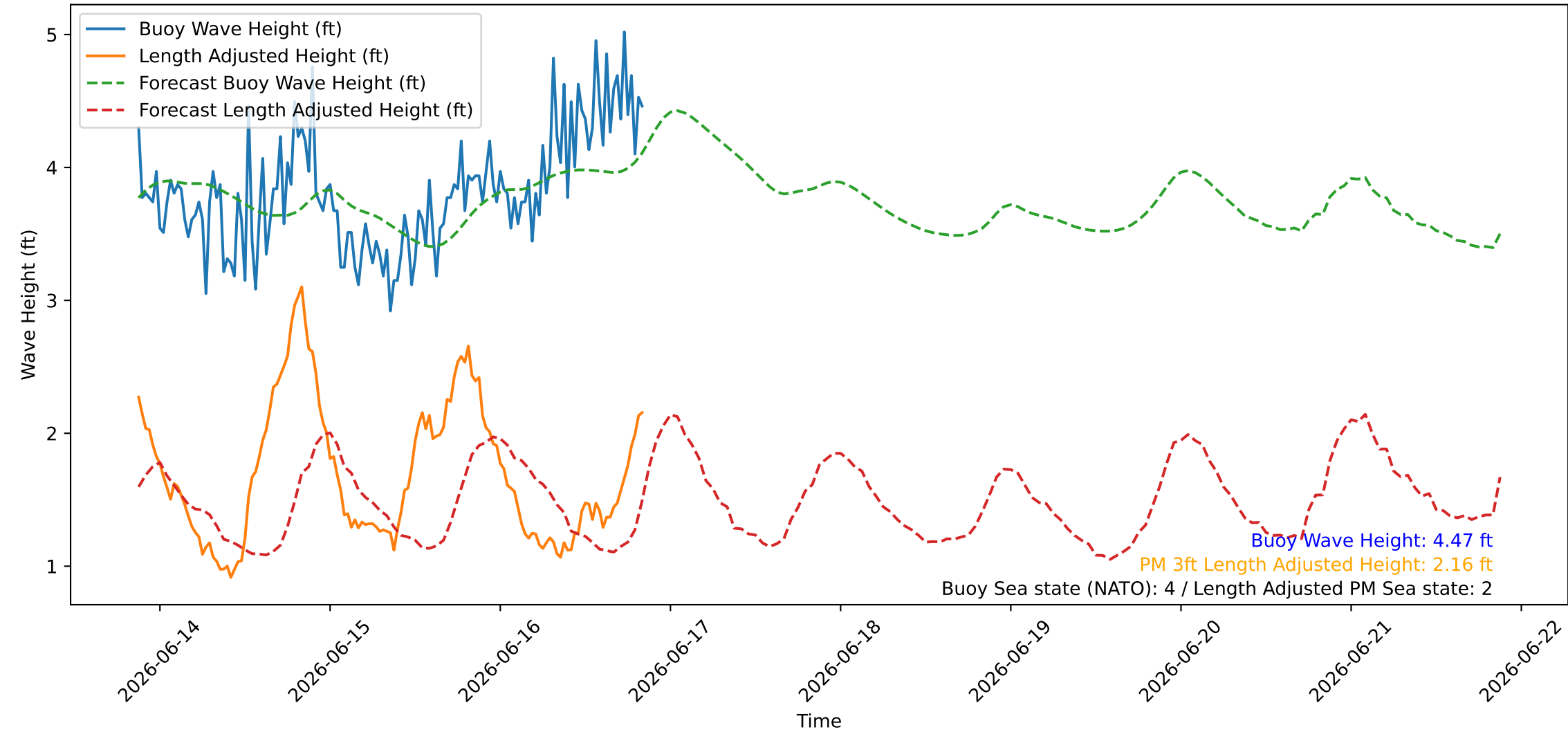
Wave Heights over Time for Red Beach at 2026-06-16 20:50:50
