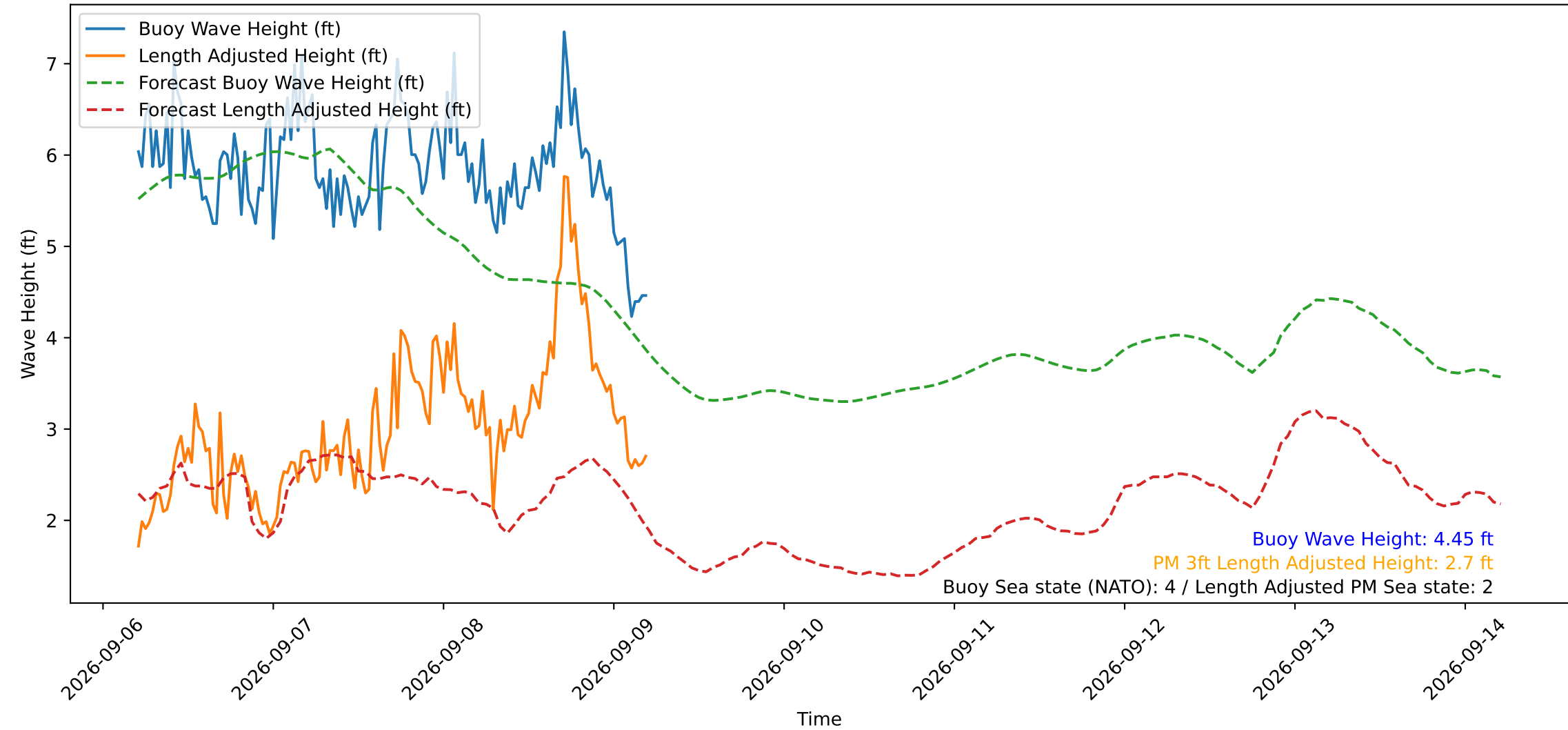
Wave Heights over Time for Oceanside Harbor at 2026-09-09 05:10:30
