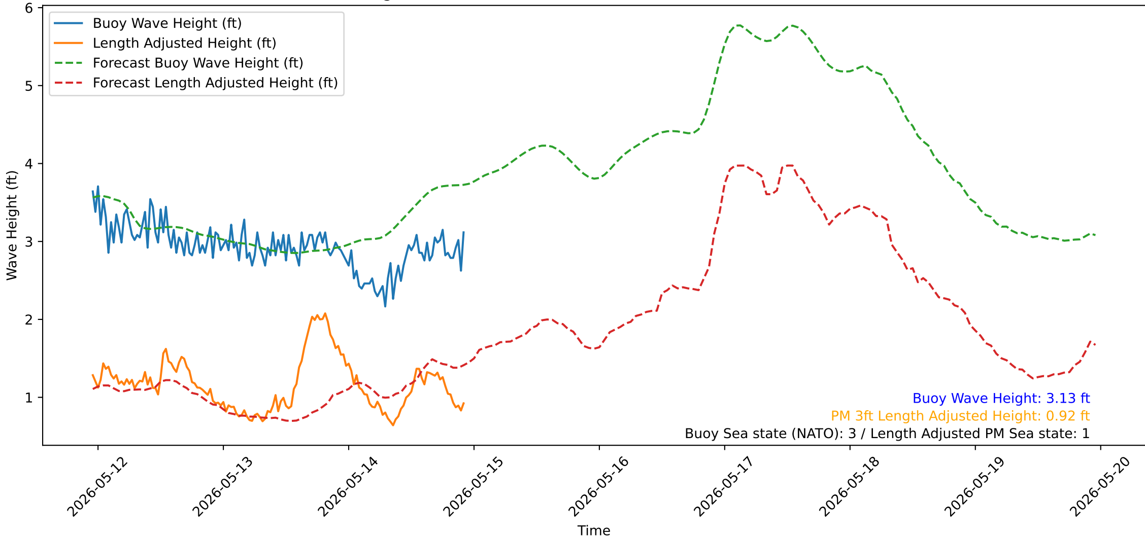
Wave Heights over Time for Oceanside Harbor at 2026-05-14 22:50:33
