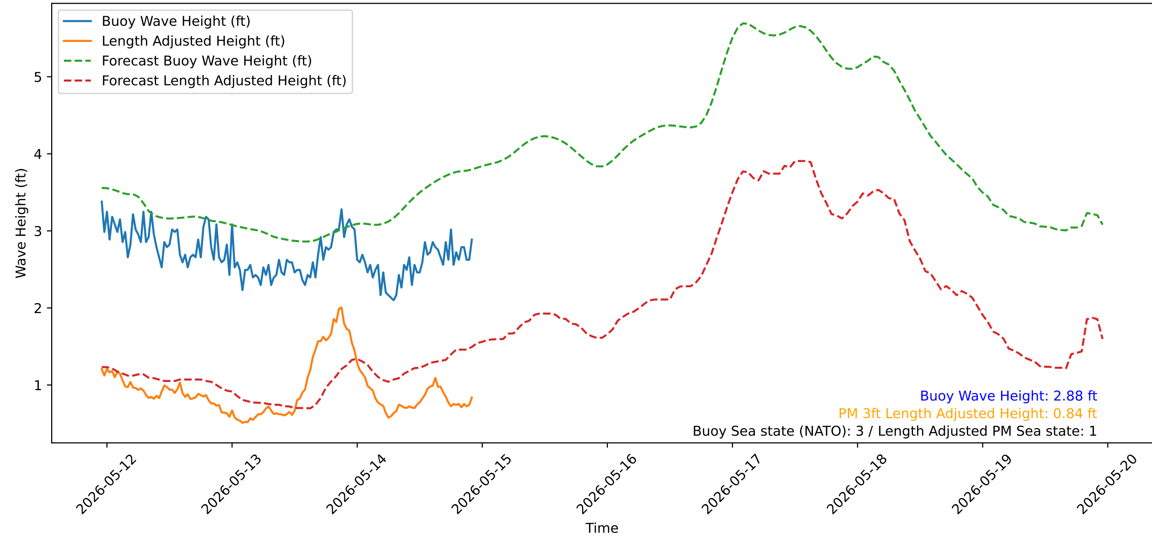
Wave Heights over Time for Green Beach at 2026-05-14 22:51:17
