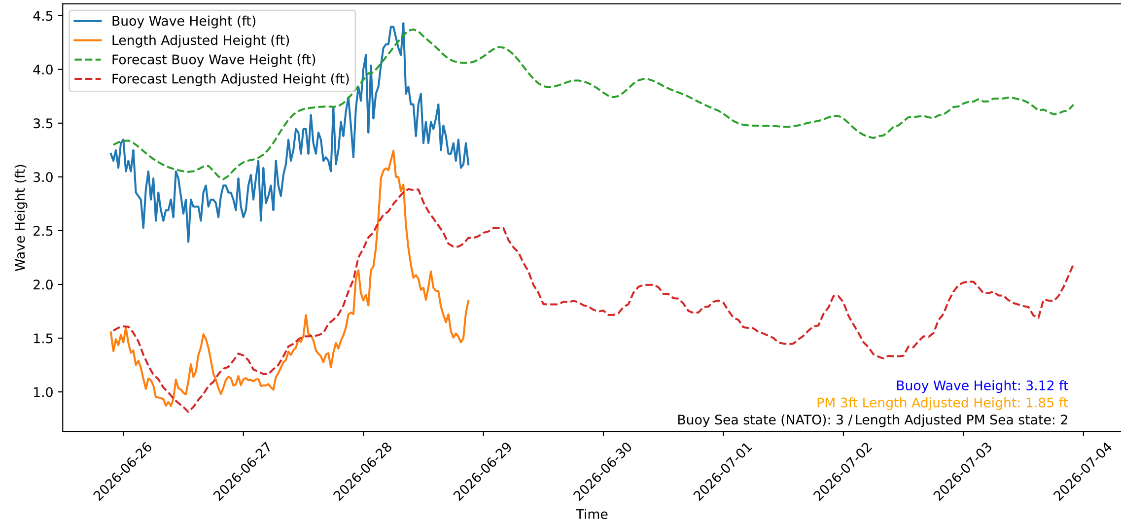
Wave Heights over Time for Oceanside Harbor at 2026-06-28 21:30:26
