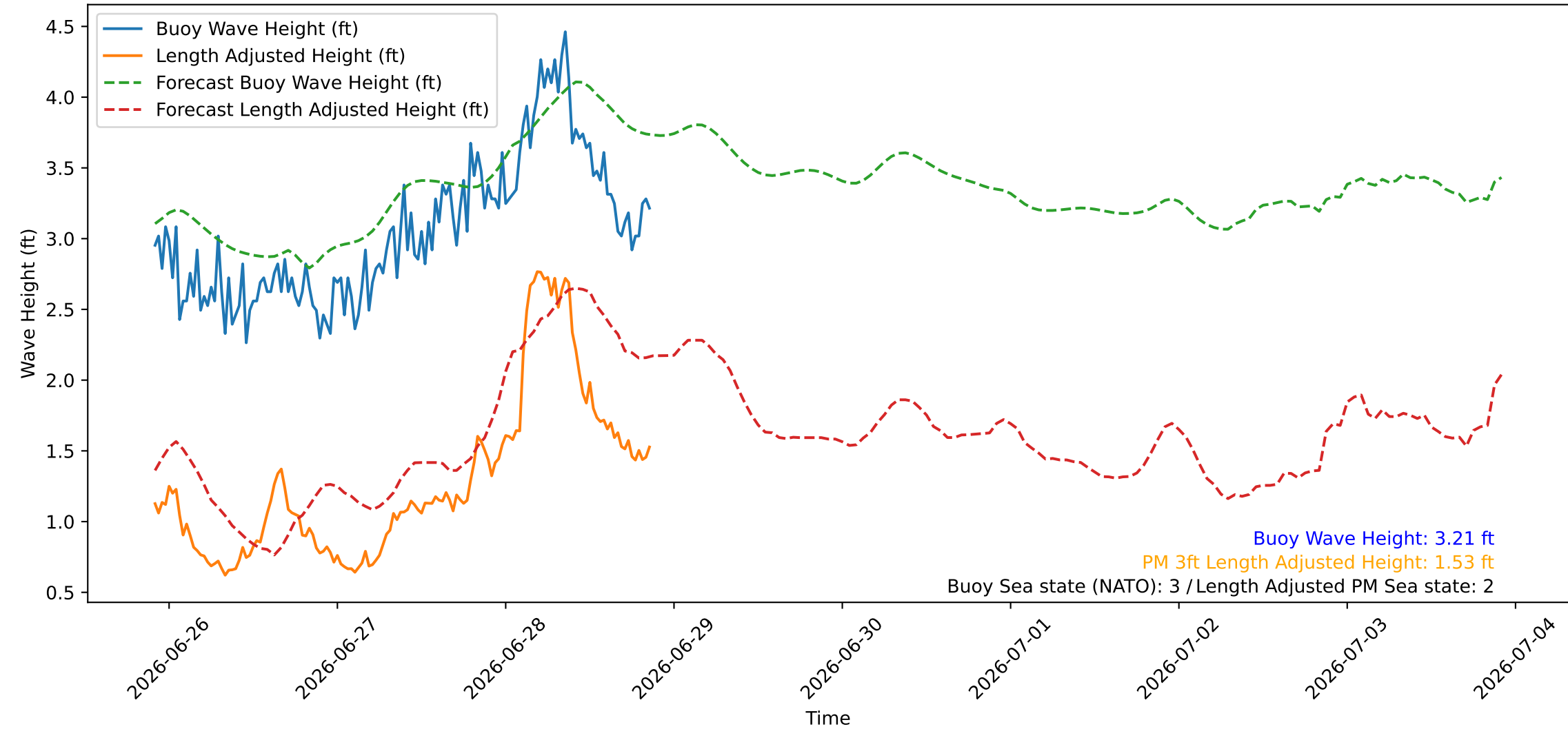
Wave Heights over Time for Red Beach at 2026-06-28 21:30:45
