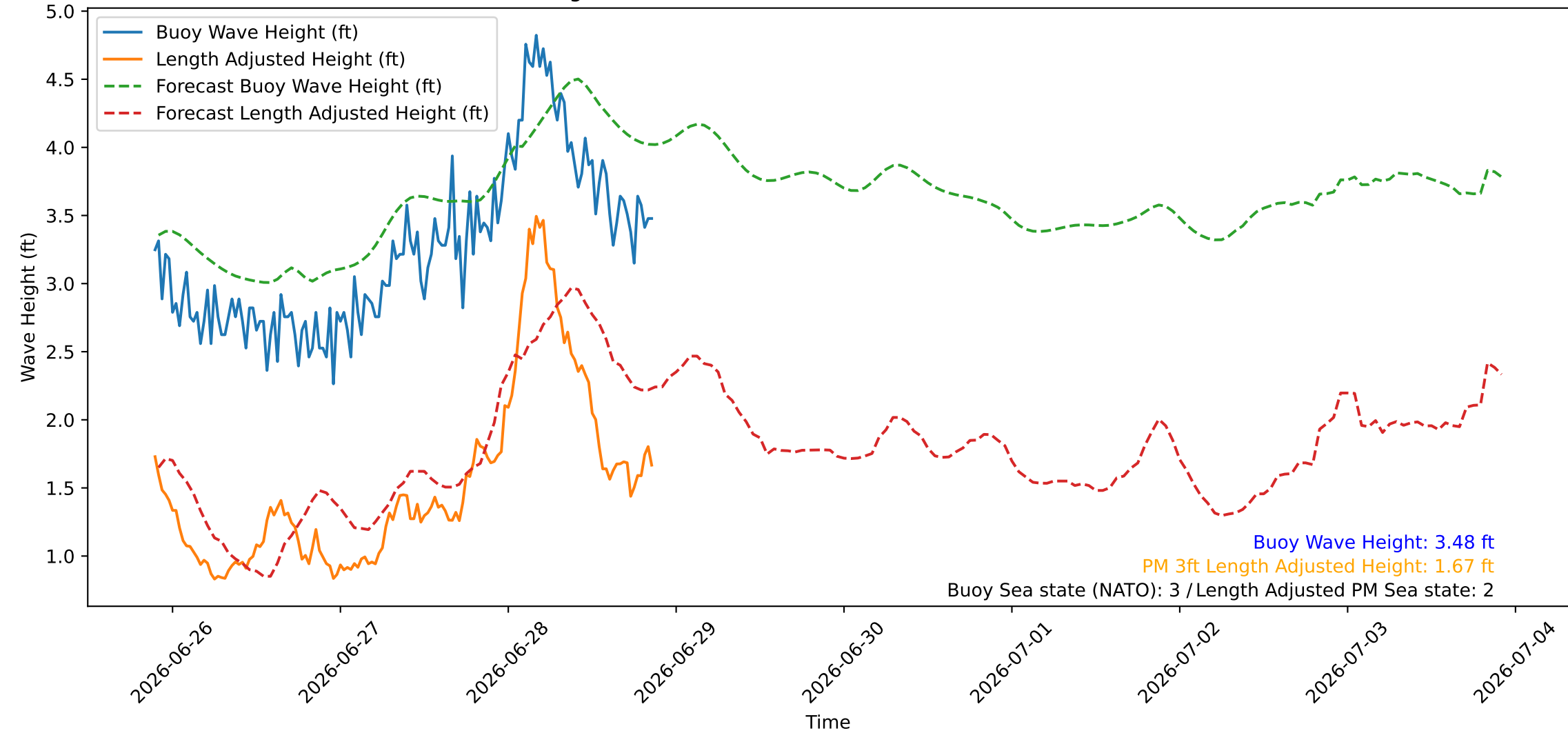
Wave Heights over Time for Green Beach at 2026-06-28 21:31:07
