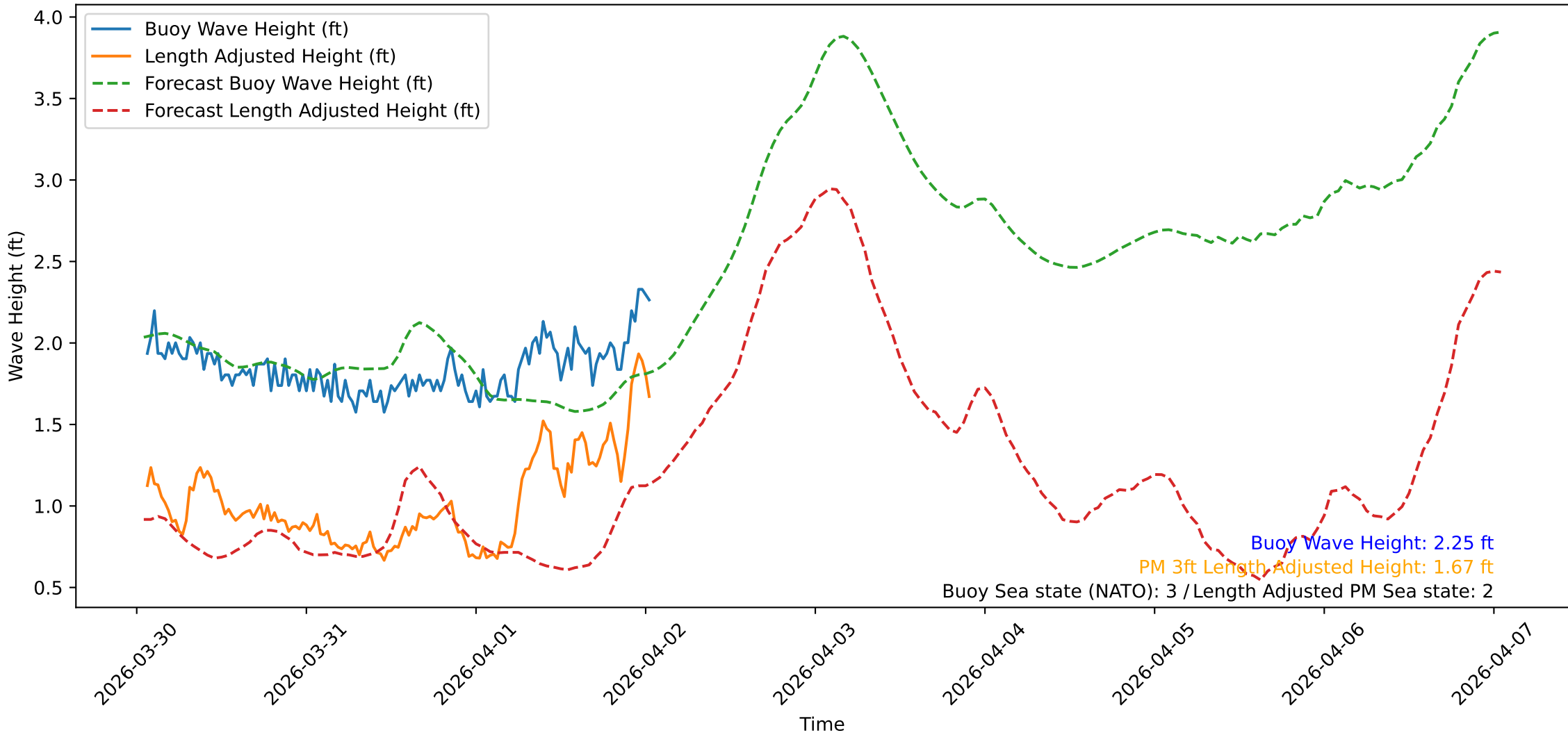
Wave Heights over Time for Oceanside Harbor at 2026-04-02 01:20:30
