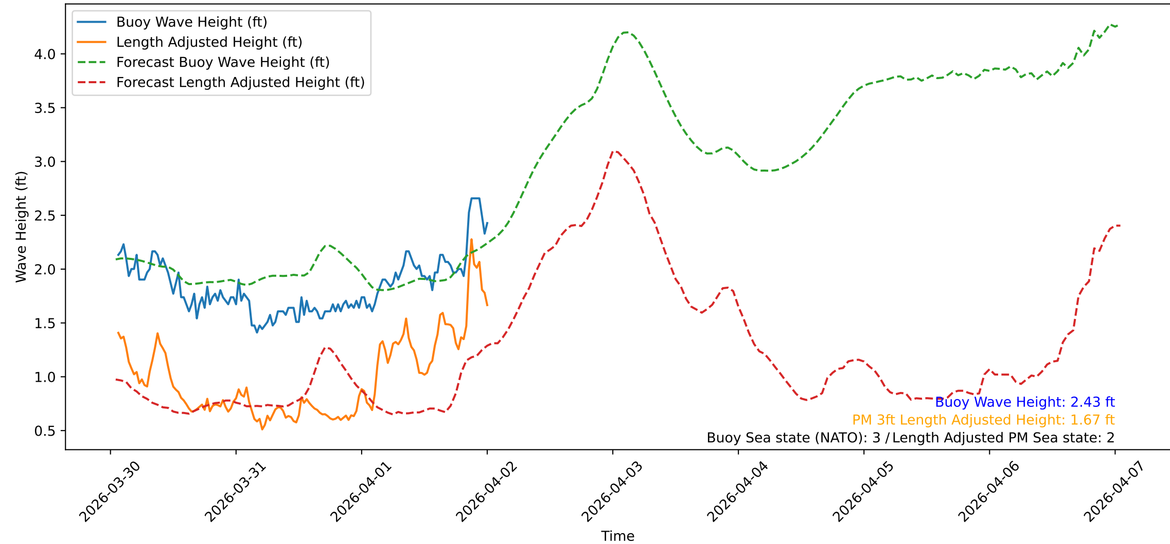
Wave Heights over Time for Green Beach at 2026-04-02 01:21:09
