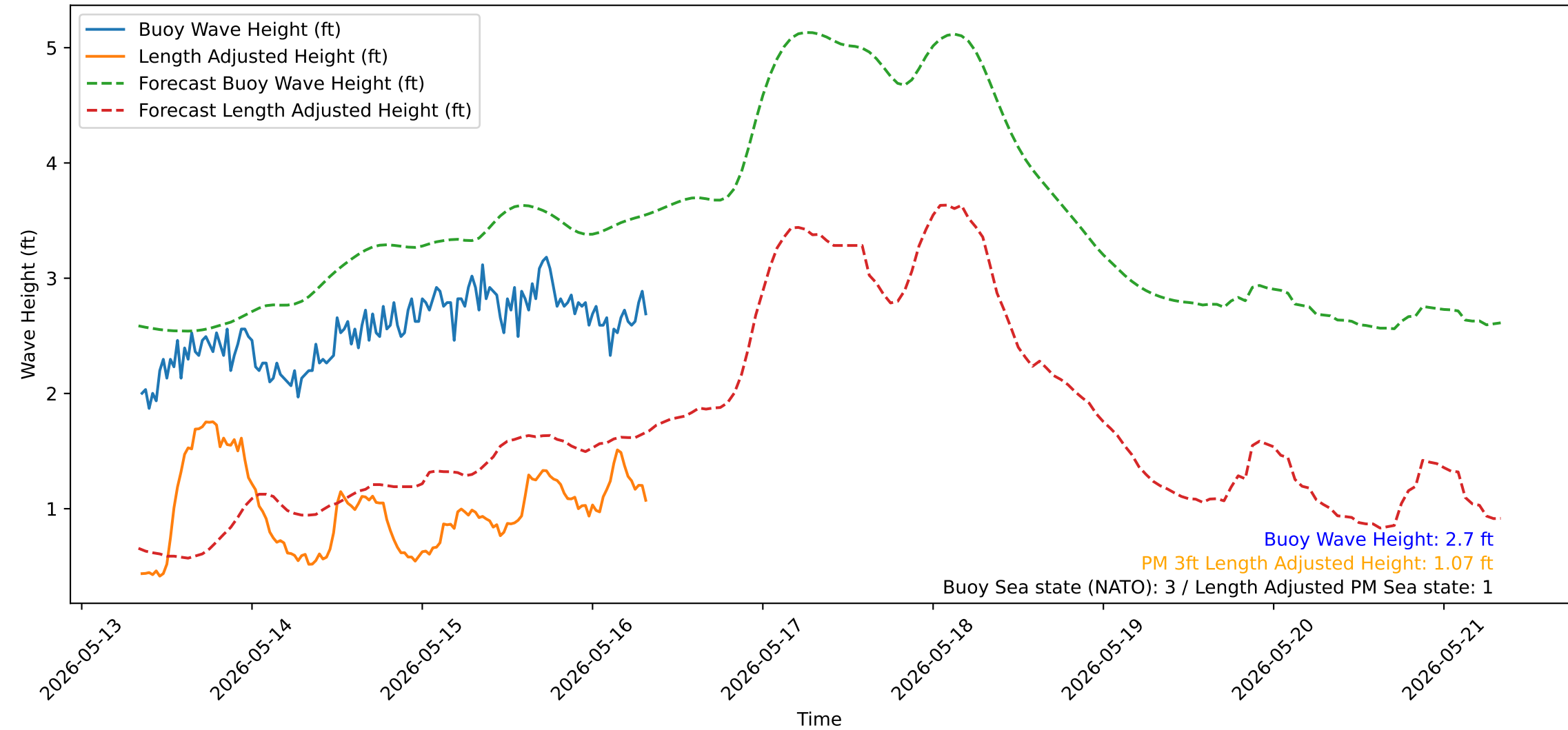
Wave Heights over Time for Red Beach at 2026-05-16 08:20:52
