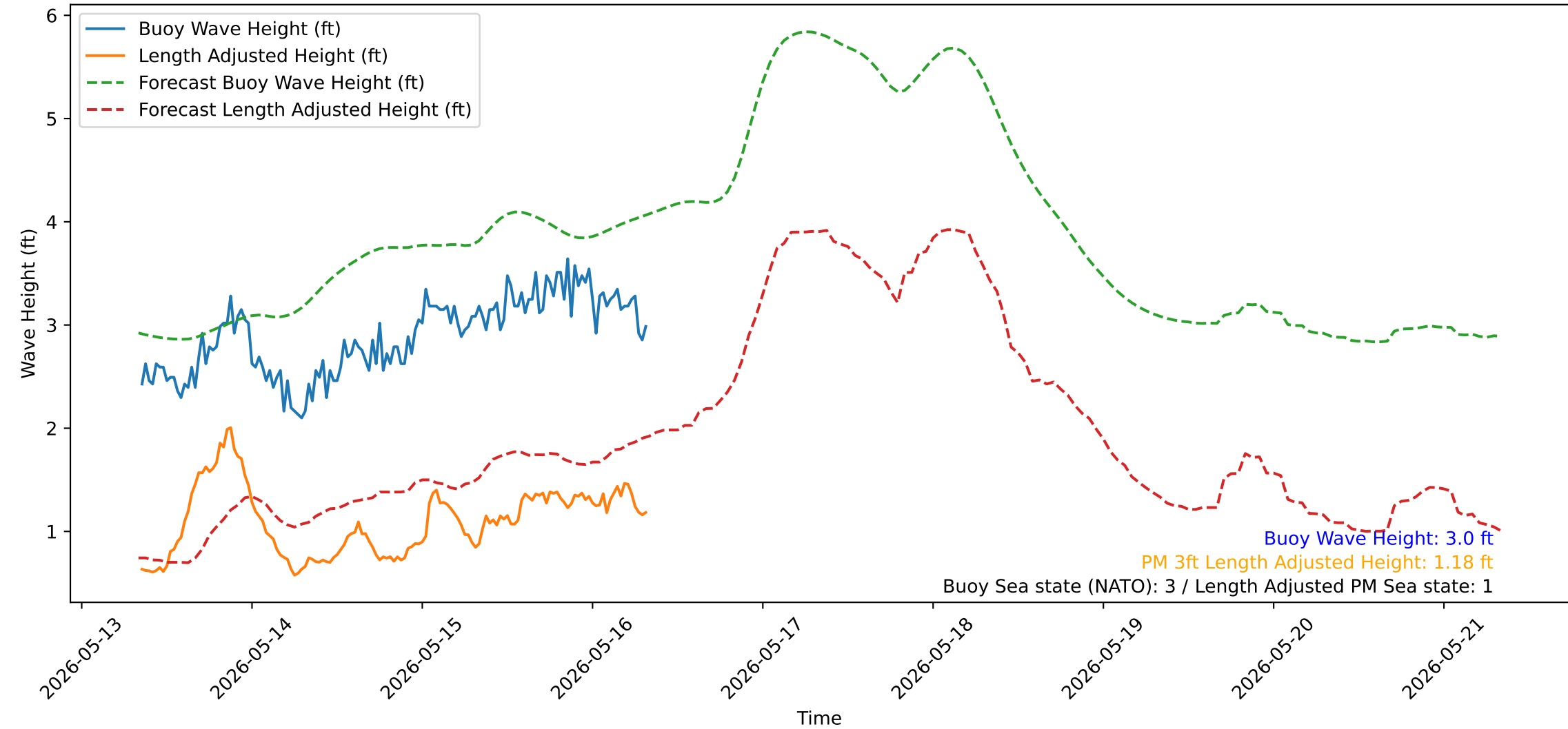
Wave Heights over Time for Green Beach at 2026-05-16 08:21:15
