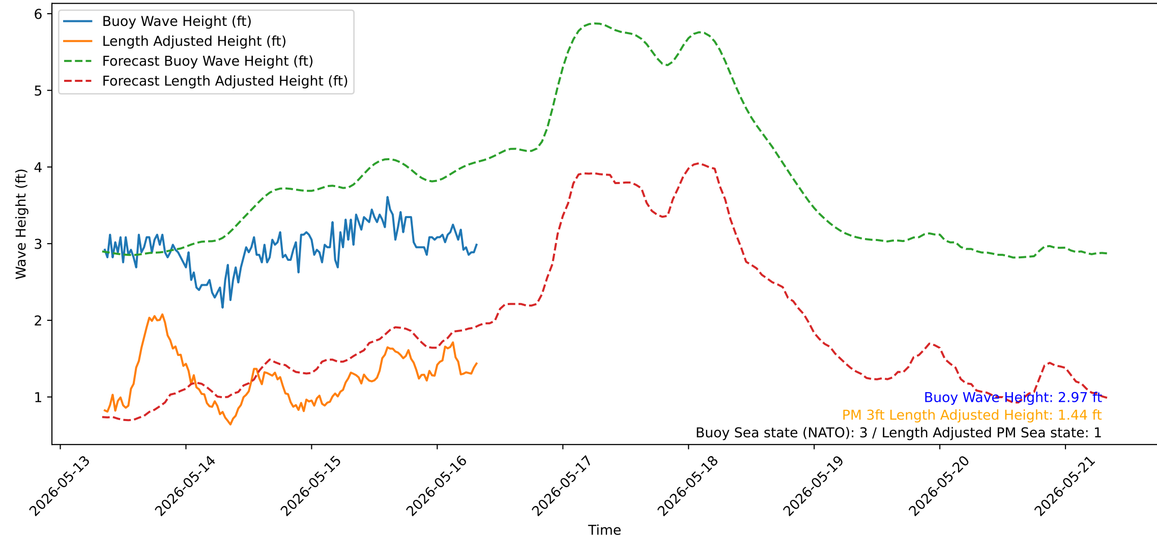
Wave Heights over Time for Oceanside Harbor at 2026-05-16 08:20:32
