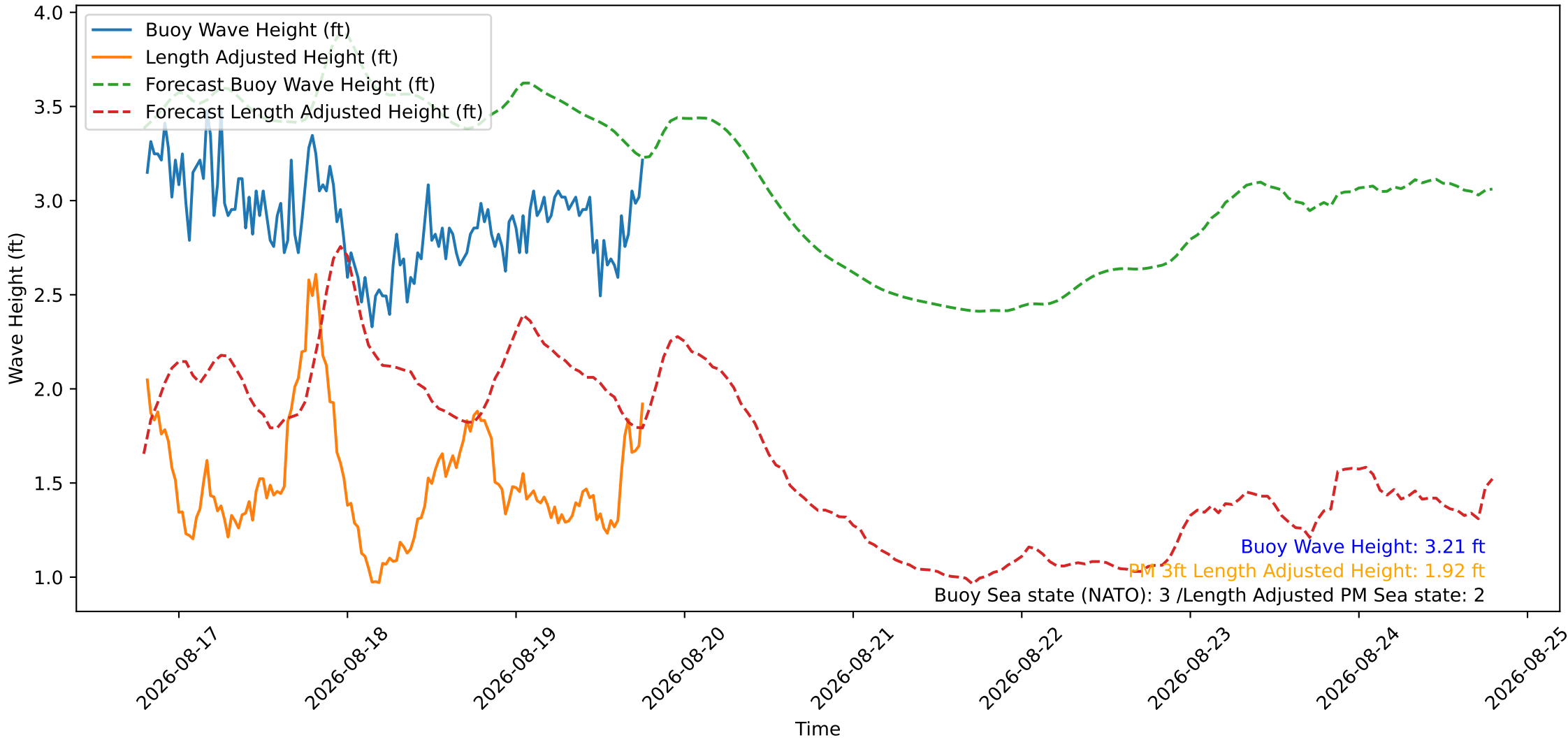
Wave Heights over Time for Red Beach at 2026-08-19 19:00:46
