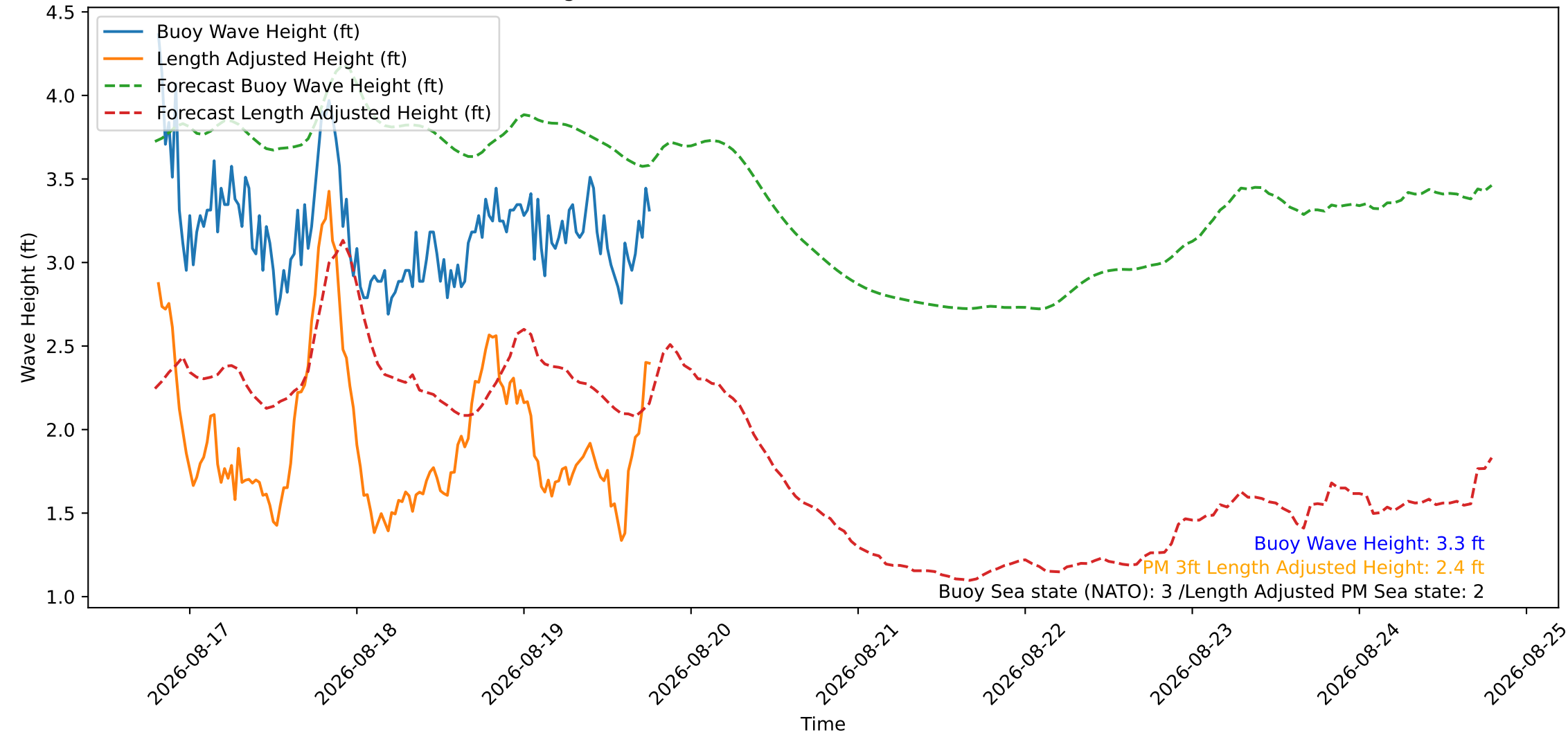
Wave Heights over Time for Green Beach at 2026-08-19 19:01:09
